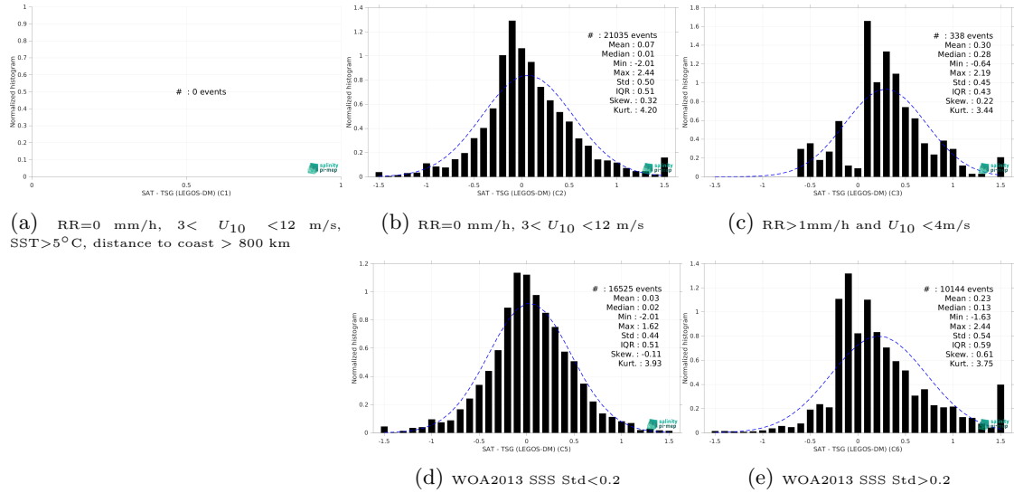
Figure 13: Normalized histogram of \Delta SSS (CCI SSS L4 Merged-OI v4.4 - 7-day running (ESA) - TSG (LEGOS-DM)) for 5 different subdatasets corresponding to: RR=0 mm/h, 3 < U_{10} < 12 m/s, SST >5^{\circ} C, distance to coast > 800 km (a), RR=0 mm/h, 3 < U_{10} < 12 m/s (b), RR >1 mm/h and U_{10} < 4 m/s (c), WOA2013 SSS Std <0.2 (d), WOA2013 SSS Std >0.2 (e).
