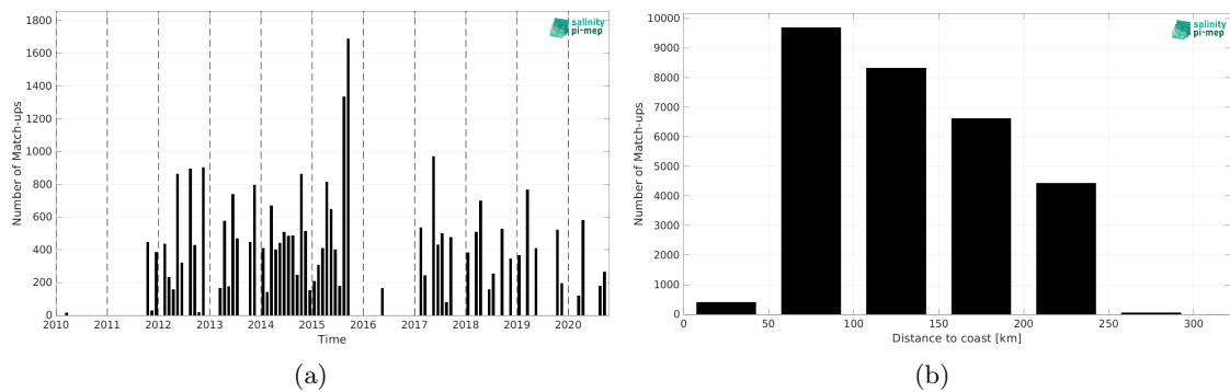
Figure 1: Number of match-ups between TSG (LEGOS-DM) and CCI SSS L4 Merged-OI v4.4 - 7-day running (ESA) SSS as a function of time (a) and as function of the distance to coast (b) over the Sea of Japan Pi-MEP region and for the full satellite product period.
