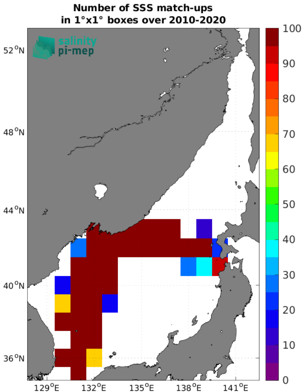
Figure 4: Number of SSS match-ups between TSG (LEGOS-DM) SSS and the CCI SSS L4 Merged-OI v4.4 - 7-day running (ESA) SSS product for the Sea of Japan Pi-MEP region over 1°x1° boxes and for the full satellite product period.
