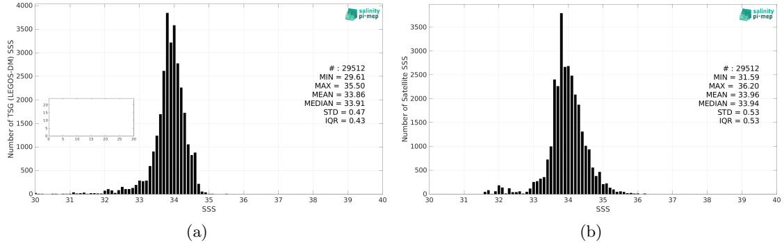
Figure 2: Histograms of SSS from TSG (LEGOS-DM) (a) and CCI SSS L4 Merged-OI v4.4 - 7-day running (ESA) (b) considering all match-up pairs per bins of 0.1 over the Sea of Japan Pi-MEP region and for the full satellite product period.
