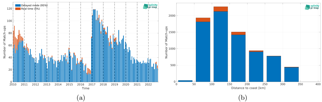
Figure 1: Number of match-ups between Argo and CCI SSS L4 Merged-OI v4.4 - 7-day running (ESA) SSS as a function of time (a) and as function of the distance to coast (b) over the Sea of Japan Pi-MEP region and for the full satellite product period.
