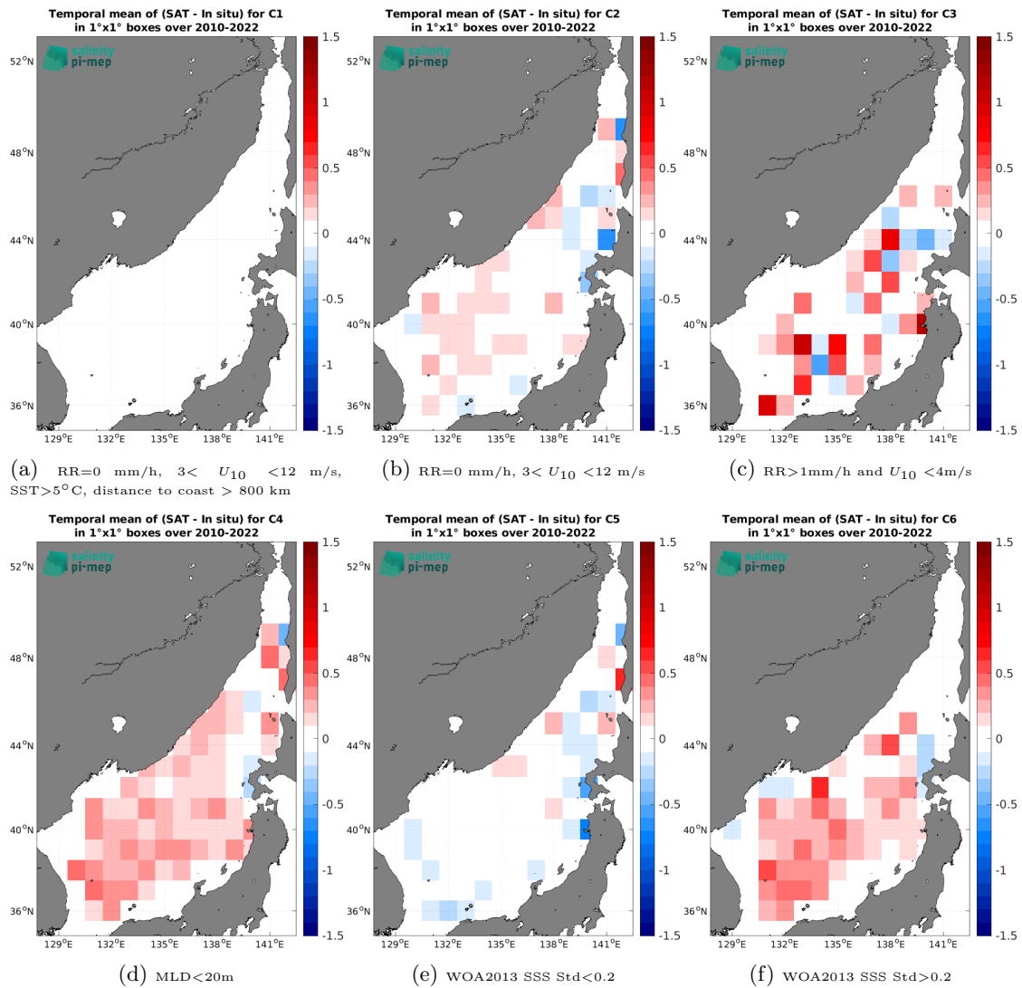
Figure 12: Temporal mean gridded over spatial boxes of size 1^\circ \times 1^\circ of \Delta SSS (CCI SSS L4 Merged-OI v4.4 - 7-day running (ESA) - Argo) for 6 different subdatasets corresponding to:RR=0 mm/h, 3 < U_{10} < 12 m/s, SST>5°C, distance to coast > 800 km (a), RR=0 mm/h, 3 < U_{10} < 12 m/s (b), RR>1mm/h and U_{10} < 4 m/s (c),MLD<20m (d),WOA2013 SSS Std<0.2 (e),WOA2013 SSS Std>0.2 (f).
