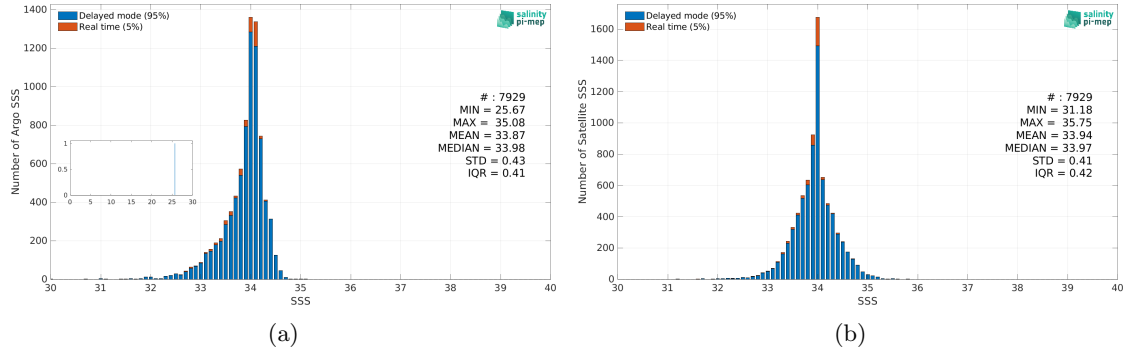
Figure 2: Histograms of SSS from Argo (a) and CCI SSS L4 Merged-OI v4.4 - 7-day running (ESA) (b) considering all match-up pairs per bins of 0.1 over the Sea of Japan Pi-MEP region and for the full satellite product period.
