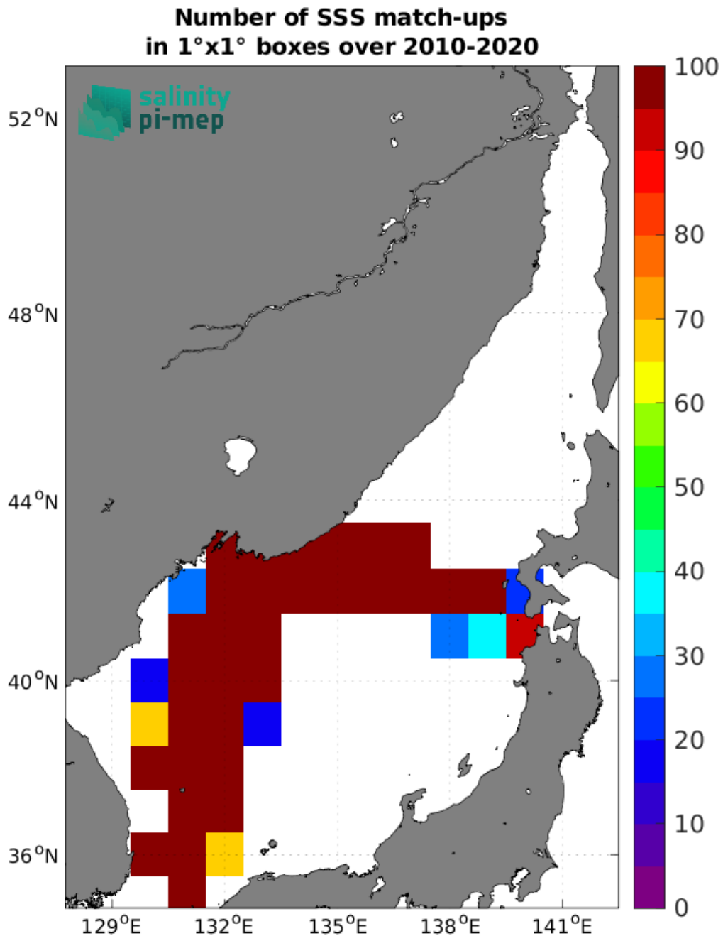
Figure 4: Number of SSS match-ups between TSG (LEGOS-DM) SSS and the CCI SSS L4 Merged-OI v4.4 - 30-day running (ESA) SSS product for the Sea of Japan Pi-MEP region over 1°x1° boxes and for the full satellite product period.
