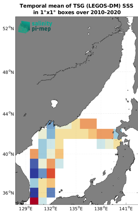
(c) MEAN(TSG (LEGOS-DM) SSS)
