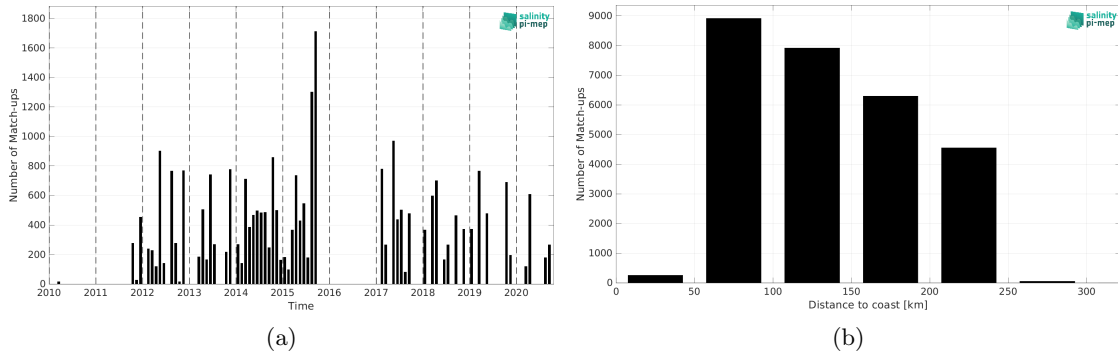
Figure 1: Number of match-ups between TSG (LEGOS-DM) and CCI SSS L4 Merged-OI v4.4 - 30-day running (ESA) SSS as a function of time (a) and as function of the distance to coast (b) over the Sea of Japan Pi-MEP region and for the full satellite product period.
