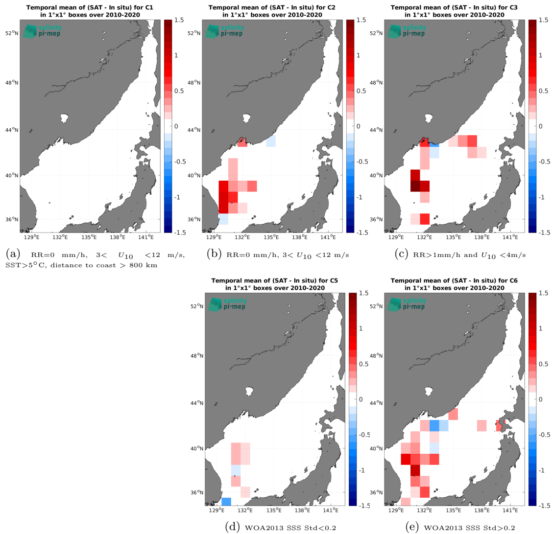
Figure 12: Temporal mean gridded over spatial boxes of size 1^\circ \times 1^\circ of \Delta SSS (CCI SSS L4 Merged-OI v4.4 - 30-day running (ESA) - TSG (LEGOS-DM)) for 5 different subdatasets corresponding to: RR=0 mm/h, 3 < U_{10} < 12 m/s, SST>5°C, distance to coast > 800 km (a), RR=0 mm/h, 3 < U_{10} < 12 m/s (b), RR>1mm/h and U_{10} < 4 m/s (c), WOA2013 SSS Std<0.2 (d), WOA2013 SSS Std>0.2 (e).
