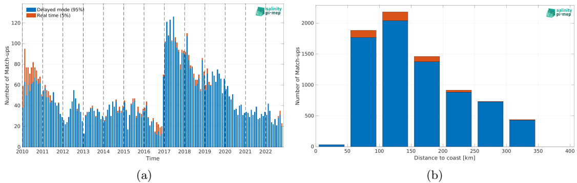
Figure 1: Number of match-ups between Argo and CCI SSS L4 Merged-OI v4.4 - 30-day running (ESA) SSS as a function of time (a) and as function of the distance to coast (b) over the Sea of Japan Pi-MEP region and for the full satellite product period.
