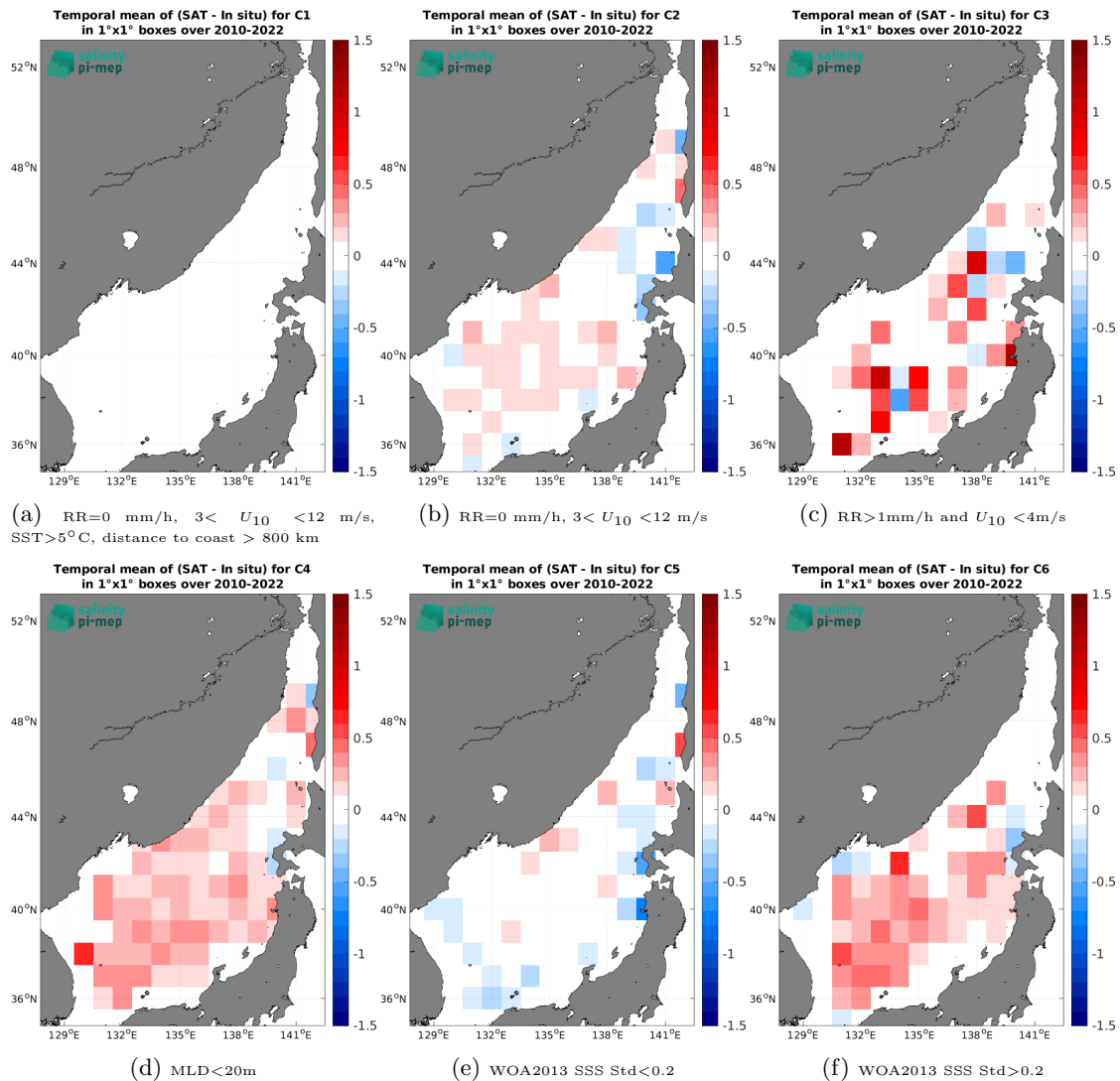
Figure 12: Temporal mean gridded over spatial boxes of size 1^\circ \times 1^\circ of \Delta SSS (CCI SSS L4 Merged-OI v4.4 - 30-day running (ESA) - Argo) for 6 different subdatasets corresponding to:RR=0 mm/h, 3 < U_{10} < 12 m/s, SST>5°C, distance to coast > 800 km (a), RR=0 mm/h, 3 < U_{10} < 12 m/s (b), RR>1mm/h and U_{10} < 4 m/s (c),MLD<20m (d),WOA2013 SSS Std<0.2 (e),WOA2013 SSS Std>0.2 (f).
