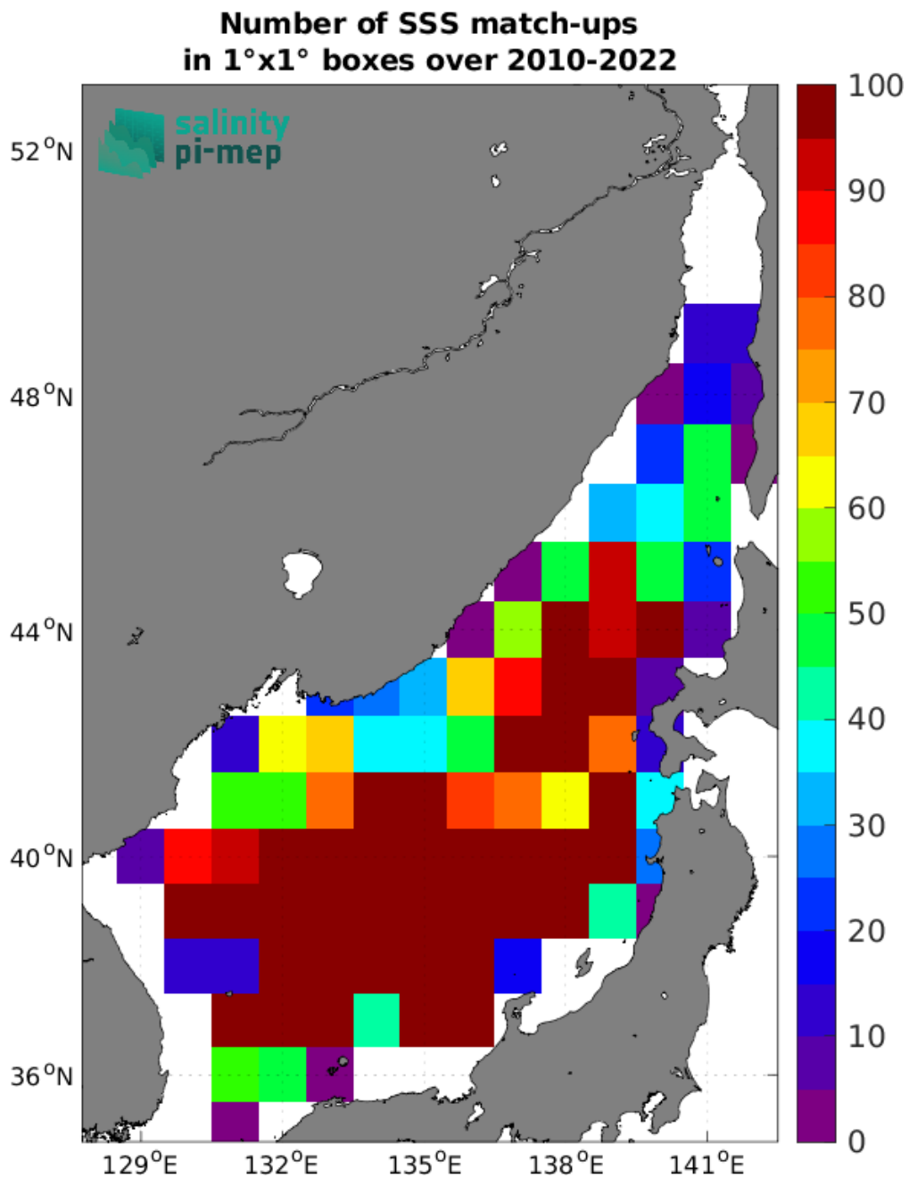
Figure 4: Number of SSS match-ups between Argo SSS and the CCI SSS L4 Merged-OI v4.4 - 30-day running (ESA) SSS product for the Sea of Japan Pi-MEP region over 1°x1° boxes and for the full satellite product period.
