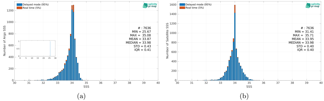
Figure 2: Histograms of SSS from Argo (a) and CCI SSS L4 Merged-OI v4.4 - 30-day running (ESA) (b) considering all match-up pairs per bins of 0.1 over the Sea of Japan Pi-MEP region and for the full satellite product period.
