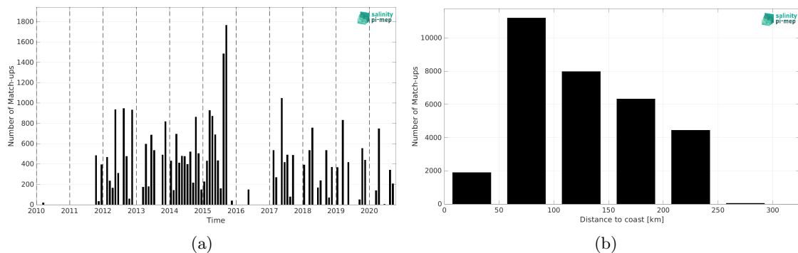
Figure 1: Number of match-ups between TSG (LEGOS-DM) and CCI SSS L4 Merged-OI v3.2 - 7-day running (ESA) SSS as a function of time (a) and as function of the distance to coast (b) over the Sea of Japan Pi-MEP region and for the full satellite product period.
