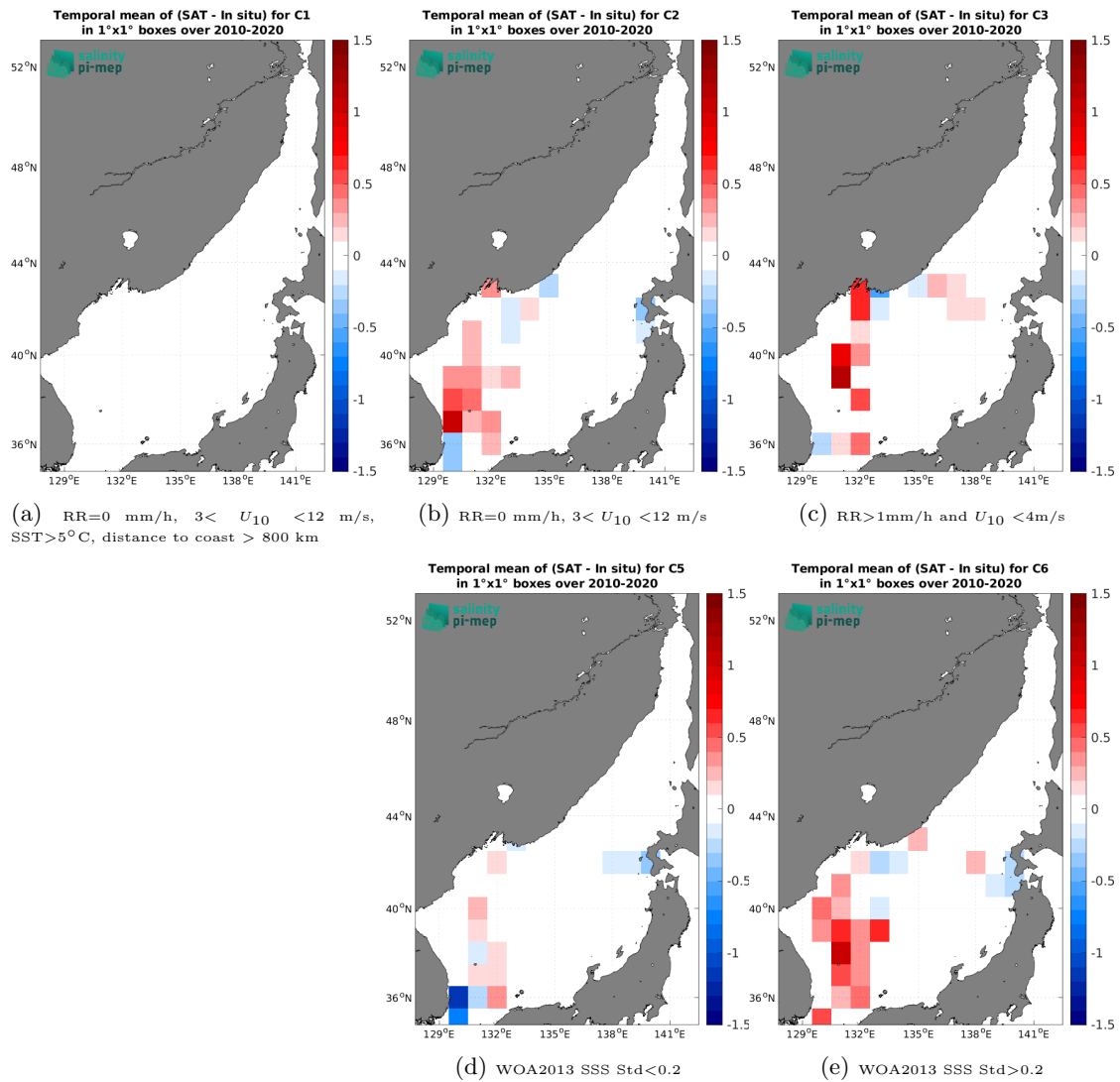
Figure 12: Temporal mean gridded over spatial boxes of size 1^\circ \times 1^\circ of \Delta\text{SSS} (CCI SSS L4 Merged-OI v3.2 - 7-day running (ESA) - TSG (LEGOS-DM)) for 5 different subdatasets corresponding to: RR=0 mm/h, 3 < U_{10} < 12 m/s, SST > 5^\circ\text{C} , distance to coast > 800 km (a), RR=0 mm/h, 3 < U_{10} < 12 m/s (b), RR > 1 mm/h and U_{10} < 4 m/s (c), WOA2013 SSS Std < 0.2 (d), WOA2013 SSS Std > 0.2 (e).
