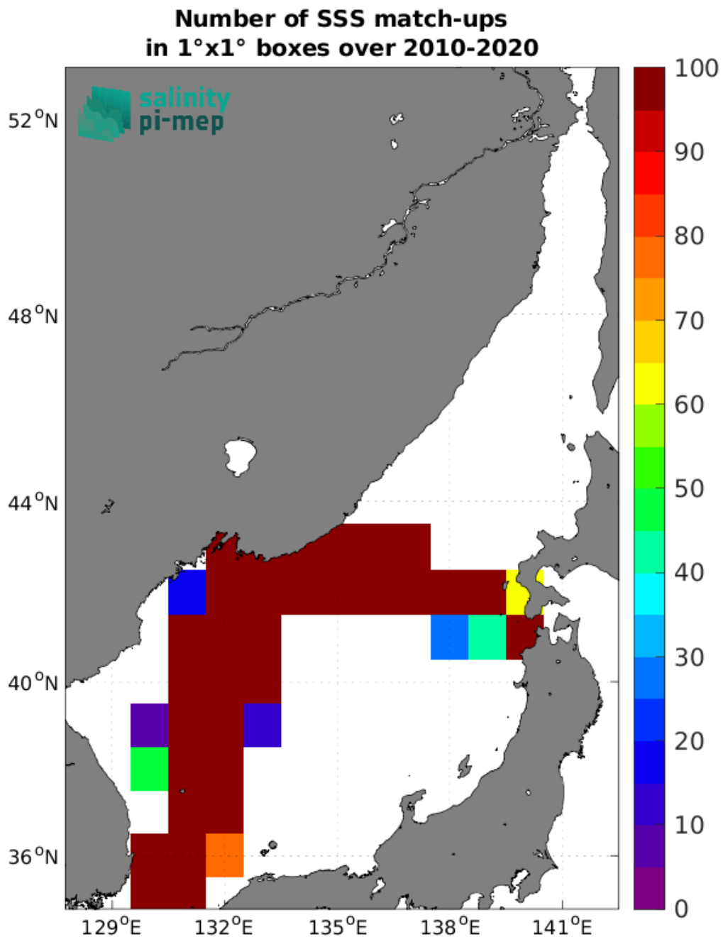
Figure 4: Number of SSS match-ups between TSG (LEGOS-DM) SSS and the CCI SSS L4 Merged-OI v3.2 - 7-day running (ESA) SSS product for the Sea of Japan Pi-MEP region over 1°x1° boxes and for the full satellite product period.
