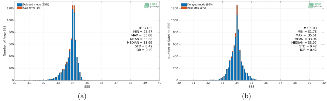
Figure 2: Histograms of SSS from Argo (a) and CCI SSS L4 Merged-OI v3.2 - 7-day running (ESA) (b) considering all match-up pairs per bins of 0.1 over the Sea of Japan Pi-MEP region and for the full satellite product period.
