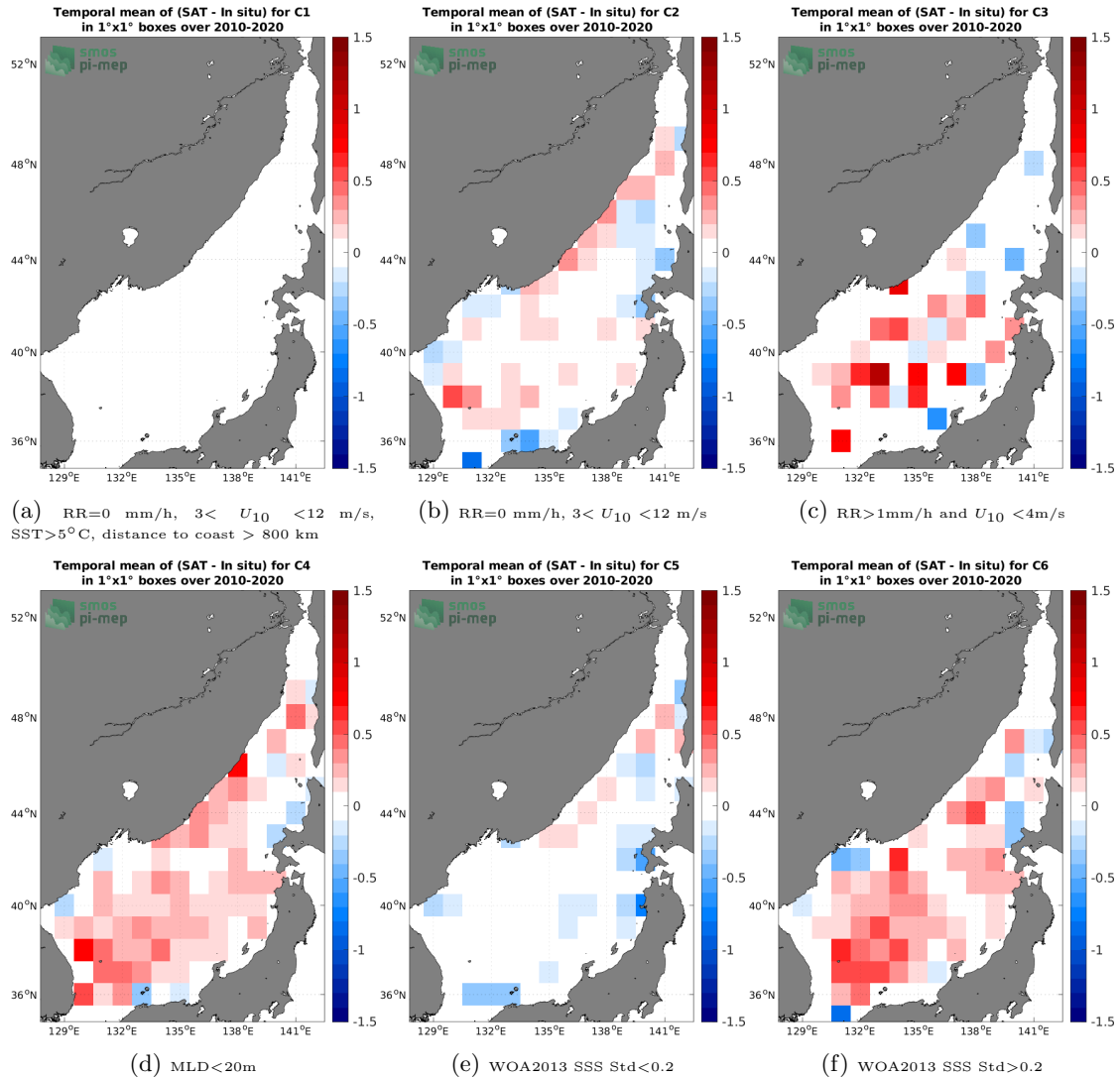
Figure 12: Temporal mean gridded over spatial boxes of size 1^\circ \times 1^\circ of \Delta\text{SSS} (CCI SSS L4 Merged-OI v3.2 - 7-day running (ESA) - Argo) for 6 different subdatasets corresponding to: RR=0 mm/h, 3 < U_{10} < 12 m/s, SST > 5^\circ\text{C} , distance to coast > 800 km (a), RR=0 mm/h, 3 < U_{10} < 12 m/s (b), RR > 1 mm/h and U_{10} < 4 m/s (c), MLD < 20 m (d), WOA2013 SSS Std < 0.2 (e), WOA2013 SSS Std > 0.2 (f).
