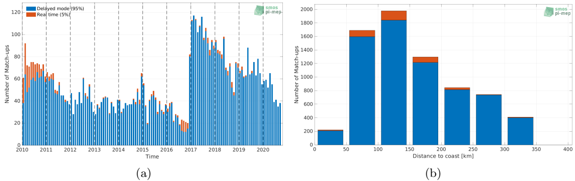
Figure 1: Number of match-ups between Argo and CCI SSS L4 Merged-OI v3.2 - 7-day running (ESA) SSS as a function of time (a) and as function of the distance to coast (b) over the Sea of Japan Pi-MEP region and for the full satellite product period.
