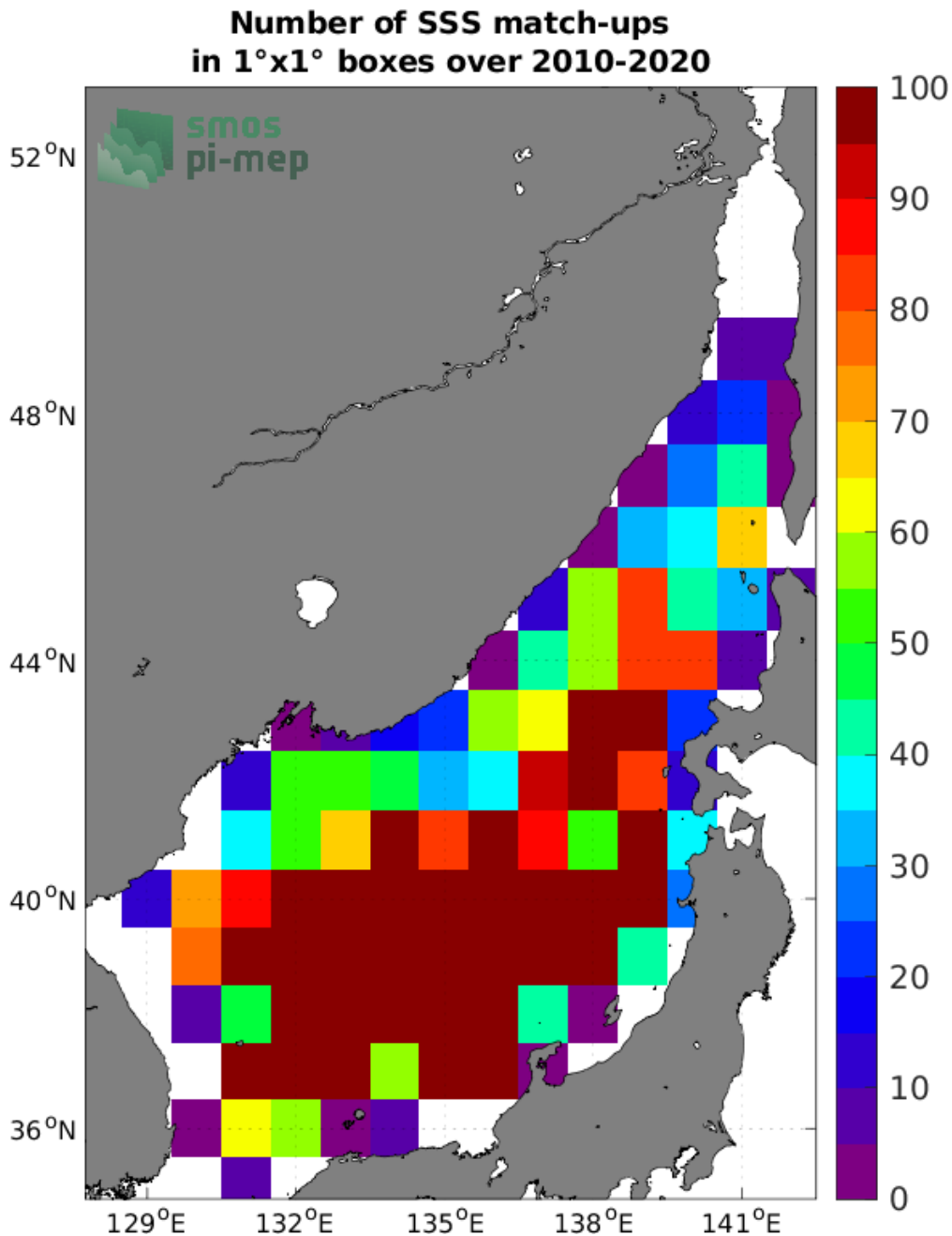
Figure 4: Number of SSS match-ups between Argo SSS and the CCI SSS L4 Merged-OI v3.2 - 7-day running (ESA) SSS product for the Sea of Japan Pi-MEP region over 1°x1° boxes and for the full satellite product period.
