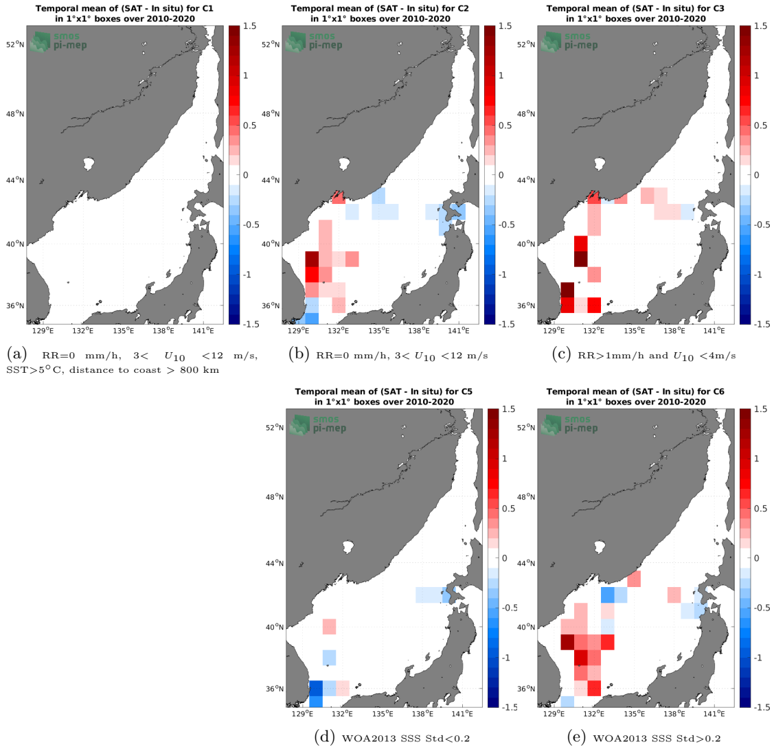
Figure 12: Temporal mean gridded over spatial boxes of size 1^\circ \times 1^\circ of \Delta SSS (CCI SSS L4 Merged-OI v3.2 - 30-day running (ESA) - TSG (LEGOS-DM)) for 5 different subdatasets corresponding to:RR=0 mm/h, 3 < U_{10} < 12 m/s, SST>5°C, distance to coast > 800 km (a), RR=0 mm/h, 3 < U_{10} < 12 m/s (b), RR>1mm/h and U_{10} < 4 m/s (c), WOA2013 SSS Std<0.2 (d), WOA2013 SSS Std>0.2 (e).
