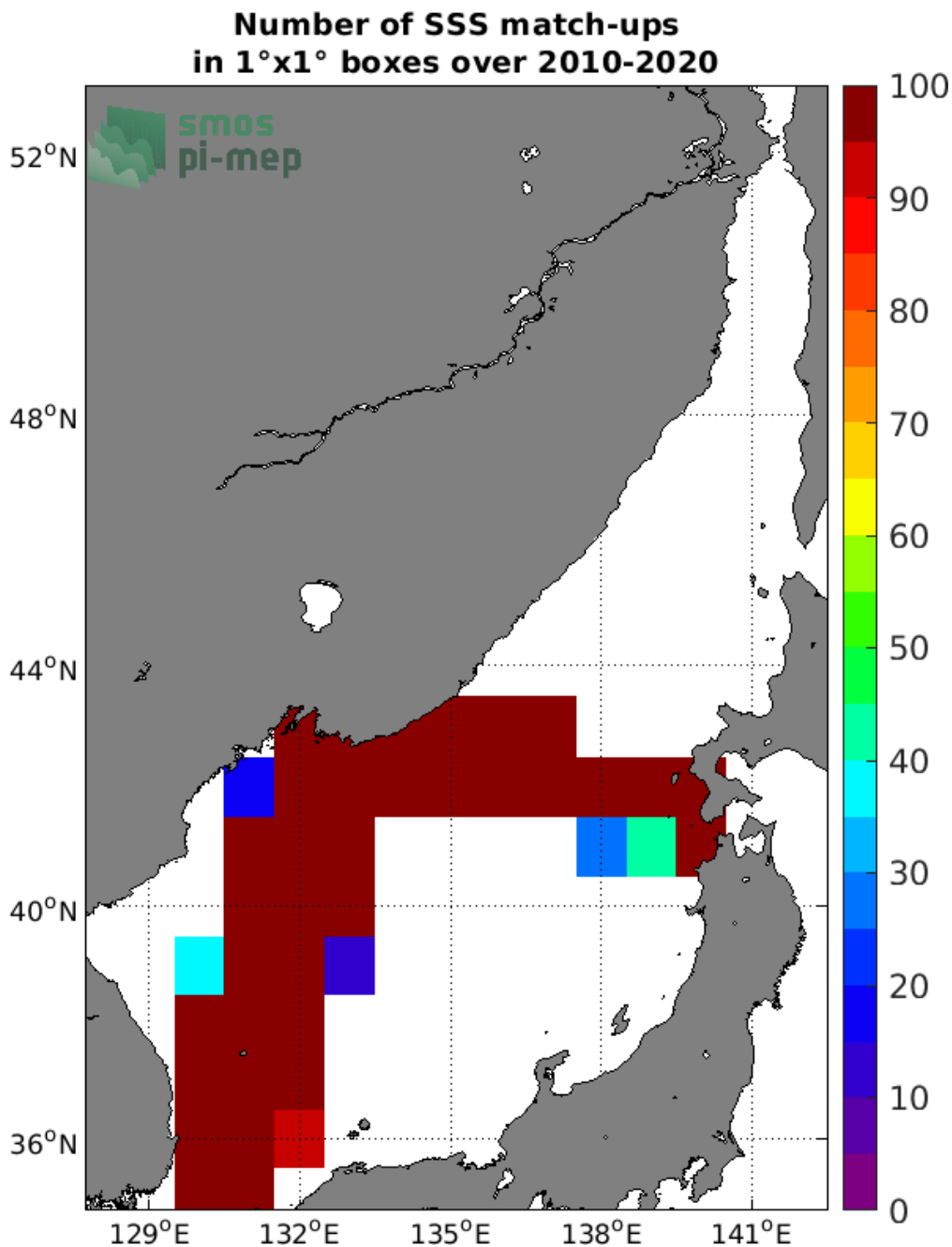
Figure 4: Number of SSS match-ups between TSG (LEGOS-DM) SSS and the CCI SSS L4 Merged-OI v3.2 - 30-day running (ESA) SSS product for the Sea of Japan Pi-MEP region over 1°x1° boxes and for the full satellite product period.
