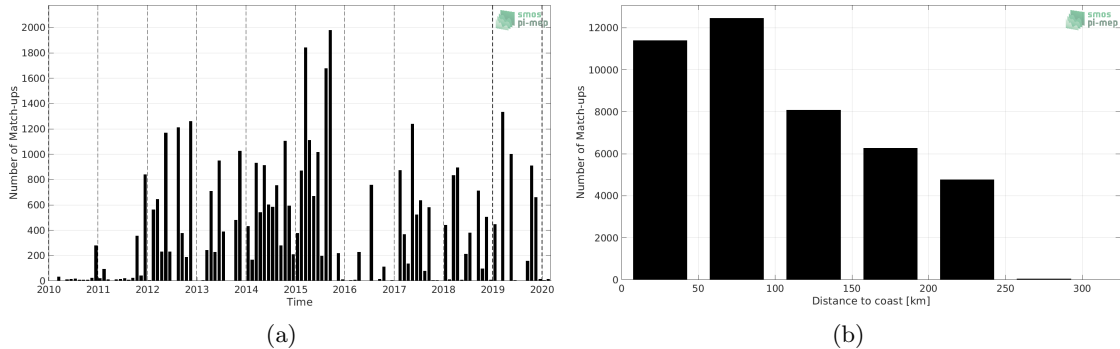
Figure 1: Number of match-ups between TSG (LEGOS-DM) and CCI SSS L4 Merged-OI v3.2 - 30-day running (ESA) SSS as a function of time (a) and as function of the distance to coast (b) over the Sea of Japan Pi-MEP region and for the full satellite product period.
