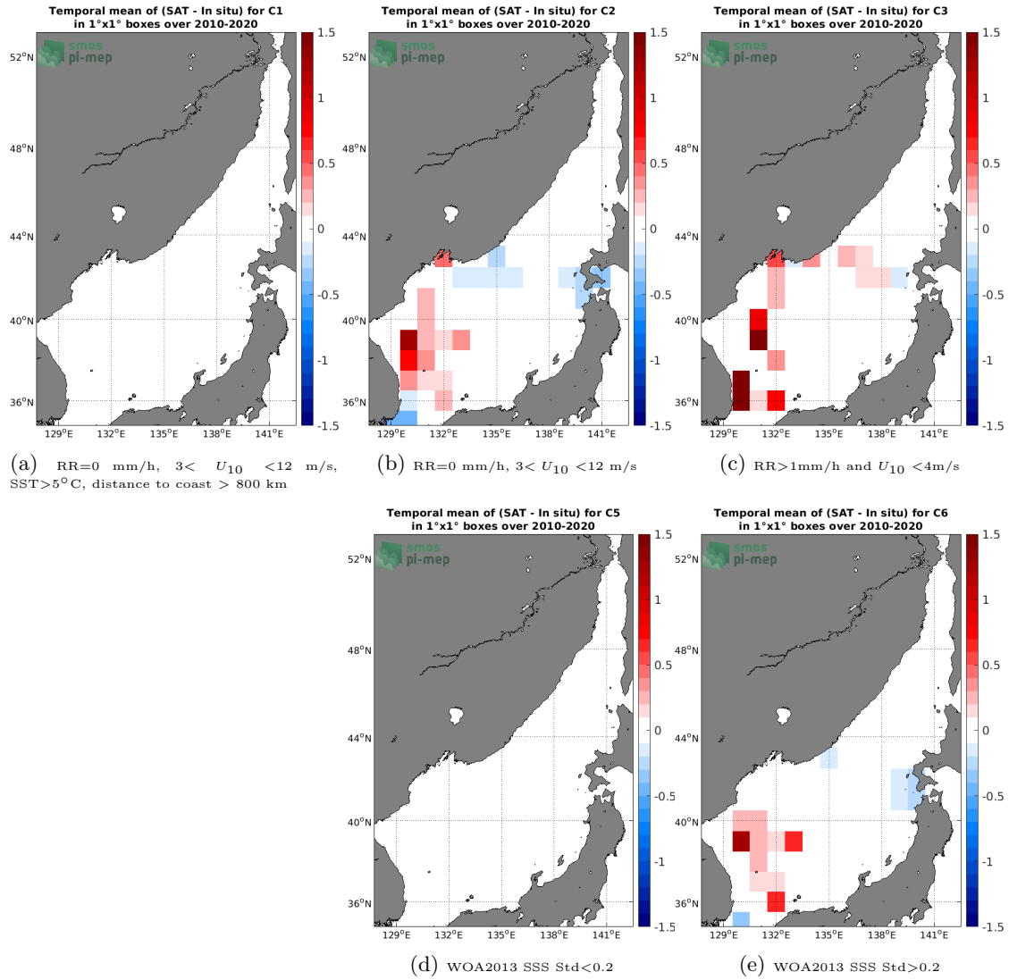
Figure 12: Temporal mean gridded over spatial boxes of size 1°x1° of \Delta SSS (CCI SSS L4 Merged-OI v3.2 - 30-day running (ESA) - TSG (LEGOS-DM)) for 5 different subdatasets corresponding to:RR=0 mm/h, 3 < U_{10} < 12 m/s, SST>5°C, distance to coast > 800 km (a), RR=0 mm/h, 3 < U_{10} < 12 m/s (b), RR>1mm/h and U_{10} < 4 m/s (c), WOA2013 SSS Std<0.2 (d), WOA2013 SSS Std>0.2 (e).
