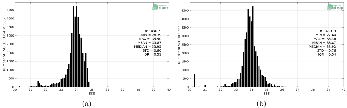
Figure 2: Histograms of SSS from TSG (LEGOS-DM) (a) and CCI SSS L4 Merged-OI v3.2 - 30-day running (ESA) (b) considering all match-up pairs per bins of 0.1 over the Sea of Japan Pi-MEP region and for the full satellite product period.
