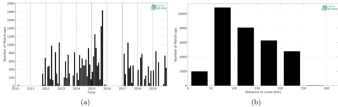
Figure 1: Number of match-ups between TSG (LEGOS-DM) and CCI SSS L4 Merged-OI v2.31 - 30-day running (ESA) SSS as a function of time (a) and as function of the distance to coast (b) over the Sea of Japan Pi-MEP region and for the full satellite product period.
