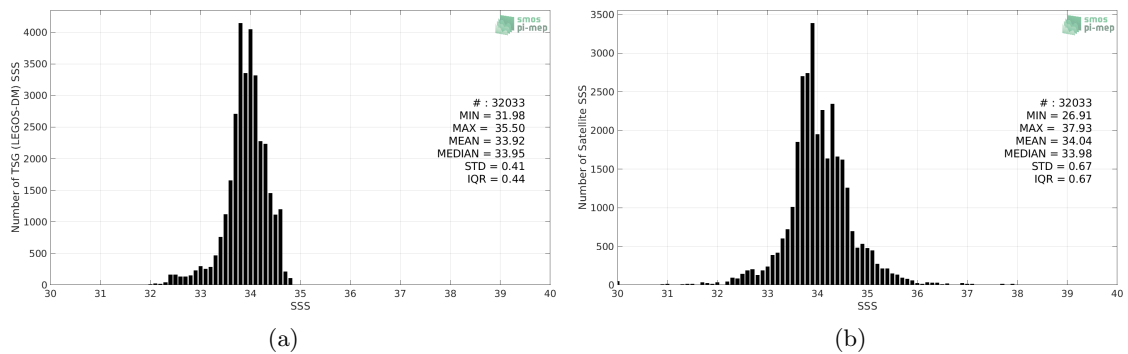
Figure 2: Histograms of SSS from TSG (LEGOS-DM) (a) and CCI SSS L4 Merged-OI v2.31 - 30-day running (ESA) (b) considering all match-up pairs per bins of 0.1 over the Sea of Japan Pi-MEP region and for the full satellite product period.
