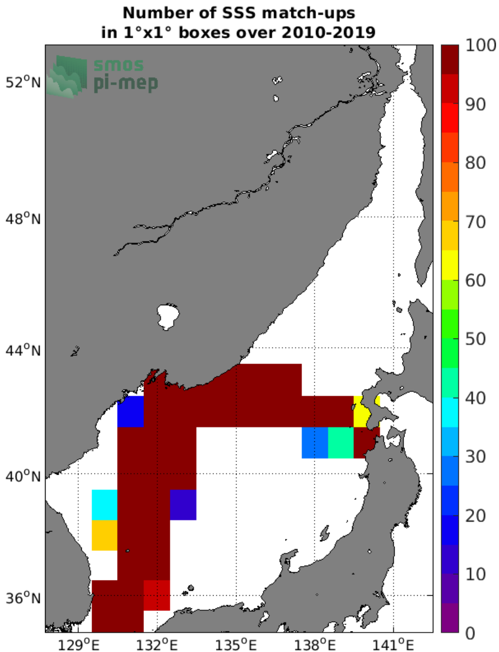
Figure 4: Number of SSS match-ups between TSG (LEGOS-DM) SSS and the CCI SSS L4 Merged-OI v2.31 - 30-day running (ESA) SSS product for the Sea of Japan Pi-MEP region over 1°x1° boxes and for the full satellite product period.
