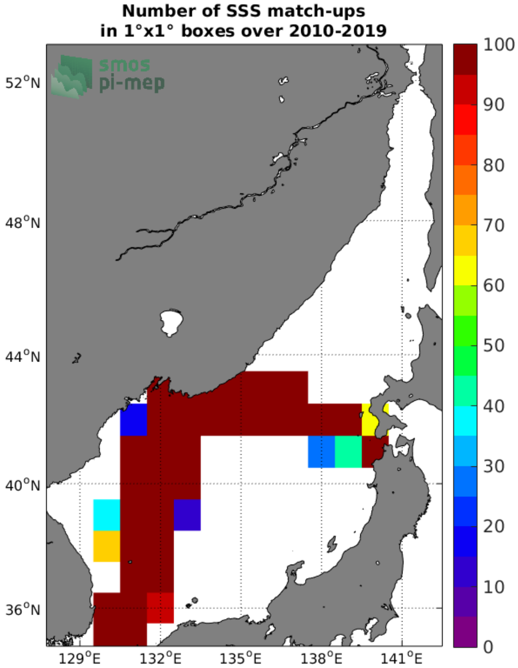
Figure 4: Number of SSS match-ups between TSG (LEGOS-DM) SSS and the CCI L4 Merged-OI v2.31 - 30-day running (ESA) SSS product for the Sea of Japan Pi-MEP region over 1°x1° boxes and for the full satellite product period.
