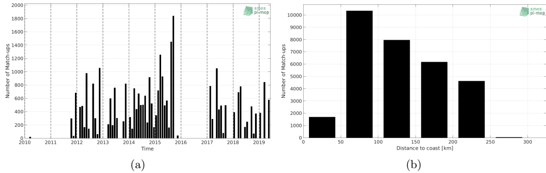
Figure 1: Number of match-ups between TSG (LEGOS-DM) and CCI L4 Merged-OI v2.31 - 30-day running (ESA) SSS as a function of time (a) and as function of the distance to coast (b) over the Sea of Japan Pi-MEP region and for the full satellite product period.
