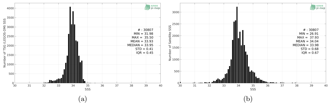
Figure 2: Histograms of SSS from TSG (LEGOS-DM) (a) and CCI L4 Merged-OI v2.31 - 30-day running (ESA) (b) considering all match-up pairs per bins of 0.1 over the Sea of Japan Pi-MEP region and for the full satellite product period.
