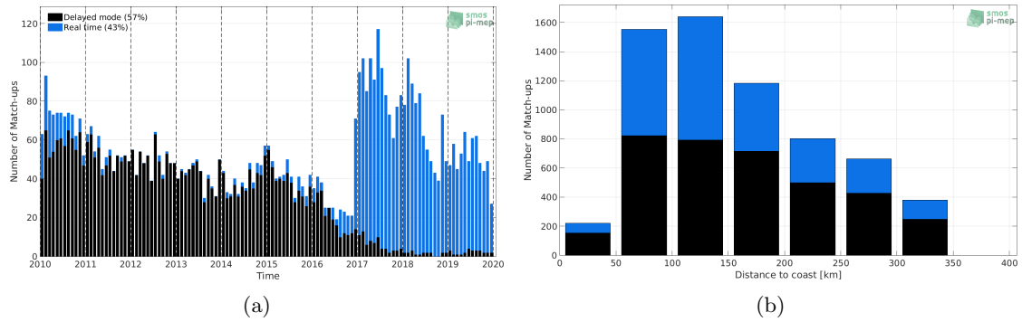
Figure 1: Number of match-ups between Argo and CCI L4 Merged-OI v2.31 - 30-day running (ESA) SSS as a function of time (a) and as function of the distance to coast (b) over the Sea of Japan Pi-MEP region and for the full satellite product period.
