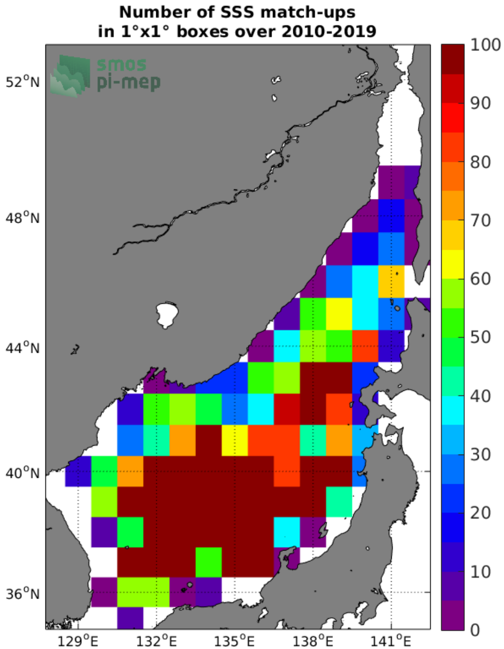
Figure 4: Number of SSS match-ups between Argo SSS and the CCI L4 Merged-OI v2.31 - 30-day running (ESA) SSS product for the Sea of Japan Pi-MEP region over 1°x1° boxes and for the full satellite product period.
