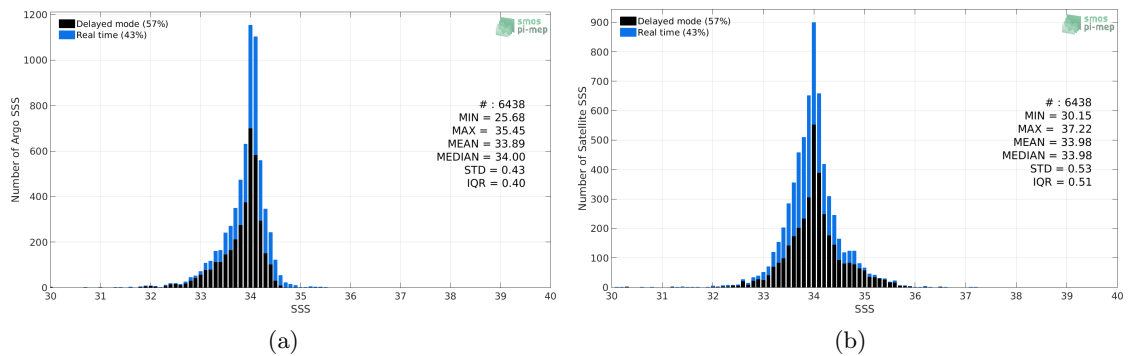
Figure 2: Histograms of SSS from Argo (a) and CCI L4 Merged-OI v2.31 - 30-day running (ESA) (b) considering all match-up pairs per bins of 0.1 over the Sea of Japan Pi-MEP region and for the full satellite product period.
