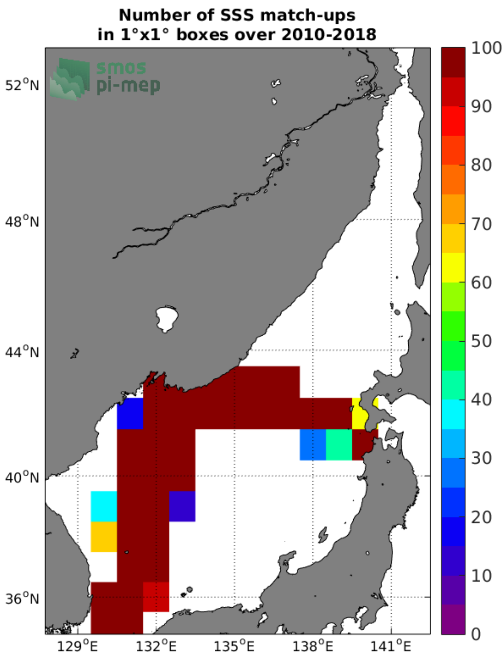
Figure 4: Number of SSS match-ups between TSG-LEGOS-DM SSS and the CCI L4 Merged-OI v1.8 - 7-day running (ESA) SSS product for the Sea of Japan Pi-MEP region over 1°x1° boxes and for the full satellite product period.
