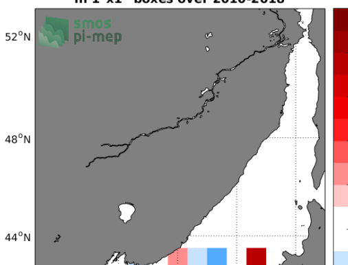
Temporal mean of (Sat - TSG-LEGOS-DM) in 1°x1° boxes over 2010-2018
