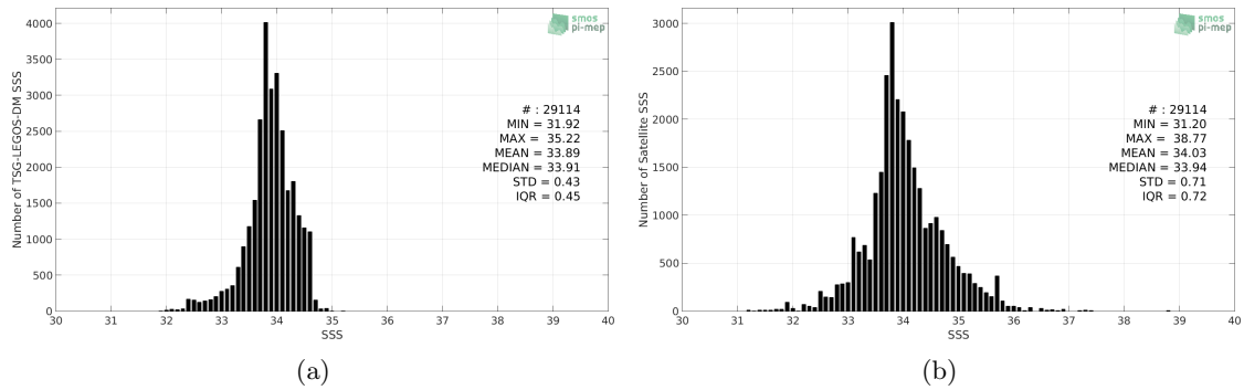
Figure 2: Histograms of SSS from TSG-LEGOS-DM (a) and CCI L4 Merged-OI v1.8 - 7-day running (ESA) (b) considering all match-up pairs per bins of 0.1 over the Sea of Japan Pi-MEP region and for the full satellite product period.
