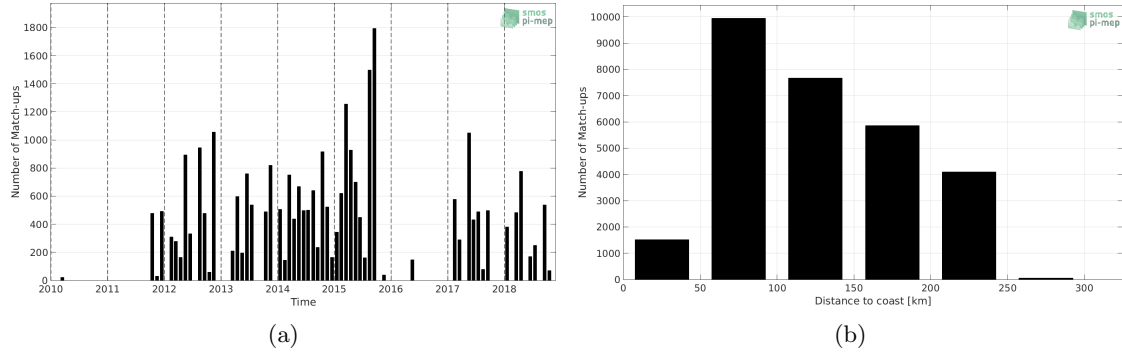
Figure 1: Number of match-ups between TSG-LEGOS-DM and CCI L4 Merged-OI v1.8 - 7-day running (ESA) SSS as a function of time (a) and as function of the distance to coast (b) over the Sea of Japan Pi-MEP region and for the full satellite product period.
