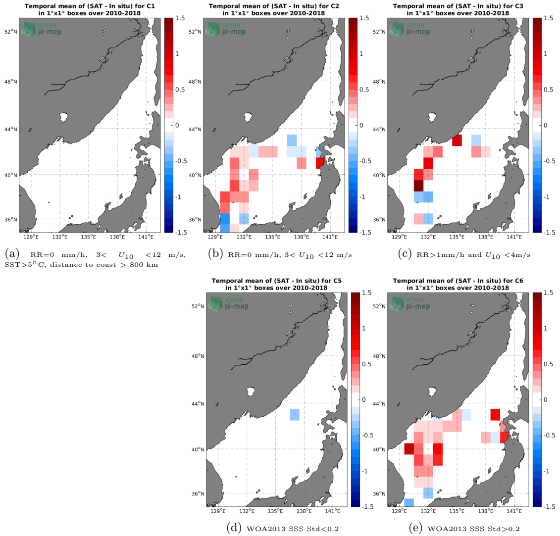
Figure 12: Temporal mean gridded over spatial boxes of size 1^\circ \times 1^\circ of \Delta SSS (CCI L4 Merged-OI v1.8 - 7-day running (ESA) - TSG-LEGOS-DM) for 5 different subdatasets corresponding to: RR=0 mm/h, 3 < U_{10} < 12 m/s, SST > 5^\circ\text{C} , distance to coast > 800 km (a), RR=0 mm/h, 3 < U_{10} < 12 m/s (b), RR > 1\text{mm/h} and U_{10} < 4\text{m/s} (c), WOA2013 SSS Std < 0.2 (d), WOA2013 SSS Std > 0.2 (e).
