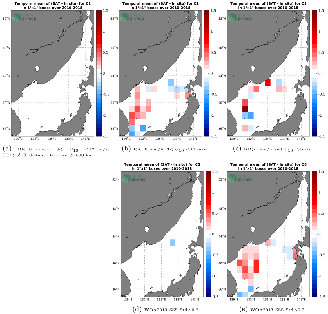
Figure 12: Temporal mean gridded over spatial boxes of size 1°x1° of \Delta SSS (CCI-L4-ESAMERGED-OI-V1.8-30DAY-RUNNING - TSG-LEGOS-DM) for 5 different subdatasets corresponding to: RR=0 mm/h, 3 < U_{10} < 12 m/s, SST > 5^\circ\text{C} , distance to coast > 800 km (a), RR=0 mm/h, 3 < U_{10} < 12 m/s (b), RR > 1 mm/h and U_{10} < 4 m/s (c), WOA2013 SSS Std < 0.2 (d), WOA2013 SSS Std > 0.2 (e).
