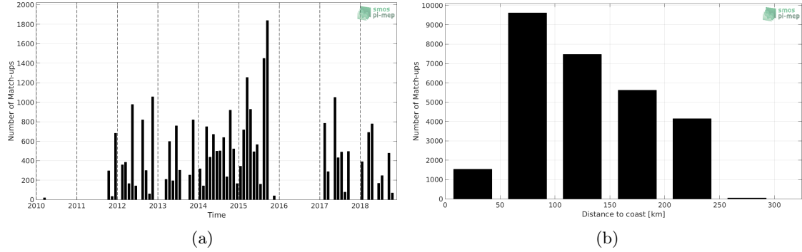
Figure 1: Number of match-ups between TSG-LEGOS-DM and CCI-L4-ESA-MERGED-OI-V1.8-30DAY-RUNNING SSS as a function of time (a) and as function of the distance to coast (b) over the Sea of Japan Pi-MEP region and for the full satellite product period.
