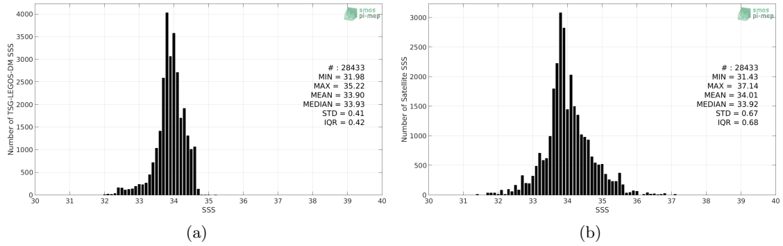
Figure 2: Histograms of SSS from TSG-LEGOS-DM (a) and CCI-L4-ESA-MERGED-OI-V1.8-30DAY-RUNNING (b) considering all match-up pairs per bins of 0.1 over the Sea of Japan Pi-MEP region and for the full satellite product period.
