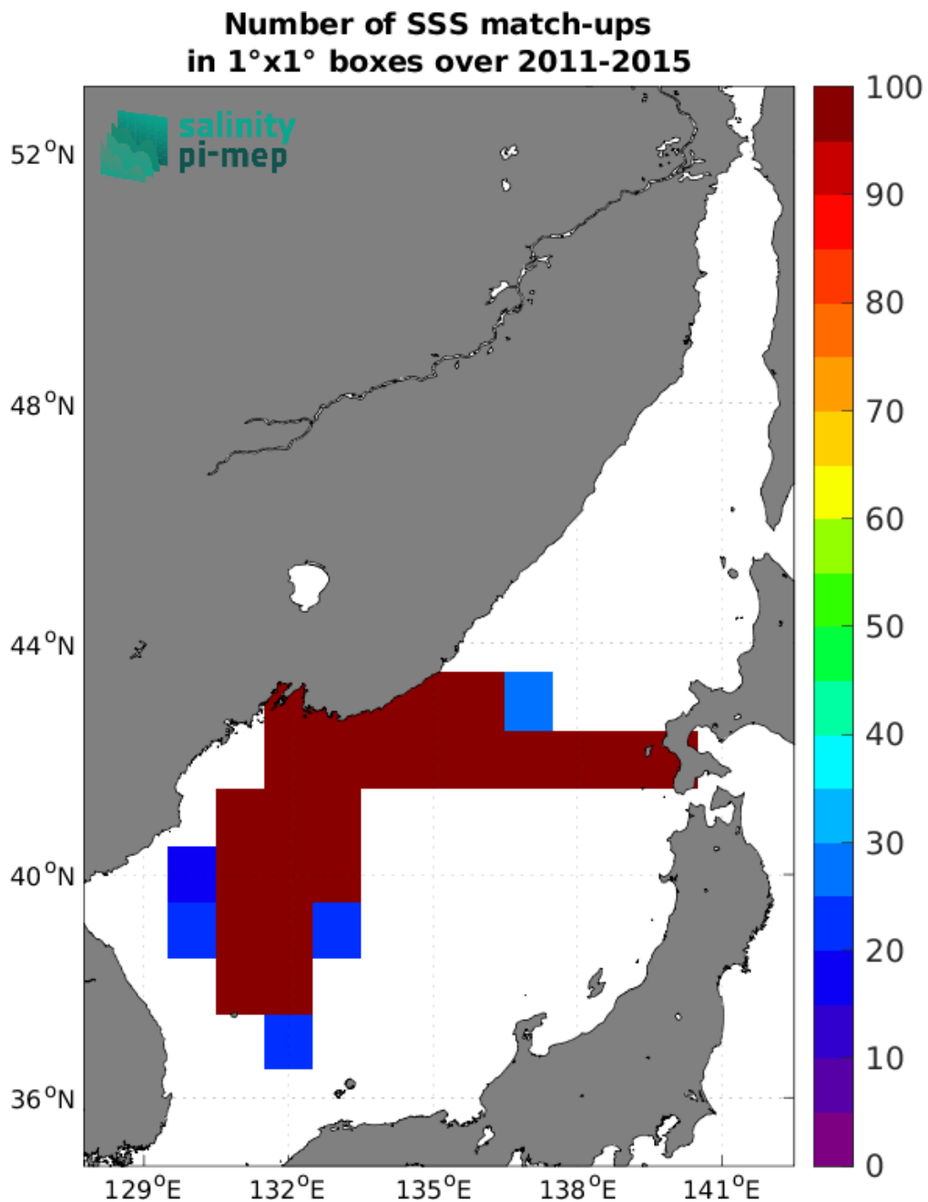
Figure 5: Number of SSS match-ups between TSG (LEGOS-DM) SSS and the Aquarius SSS L4 OI v5 - Weekly (IPRC) SSS product for the Sea of Japan Pi-MEP region over 1°×1° boxes and for the full satellite product period.
