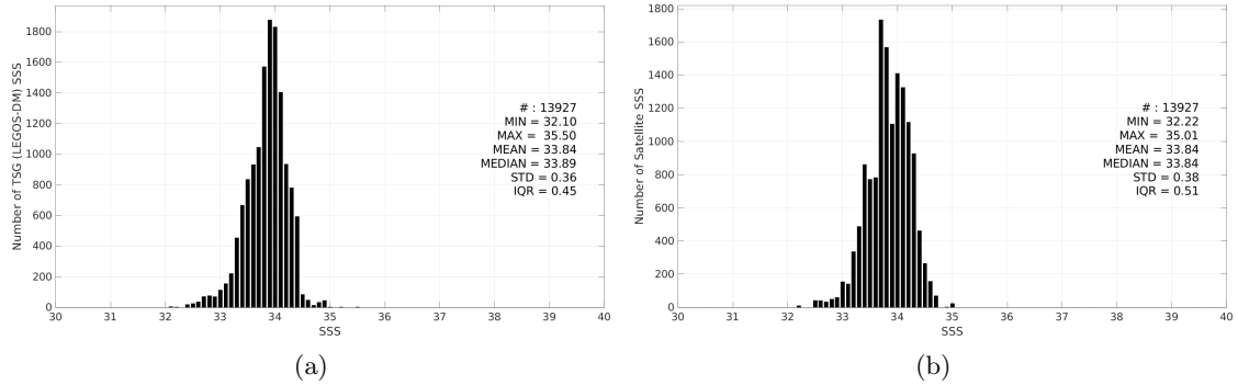
Figure 3: Histograms of SSS from TSG (LEGOS-DM) (a) and Aquarius SSS L4 OI v5 - Weekly (IPRC) (b) considering all match-up pairs per bins of 0.1 over the Sea of Japan Pi-MEP region and for the full satellite product period.
