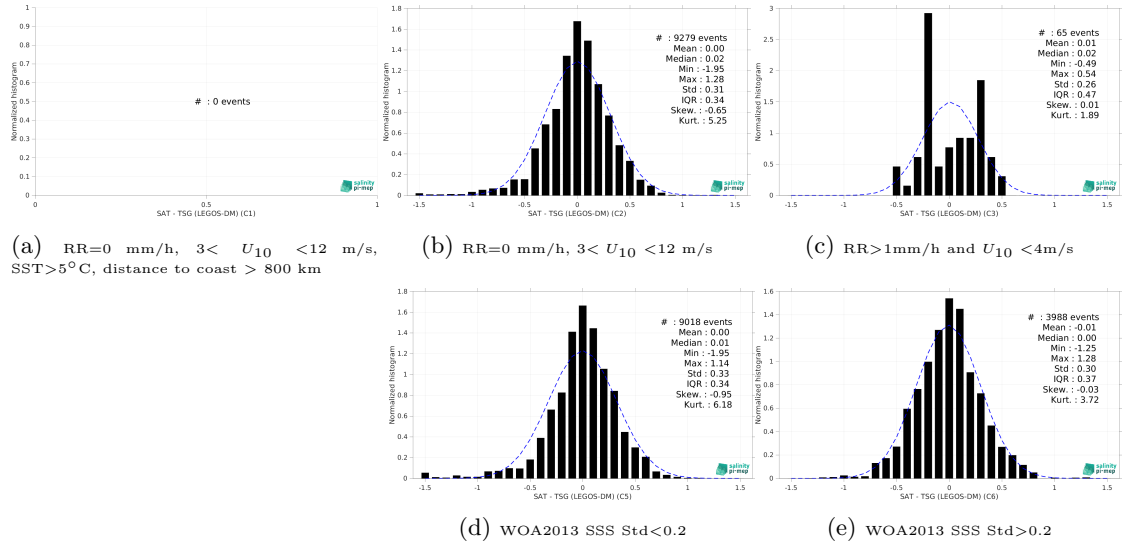
Figure 15: Normalized histogram of \Delta SSS (Aquarius SSS L4 OI v5 - Weekly (IPRC) - TSG (LEGOS-DM)) for 5 different subdatasets corresponding to: RR=0 mm/h, 3 < U_{10} < 12 m/s, SST > 5°C, distance to coast > 800 km (a), RR=0 mm/h, 3 < U_{10} < 12 m/s (b), RR > 1mm/h and U_{10} < 4 m/s (c), WOA2013 SSS Std < 0.2 (d), WOA2013 SSS Std > 0.2 (e).
