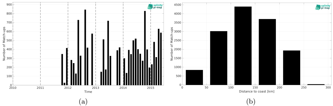
Figure 2: Number of match-ups between TSG (LEGOS-DM) and Aquarius SSS L4 OI v5 - Weekly (IPRC) SSS as a function of time (a) and as function of the distance to coast (b) over the Sea of Japan Pi-MEP region and for the full satellite product period.
