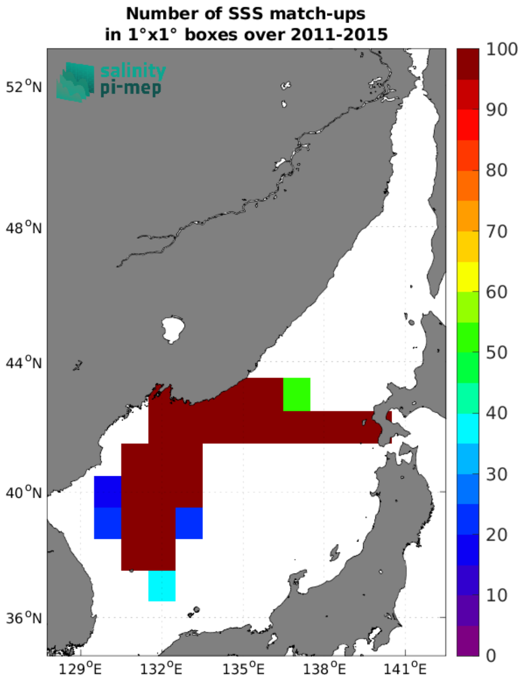
Figure 4: Number of SSS match-ups between TSG (LEGOS-DM) SSS and the Aquarius SSS L4 OI v5 - Weekly (IPRC) SSS product for the Sea of Japan Pi-MEP region over 1°×1° boxes and for the full satellite product period.
