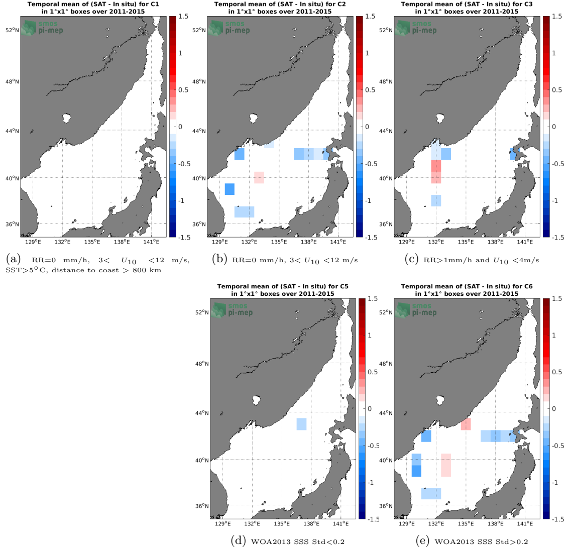
Figure 12: Temporal mean gridded over spatial boxes of size 1^\circ \times 1^\circ of \Delta SSS (Aquarius SSS L4 OI v5 - Weekly (IPRC) - TSG (LEGOS-DM)) for 5 different subdatasets corresponding to: RR=0 mm/h, 3 < U_{10} < 12 m/s, SST>5°C, distance to coast > 800 km (a), RR=0 mm/h, 3 < U_{10} < 12 m/s (b), RR>1mm/h and U_{10} < 4 m/s (c), WOA2013 SSS Std<0.2 (d), WOA2013 SSS Std>0.2 (e).
