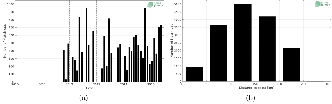
Figure 1: Number of match-ups between TSG (LEGOS-DM) and Aquarius SSS L4 OI v5 - Weekly (IPRC) SSS as a function of time (a) and as function of the distance to coast (b) over the Sea of Japan Pi-MEP region and for the full satellite product period.
