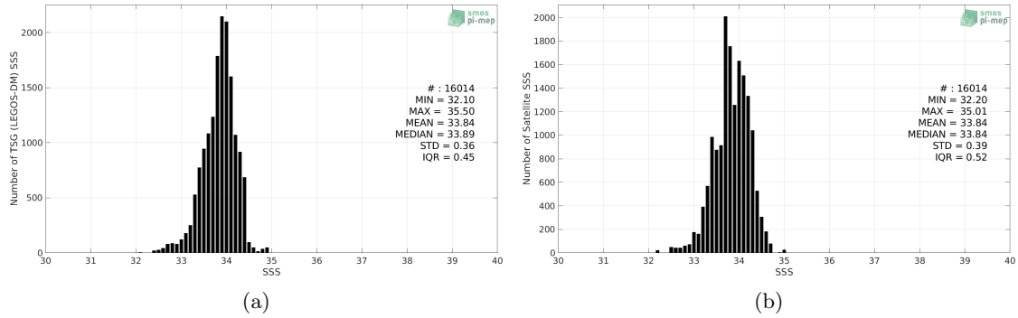
Figure 2: Histograms of SSS from TSG (LEGOS-DM) (a) and Aquarius SSS L4 OI v5 - Weekly (IPRC) (b) considering all match-up pairs per bins of 0.1 over the Sea of Japan Pi-MEP region and for the full satellite product period.
