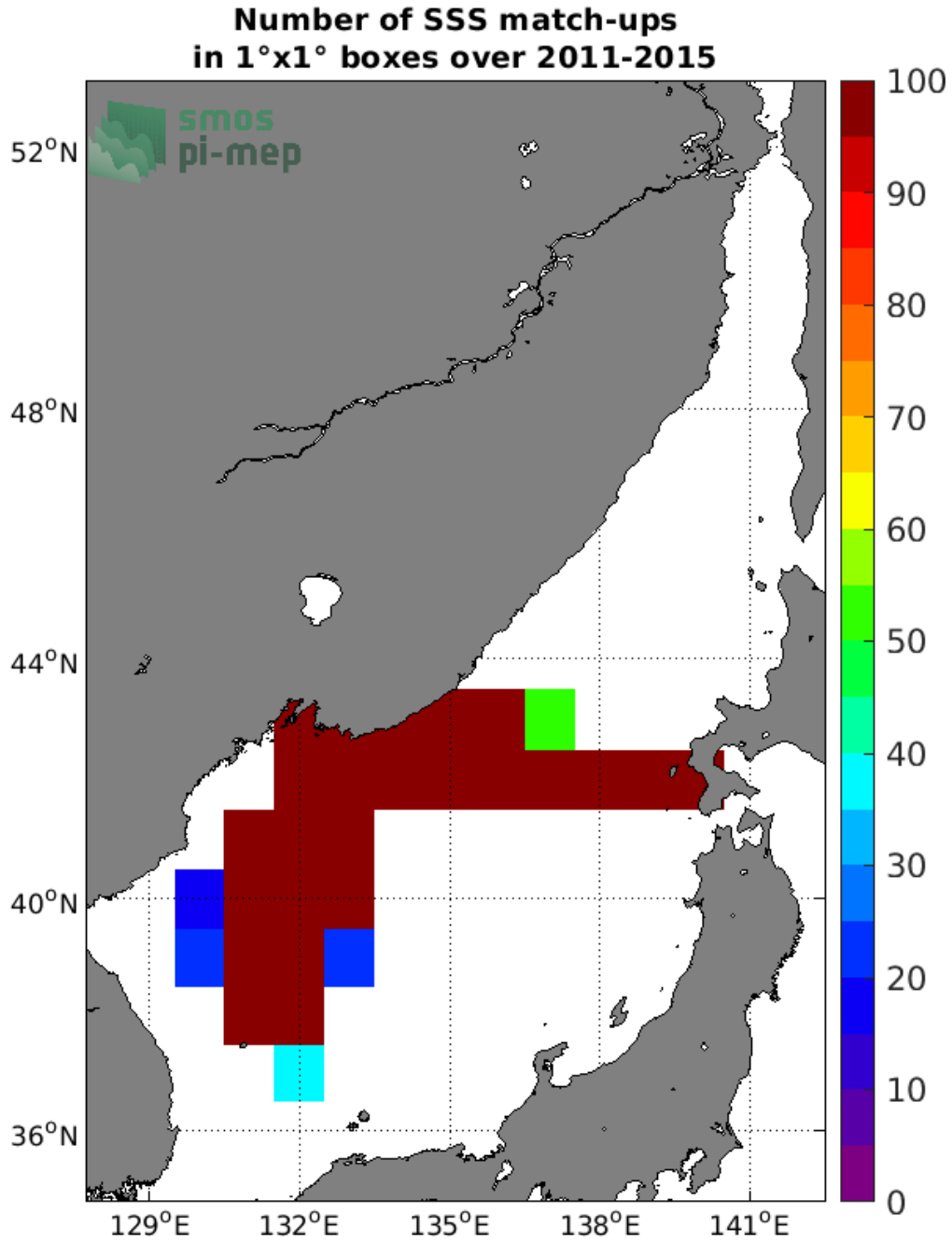
Figure 4: Number of SSS match-ups between TSG (LEGOS-DM) SSS and the Aquarius SSS L4 OI v5 - Weekly (IPRC) SSS product for the Sea of Japan Pi-MEP region over 1°x1° boxes and for the full satellite product period.
