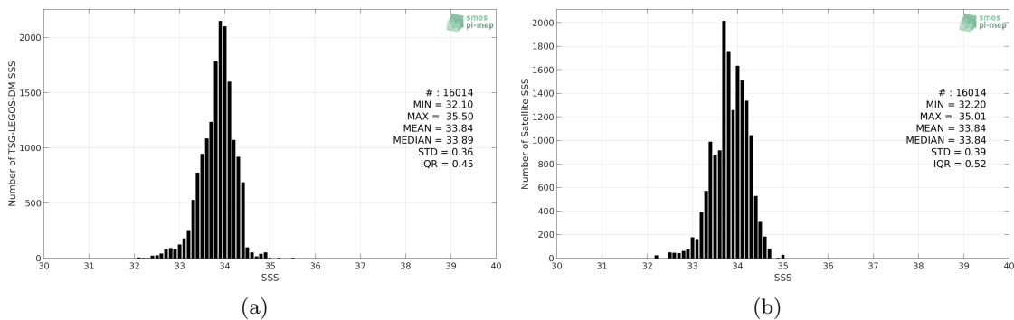
Figure 2: Histograms of SSS from TSG-LEGOS-DM (a) and Aquarius-L4-IPRC-V5-WEEKLY (b) considering all match-up pairs per bins of 0.1 over the Sea of Japan Pi-MEP region and for the full satellite product period.
