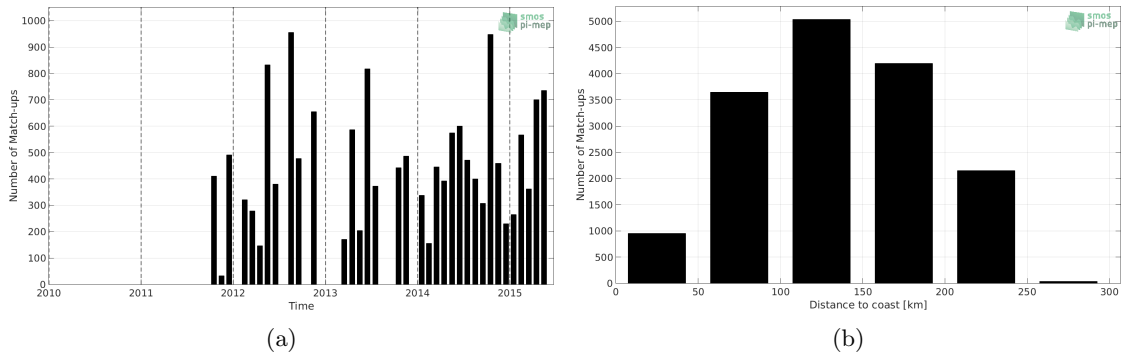
Figure 1: Number of match-ups between TSG-LEGOS-DM and Aquarius-L4-IPRC-V5-WEEKLY SSS as a function of time (a) and as function of the distance to coast (b) over the Sea of Japan Pi-MEP region and for the full satellite product period.
