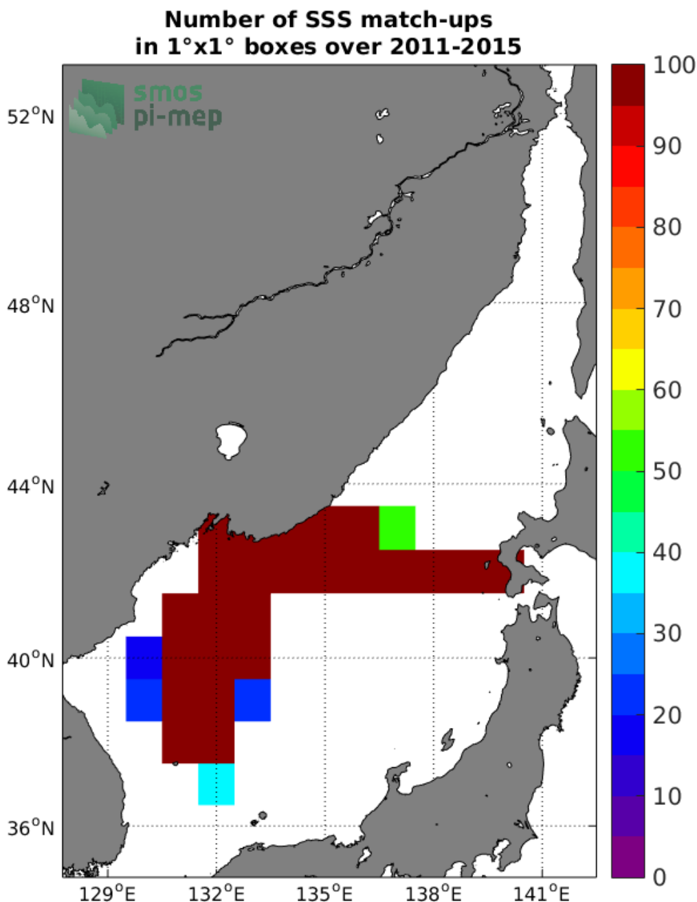
Figure 4: Number of SSS match-ups between TSG-LEGOS-DM SSS and the Aquarius-L4-IPRC-V5-WEEKLY SSS product for the Sea of Japan Pi-MEP region over 1°x1° boxes and for the full satellite product period.
