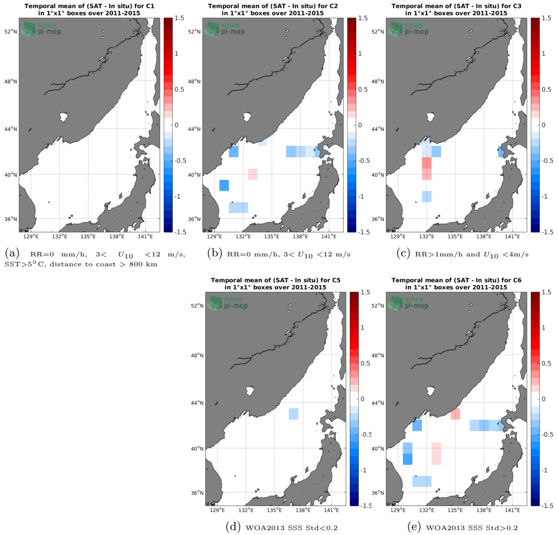
Figure 12: Temporal mean gridded over spatial boxes of size 1°x1° of \Delta\text{SSS} (Aquarius-L4-IPRC-V5-WEEKLY - TSG-LEGOS-DM) for 5 different subdatasets corresponding to: RR=0 mm/h, 3 < U_{10} < 12 m/s, SST > 5^\circ\text{C} , distance to coast > 800 km (a), RR=0 mm/h, 3 < U_{10} < 12 m/s (b), RR > 1 mm/h and U_{10} < 4 m/s (c), WOA2013 SSS Std < 0.2 (d), WOA2013 SSS Std > 0.2 (e).
