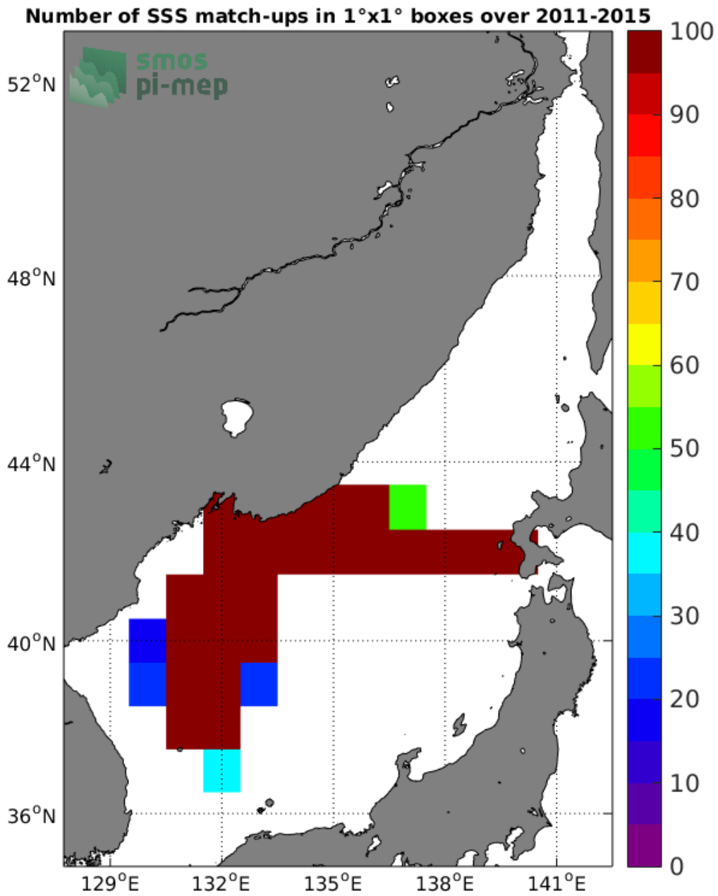
Figure 4: Number of SSS match-ups between TSG-LEGOS-DM SSS and the Aquarius-L4-IPRC-V5-WEEKLY SSS product for the Sea of Japan Pi-MEP region over 1°x1° boxes and for the full satellite product period.
