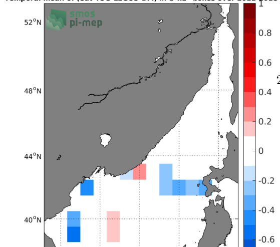
Temporal mean of (Sat-TSG-LEGOS-DM) in 1°x1° boxes over 2011-2015
