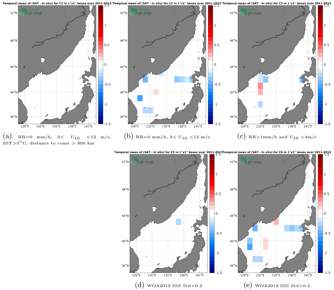
Figure 12: Temporal mean gridded over spatial boxes of size 1^\circ \times 1^\circ of \Delta SSS (Aquarius-L4-IPRC-V5-WEEKLY - TSG-LEGOS-DM) for 5 different subdatasets corresponding to: RR=0 mm/h, 3 < U_{10} < 12 m/s, SST > 5^\circ C , distance to coast > 800 km (a), RR=0 mm/h, 3 < U_{10} < 12 m/s (b), RR > 1 mm/h and U_{10} < 4 m/s (c), WOA2013 SSS Std < 0.2 (d), WOA2013 SSS Std > 0.2 (e).
