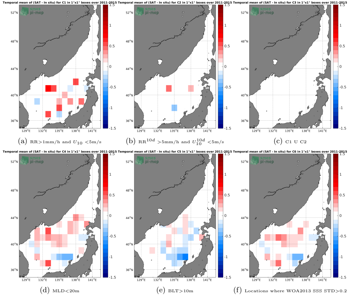
Figure 12: Temporal mean gridded over spatial boxes of size 1°x1° of \Delta SSS (Aquarius-L4-IPRC-V5-WEEKLY - Argo) for 6 different subdatasets corresponding to:RR>1mm/h and U_{10} < 5\text{m/s} (a), RR^{10d} > 5\text{mm/h} and U_{10}^{10d} < 5\text{m/s} (b), C1 U C2 (c),MLD<20m (d),BLT>10m (e),Locations where WOA2013 SSS STD>0.2 (f).
