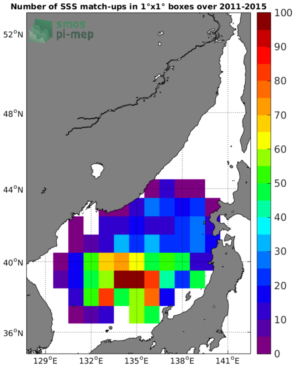
Figure 4: Number of SSS match-ups between Argo SSS and the Aquarius-L4-IPRC-V5-WEEKLY SSS product for the Sea of Japan Pi-MEP region over 1°x1° boxes and for the full satellite product period.
