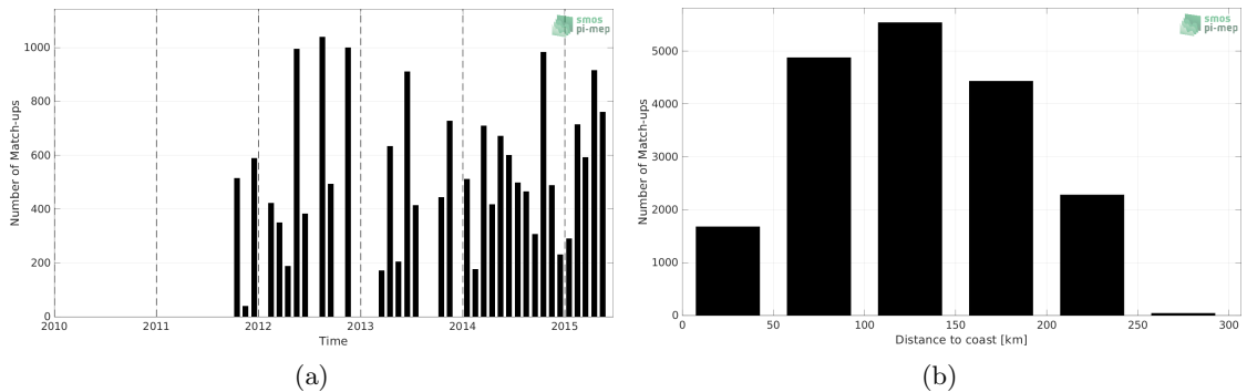
Figure 1: Number of match-ups between TSG (LEGOS-DM) and Aquarius SSS L4 OI v5 - Monthly (IPRC) SSS as a function of time (a) and as function of the distance to coast (b) over the Sea of Japan Pi-MEP region and for the full satellite product period.
