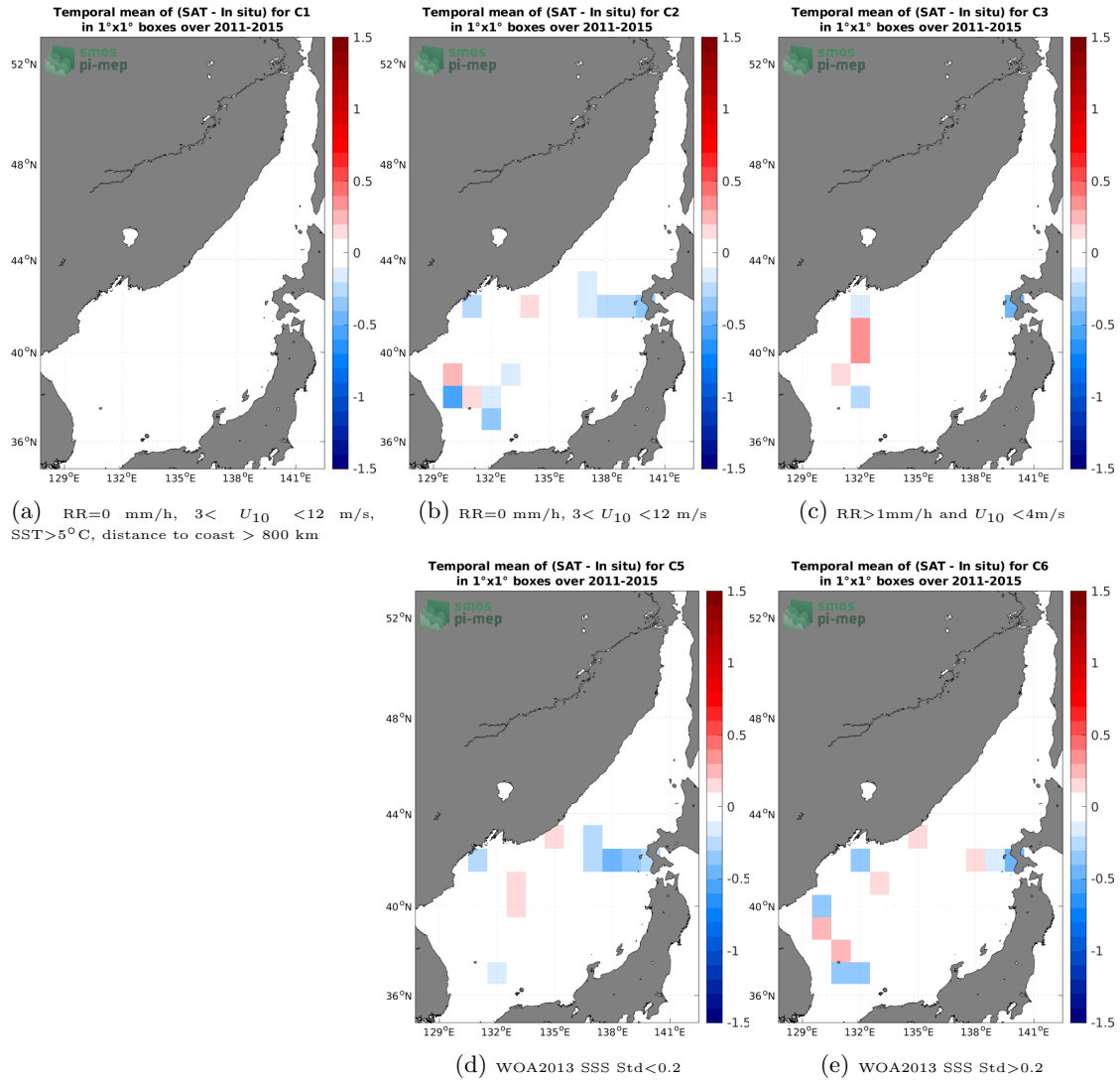
Figure 12: Temporal mean gridded over spatial boxes of size 1^\circ \times 1^\circ of \Delta\text{SSS} (Aquarius SSS L4 OI v5 - Monthly (IPRC) - TSG (LEGOS-DM)) for 5 different subdatasets corresponding to: RR=0 mm/h, 3 < U_{10} < 12 m/s, SST > 5^\circ\text{C} , distance to coast > 800 km (a), RR=0 mm/h, 3 < U_{10} < 12 m/s (b), RR > 1 mm/h and U_{10} < 4 m/s (c), WOA2013 SSS Std < 0.2 (d), WOA2013 SSS Std > 0.2 (e).
