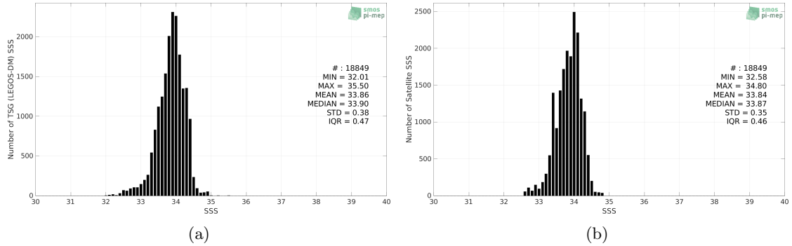
Figure 2: Histograms of SSS from TSG (LEGOS-DM) (a) and Aquarius SSS L4 OI v5 - Monthly (IPRC) (b) considering all match-up pairs per bins of 0.1 over the Sea of Japan Pi-MEP region and for the full satellite product period.
