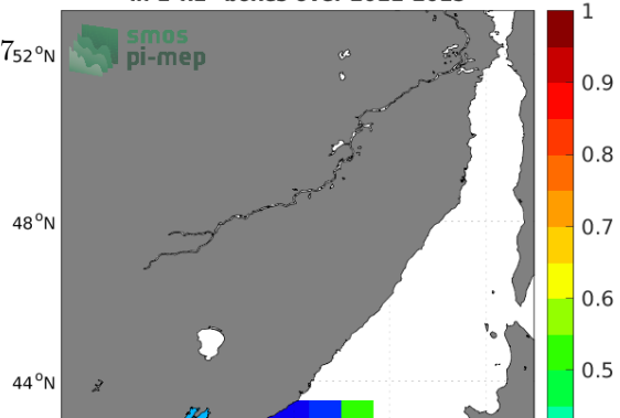
Temporal STD of (Sat - TSG (LEGOS-DM)) in 1°x1° boxes over 2011-2015
