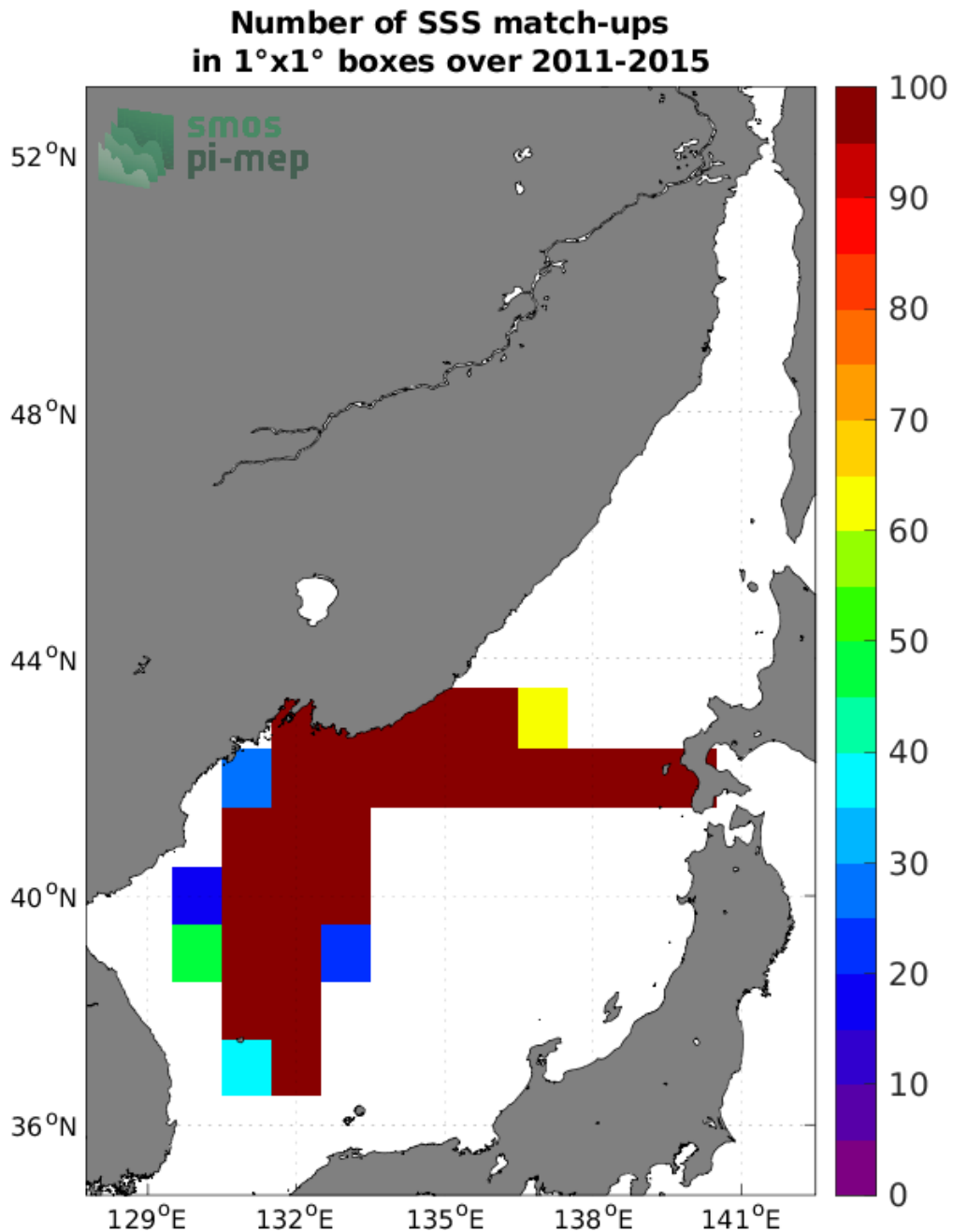
Figure 4: Number of SSS match-ups between TSG (LEGOS-DM) SSS and the Aquarius SSS L4 OI v5 - Monthly (IPRC) SSS product for the Sea of Japan Pi-MEP region over 1°x1° boxes and for the full satellite product period.
