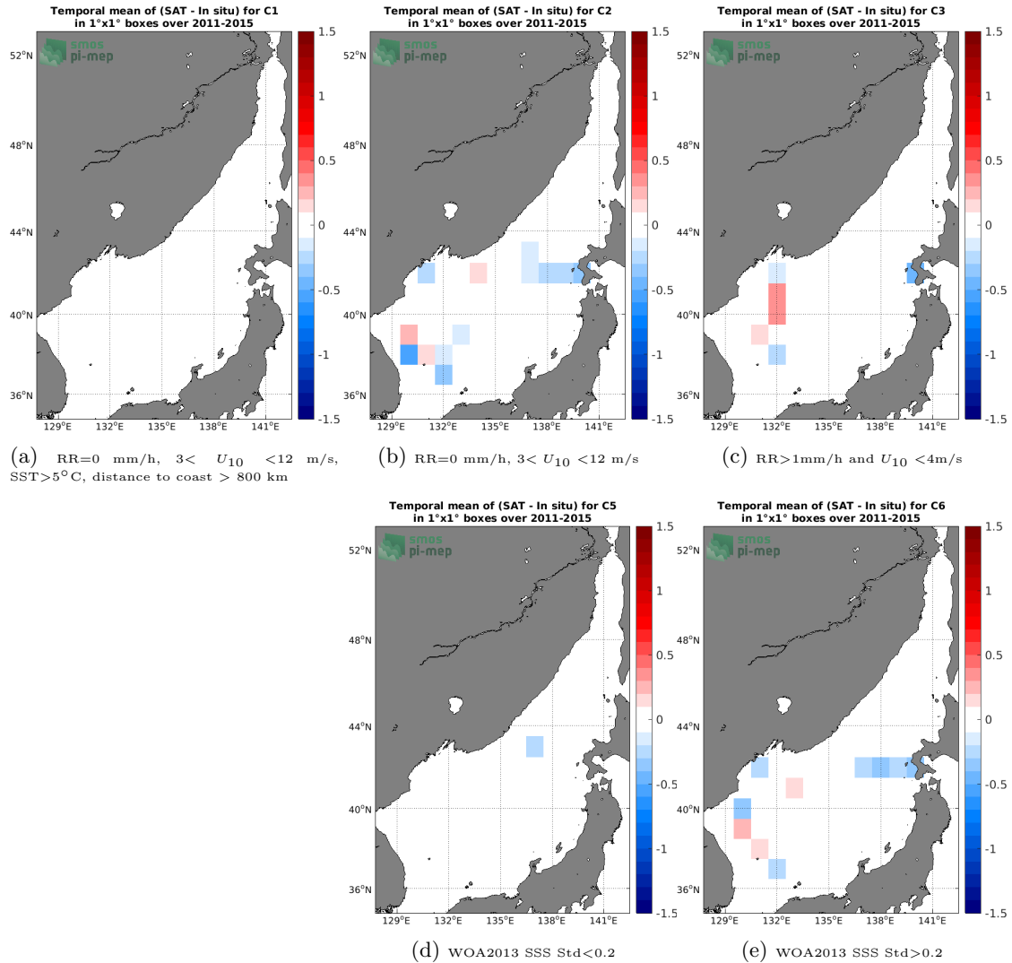
Figure 12: Temporal mean gridded over spatial boxes of size 1^\circ \times 1^\circ of \Delta SSS (Aquarius SSS L4 OI v5 - Monthly (IPRC) - TSG (LEGOS-DM)) for 5 different subdatasets corresponding to: RR=0 mm/h, 3 < U_{10} < 12 m/s, SST > 5°C, distance to coast > 800 km (a), RR=0 mm/h, 3 < U_{10} < 12 m/s (b), RR > 1mm/h and U_{10} < 4 m/s (c), WOA2013 SSS Std < 0.2 (d), WOA2013 SSS Std > 0.2 (e).
