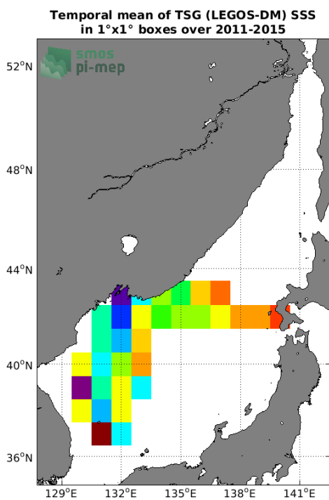
(c) MEAN(TSG (LEGOS-DM) SSS)
