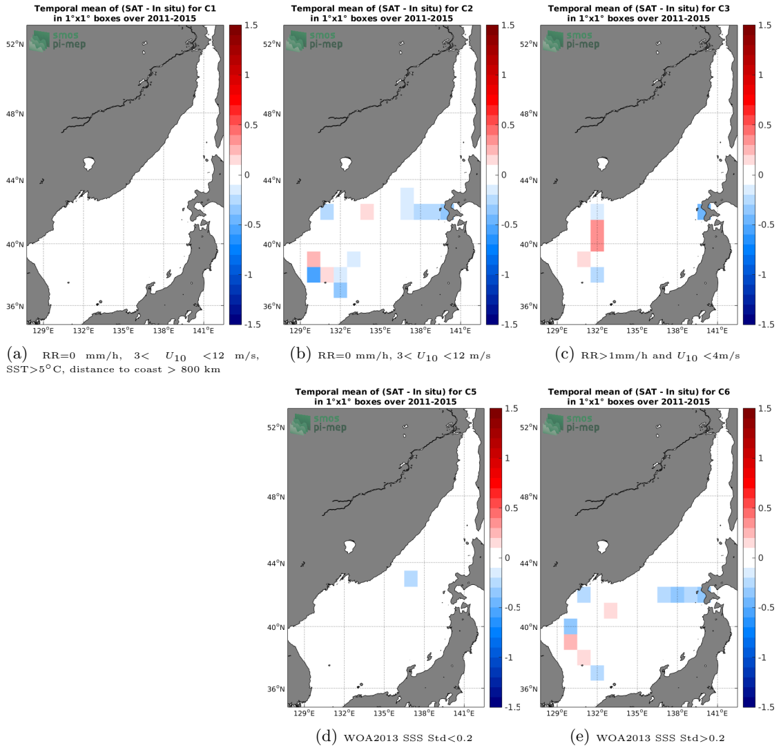
Figure 12: Temporal mean gridded over spatial boxes of size 1°x1° of \Delta\text{SSS} (Aquarius-L4-IPRC-V5-MONTHLY - TSG-LEGOS-DM) for 5 different subdatasets corresponding to: RR=0 mm/h, 3 < U_{10} < 12 m/s, SST > 5^\circ\text{C} , distance to coast > 800 km (a), RR=0 mm/h, 3 < U_{10} < 12 m/s (b), RR > 1 mm/h and U_{10} < 4 m/s (c), WOA2013 SSS Std < 0.2 (d), WOA2013 SSS Std > 0.2 (e).
