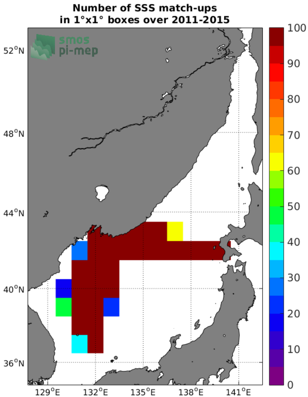
Figure 4: Number of SSS match-ups between TSG-LEGOS-DM SSS and the Aquarius-L4-IPRC-V5-MONTHLY SSS product for the Sea of Japan Pi-MEP region over 1°x1° boxes and for the full satellite product period.
