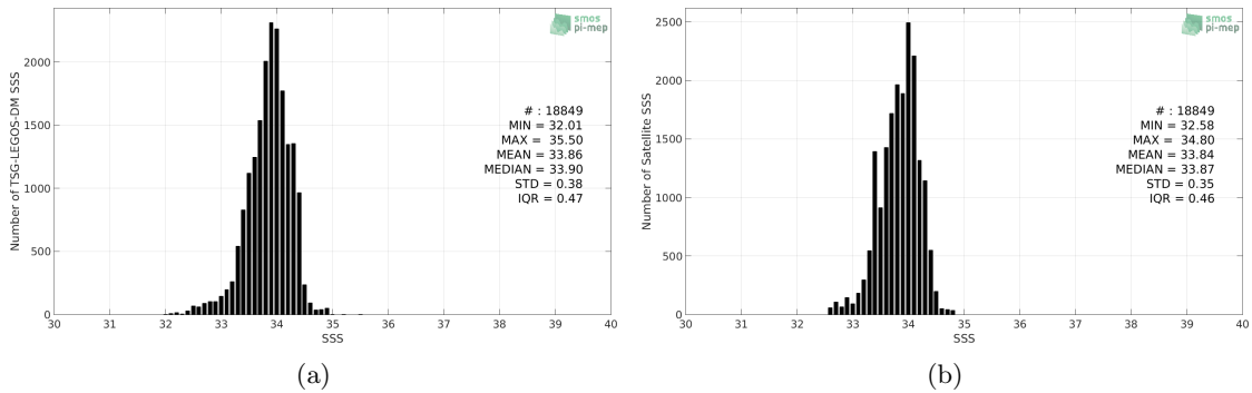
Figure 2: Histograms of SSS from TSG-LEGOS-DM (a) and Aquarius-L4-IPRC-V5-MONTHLY (b) considering all match-up pairs per bins of 0.1 over the Sea of Japan Pi-MEP region and for the full satellite product period.
