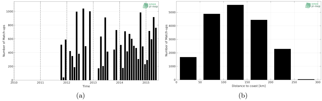
Figure 1: Number of match-ups between TSG-LEGOS-DM and Aquarius-L4-IPRC-V5-MONTHLY SSS as a function of time (a) and as function of the distance to coast (b) over the Sea of Japan Pi-MEP region and for the full satellite product period.
