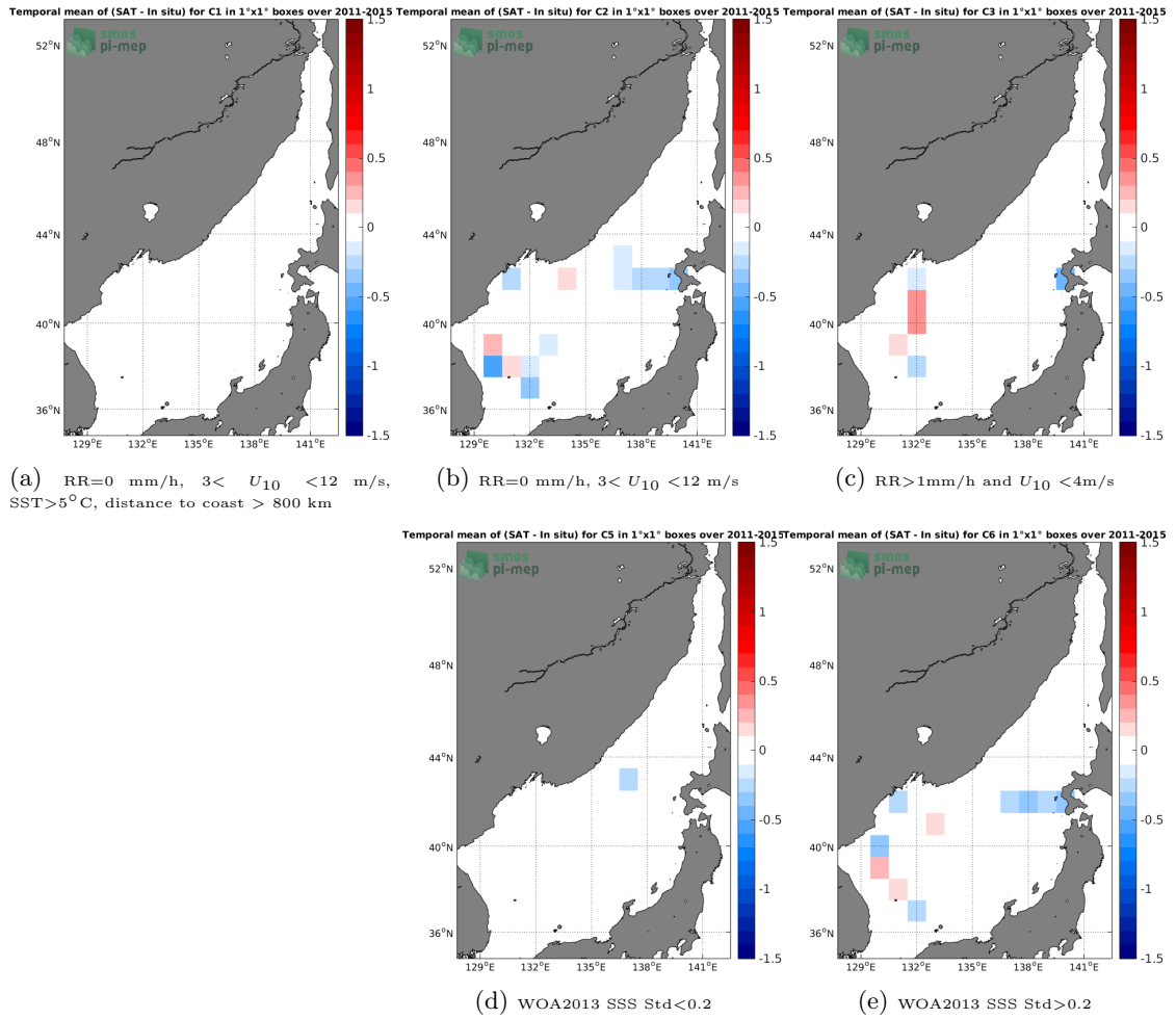
Figure 12: Temporal mean gridded over spatial boxes of size 1^\circ \times 1^\circ of \Delta SSS (Aquarius-L4-IPRC-V5-MONTHLY - TSG-LEGOS-DM) for 5 different subdatasets corresponding to: RR=0 mm/h, 3 < U_{10} < 12 m/s, SST > 5^\circ C , distance to coast > 800 km (a), RR=0 mm/h, 3 < U_{10} < 12 m/s (b), RR > 1 mm/h and U_{10} < 4 m/s (c), WOA2013 SSS Std < 0.2 (d), WOA2013 SSS Std > 0.2 (e).
