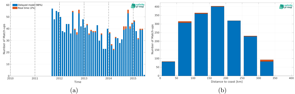
Figure 2: Number of match-ups between Argo and Aquarius SSS L4 OI v5 - Monthly (IPRC) SSS as a function of time (a) and as function of the distance to coast (b) over the Sea of Japan Pi-MEP region and for the full satellite product period.
