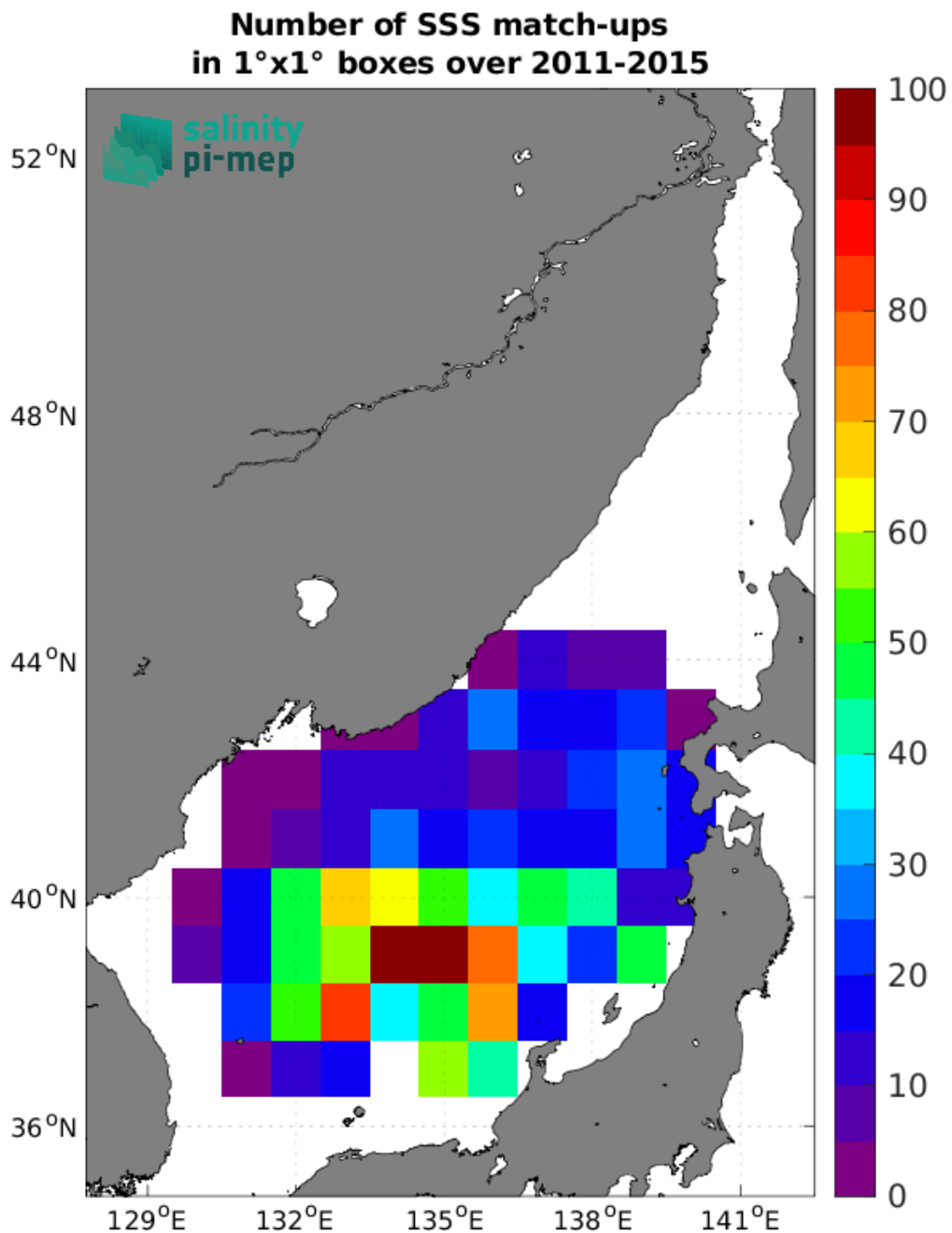
Figure 5: Number of SSS match-ups between Argo SSS and the Aquarius SSS L4 OI v5 - Monthly (IPRC) SSS product for the Sea of Japan Pi-MEP region over 1°x1° boxes and for the full satellite product period.
