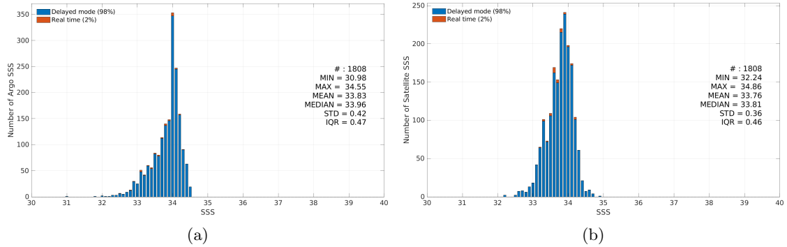
Figure 3: Histograms of SSS from Argo (a) and Aquarius SSS L4 OI v5 - Monthly (IPRC) (b) considering all match-up pairs per bins of 0.1 over the Sea of Japan Pi-MEP region and for the full satellite product period.
