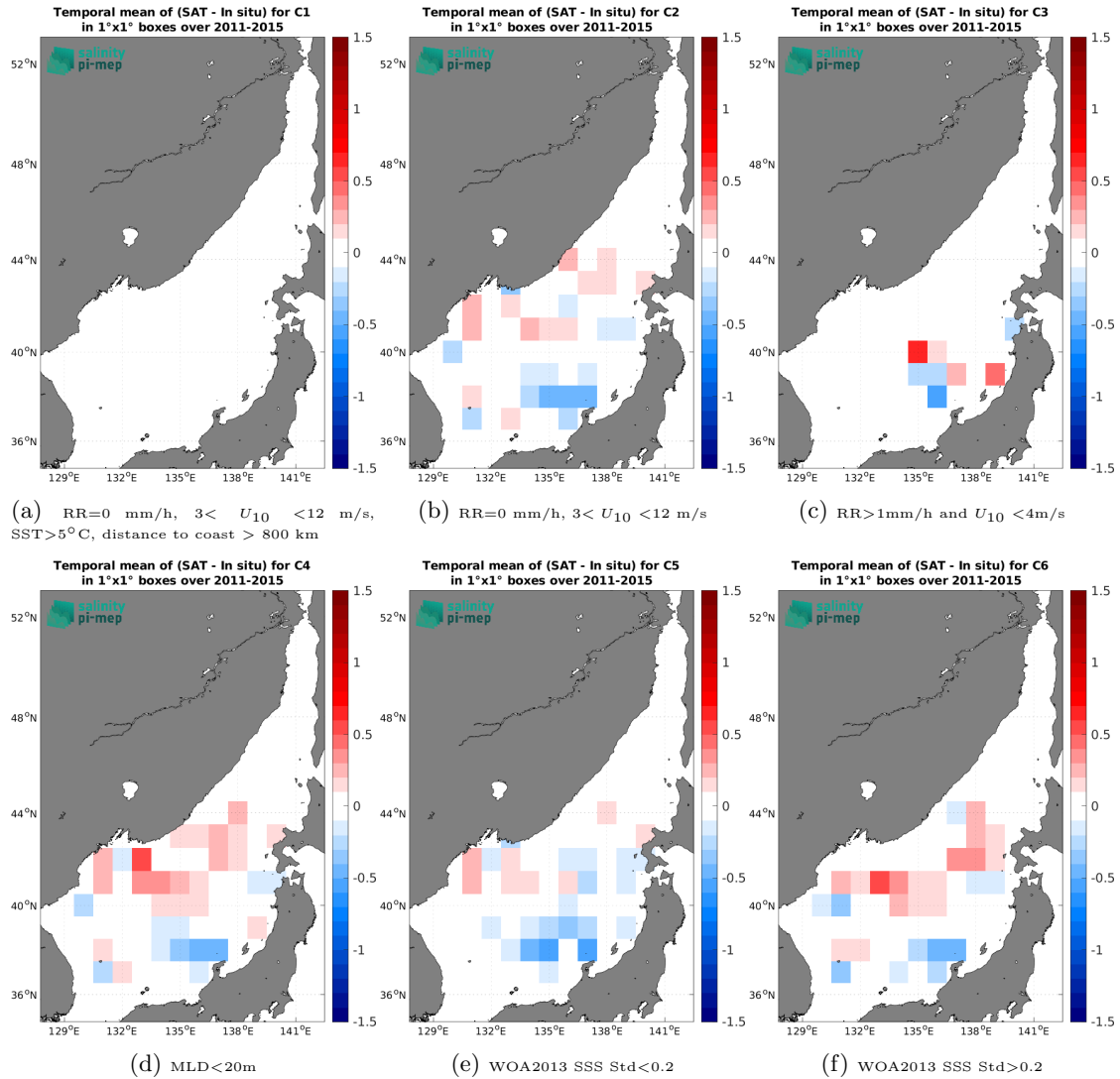
Figure 14: Temporal mean gridded over spatial boxes of size 1^\circ \times 1^\circ of \Delta SSS (Aquarius SSS L4 OI v5 - Monthly (IPRC) - Argo) for 6 different subdatasets corresponding to:RR=0 mm/h, 3 < U_{10} < 12 m/s, SST>5°C, distance to coast > 800 km (a), RR=0 mm/h, 3 < U_{10} < 12 m/s (b), RR>1mm/h and U_{10} < 4 m/s (c),MLD<20m (d),WOA2013 SSS Std<0.2 (e),WOA2013 SSS Std>0.2 (f).
