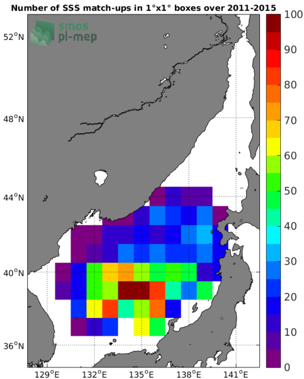
Figure 4: Number of SSS match-ups between Argo SSS and the Aquarius-L4-IPRC-V5-MONTHLY SSS product for the Sea of Japan Pi-MEP region over 1°x1° boxes and for the full satellite product period.
