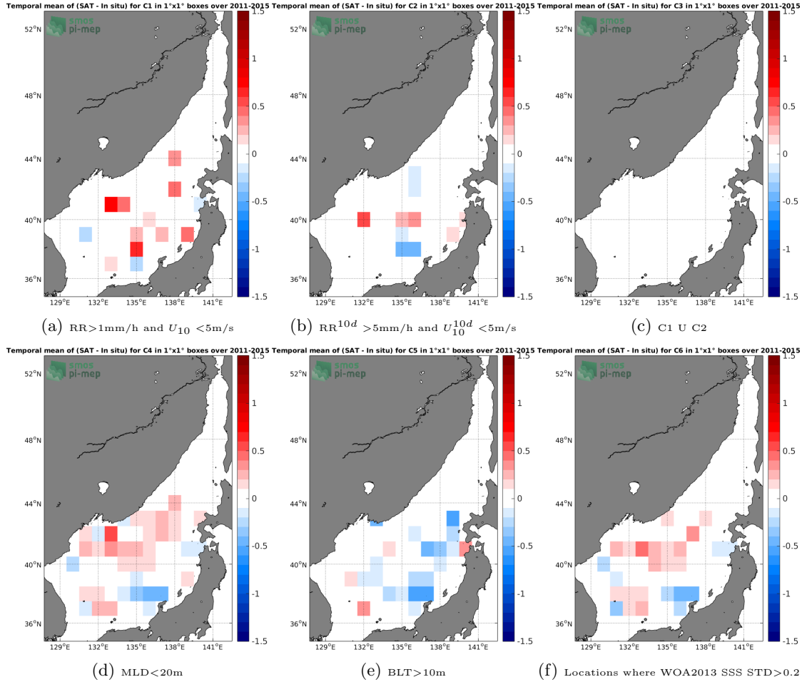
Figure 12: Temporal mean gridded over spatial boxes of size 1°x1° of \Delta SSS (Aquarius-L4-IPRC-V5-MONTHLY - Argo) for 6 different subdatasets corresponding to:RR>1mm/h and U_{10} < 5\text{m/s} (a), RR^{10d} > 5\text{mm/h} and U_{10}^{10d} < 5\text{m/s} (b), C1 U C2 (c),MLD<20m (d),BLT>10m (e),Locations where WOA2013 SSS STD>0.2 (f).
