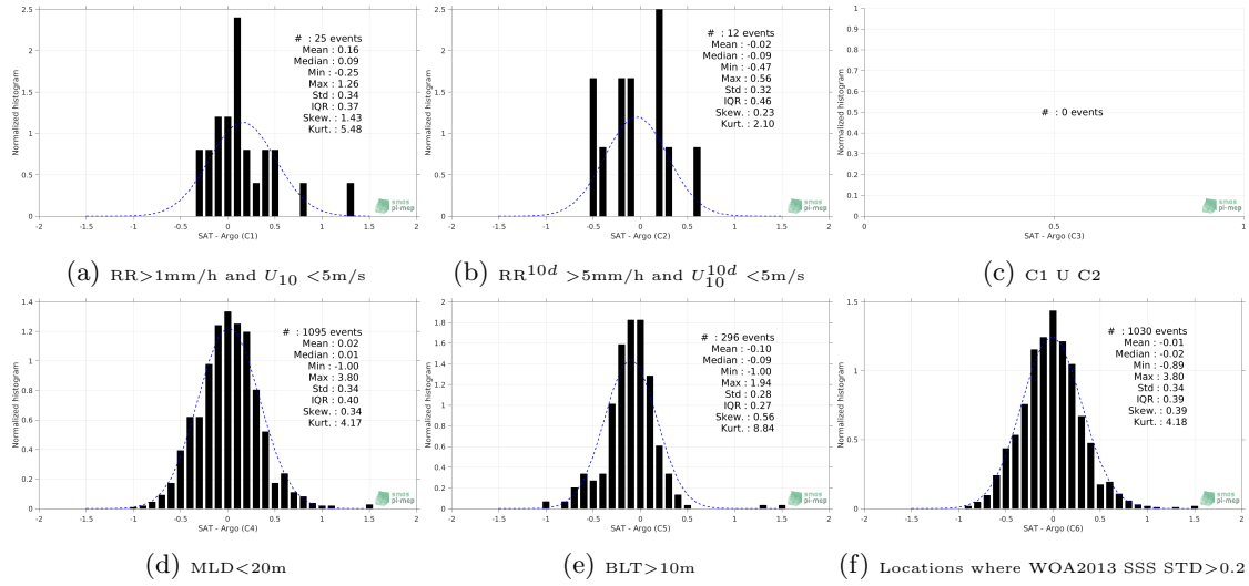
Figure 13: Normalized histogram of \Delta SSS (Aquarius-L4-IPRC-V5-MONTHLY - Argo) for 6 different subdatasets corresponding to: RR > 1mm/h and U_{10} < 5\text{m/s} (a), RR 10d > 5mm/h and U_{10}^{10d} < 5\text{m/s} (b), C1 U C2 (c), MLD < 20m (d), BLT > 10m (e), Locations where WOA2013 SSS STD > 0.2 (f).
