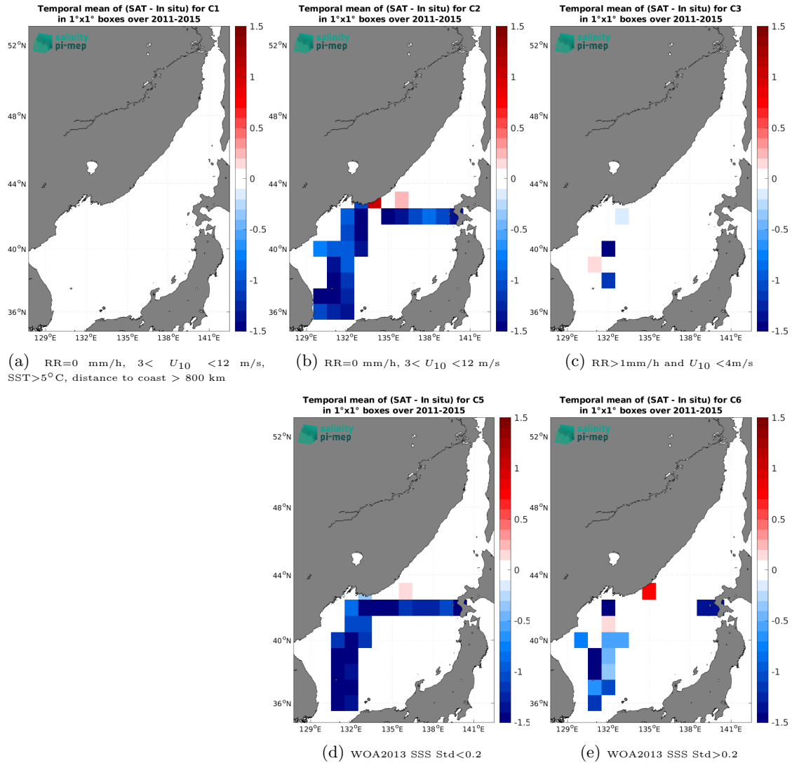
Figure 14: Temporal mean gridded over spatial boxes of size 1^\circ \times 1^\circ of \Delta\text{SSS} (Aquarius SSS L3 OR v5 - 7-Day running (NASA-GSFC) - TSG (LEGOS-DM)) for 5 different subdatasets corresponding to: RR=0 mm/h, 3 < U_{10} < 12 m/s, SST > 5^\circ\text{C} , distance to coast > 800 km (a), RR=0 mm/h, 3 < U_{10} < 12 m/s (b), RR > 1 mm/h and U_{10} < 4 m/s (c), WOA2013 SSS Std < 0.2 (d), WOA2013 SSS Std > 0.2 (e).
