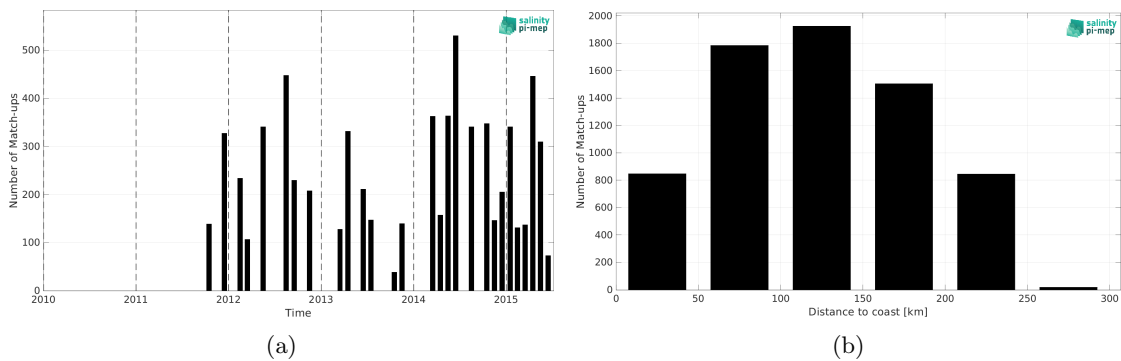
Figure 2: Number of match-ups between TSG (LEGOS-DM) and Aquarius SSS L3 OR v5 - 7-Day running (NASA-GSFC) SSS as a function of time (a) and as function of the distance to coast (b) over the Sea of Japan Pi-MEP region and for the full satellite product period.
