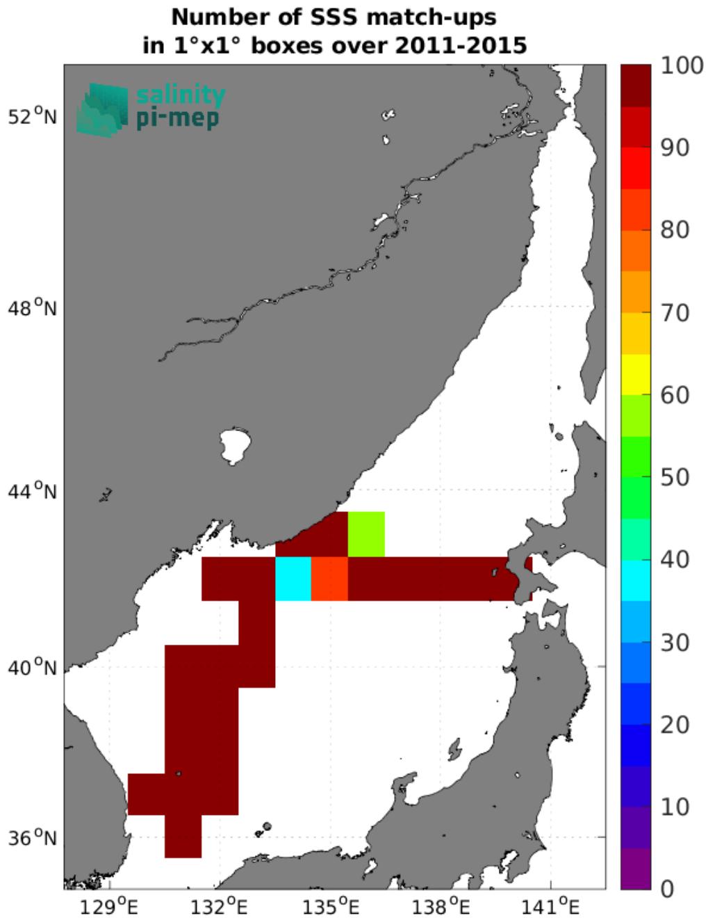
Figure 5: Number of SSS match-ups between TSG (LEGOS-DM) SSS and the Aquarius SSS L3 OR v5 - 7-Day running (NASA-GSFC) SSS product for the Sea of Japan Pi-MEP region over 1°x1° boxes and for the full satellite product period.
