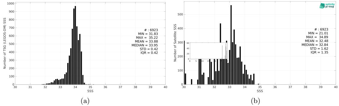
Figure 3: Histograms of SSS from TSG (LEGOS-DM) (a) and Aquarius SSS L3 OR v5 - 7-Day running (NASA-GSFC) (b) considering all match-up pairs per bins of 0.1 over the Sea of Japan Pi-MEP region and for the full satellite product period.
