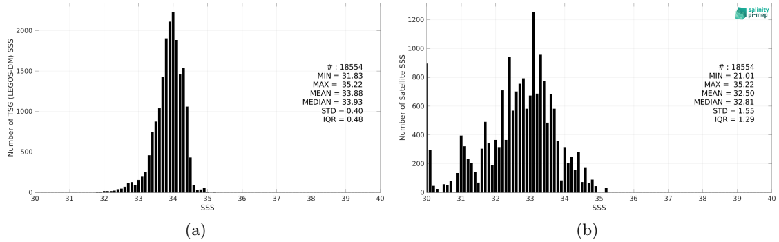
Figure 2: Histograms of SSS from TSG (LEGOS-DM) (a) and Aquarius SSS L3 OR v5 - 7-Day running (NASA-GSFC) (b) considering all match-up pairs per bins of 0.1 over the Sea of Japan Pi-MEP region and for the full satellite product period.
