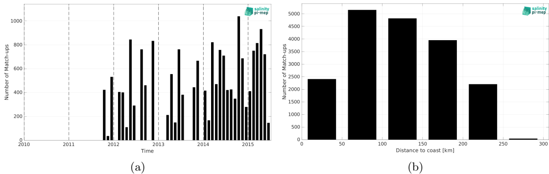
Figure 1: Number of match-ups between TSG (LEGOS-DM) and Aquarius SSS L3 OR v5 - 7-Day running (NASA-GSFC) SSS as a function of time (a) and as function of the distance to coast (b) over the Sea of Japan Pi-MEP region and for the full satellite product period.
