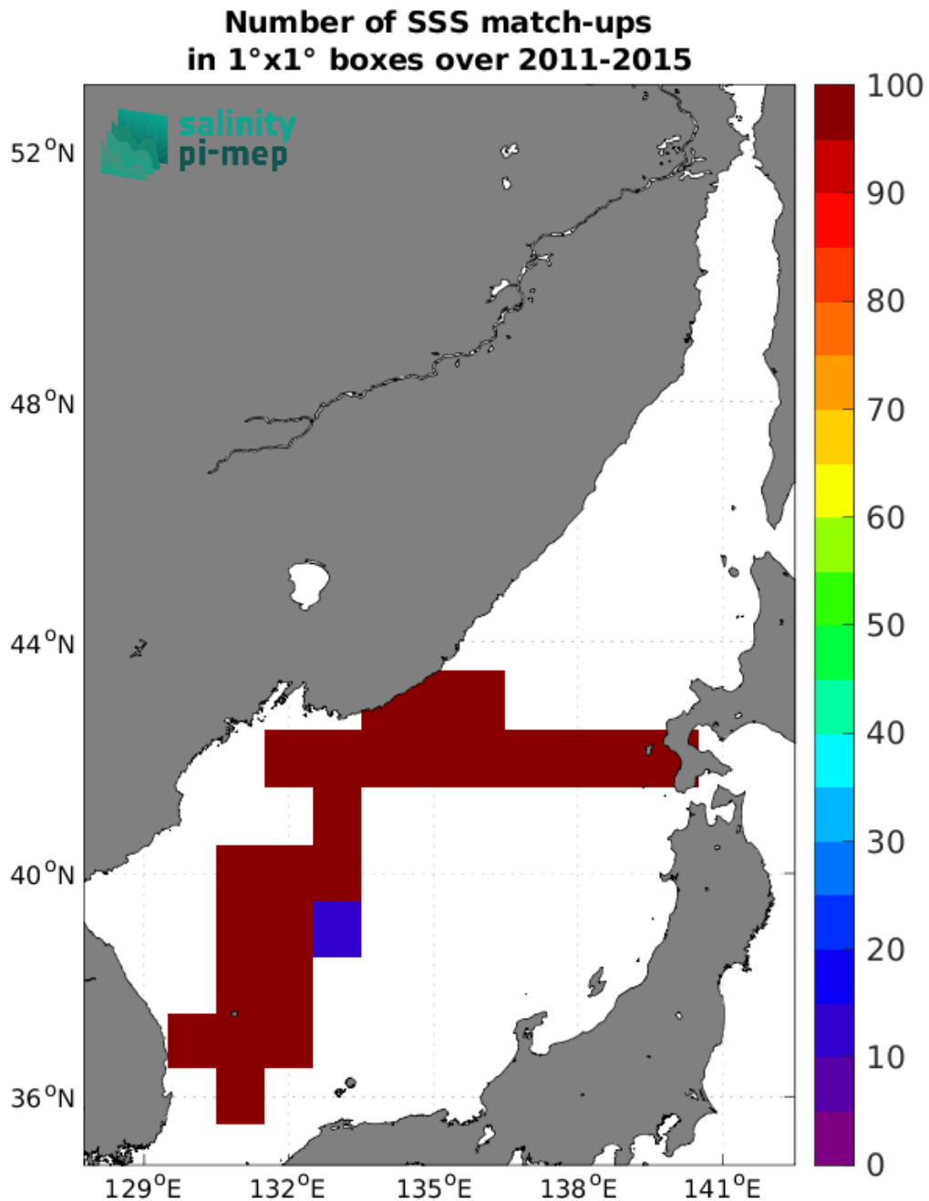
Figure 4: Number of SSS match-ups between TSG (LEGOS-DM) SSS and the Aquarius SSS L3 OR v5 - 7-Day running (NASA-GSFC) SSS product for the Sea of Japan Pi-MEP region over 1°x1° boxes and for the full satellite product period.
