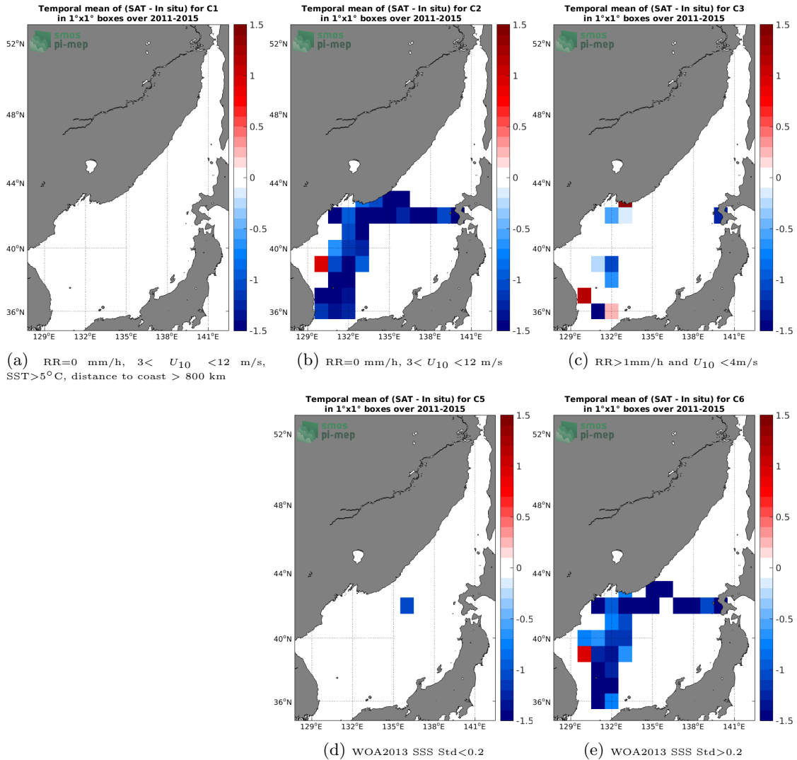
Figure 12: Temporal mean gridded over spatial boxes of size 1^\circ \times 1^\circ of \Delta SSS (Aquarius SSS L3 OR v5 - 7-Day running (NASA-GSFC) - TSG (LEGOS-DM)) for 5 different subdatasets corresponding to:RR=0 mm/h, 3 < U_{10} < 12 m/s, SST>5°C, distance to coast > 800 km (a), RR=0 mm/h, 3 < U_{10} < 12 m/s (b), RR>1mm/h and U_{10} < 4 m/s (c), WOA2013 SSS Std<0.2 (d), WOA2013 SSS Std>0.2 (e).
