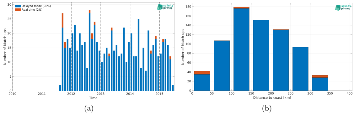
Figure 2: Number of match-ups between Argo and Aquarius SSS L3 OR v5 - 7-Day running (NASA-GSFC) SSS as a function of time (a) and as function of the distance to coast (b) over the Sea of Japan Pi-MEP region and for the full satellite product period.
