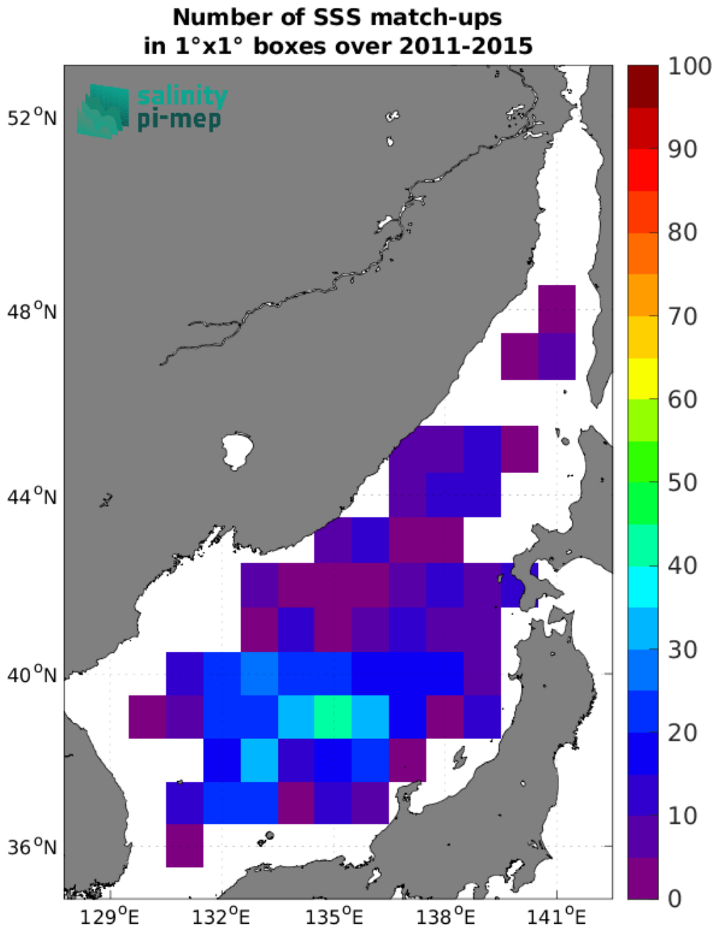
Figure 5: Number of SSS match-ups between Argo SSS and the Aquarius SSS L3 OR v5 - 7-Day running (NASA-GSFC) SSS product for the Sea of Japan Pi-MEP region over 1°x1° boxes and for the full satellite product period.
