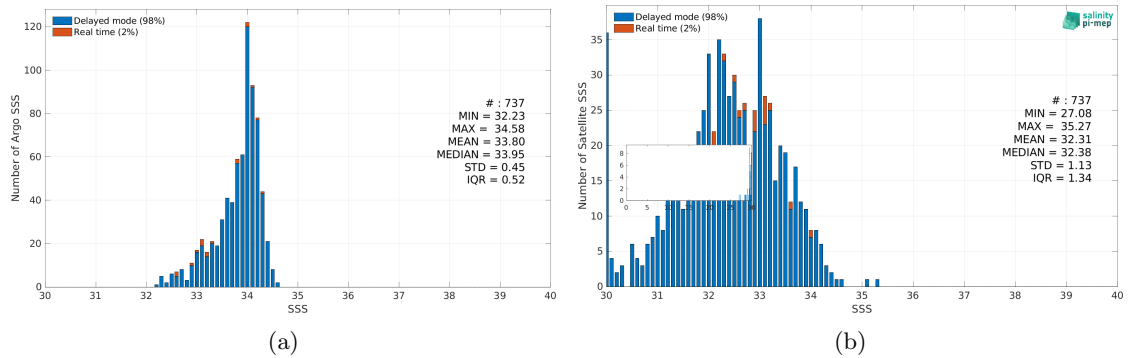
Figure 3: Histograms of SSS from Argo (a) and Aquarius SSS L3 OR v5 - 7-Day running (NASA-GSFC) (b) considering all match-up pairs per bins of 0.1 over the Sea of Japan Pi-MEP region and for the full satellite product period.
