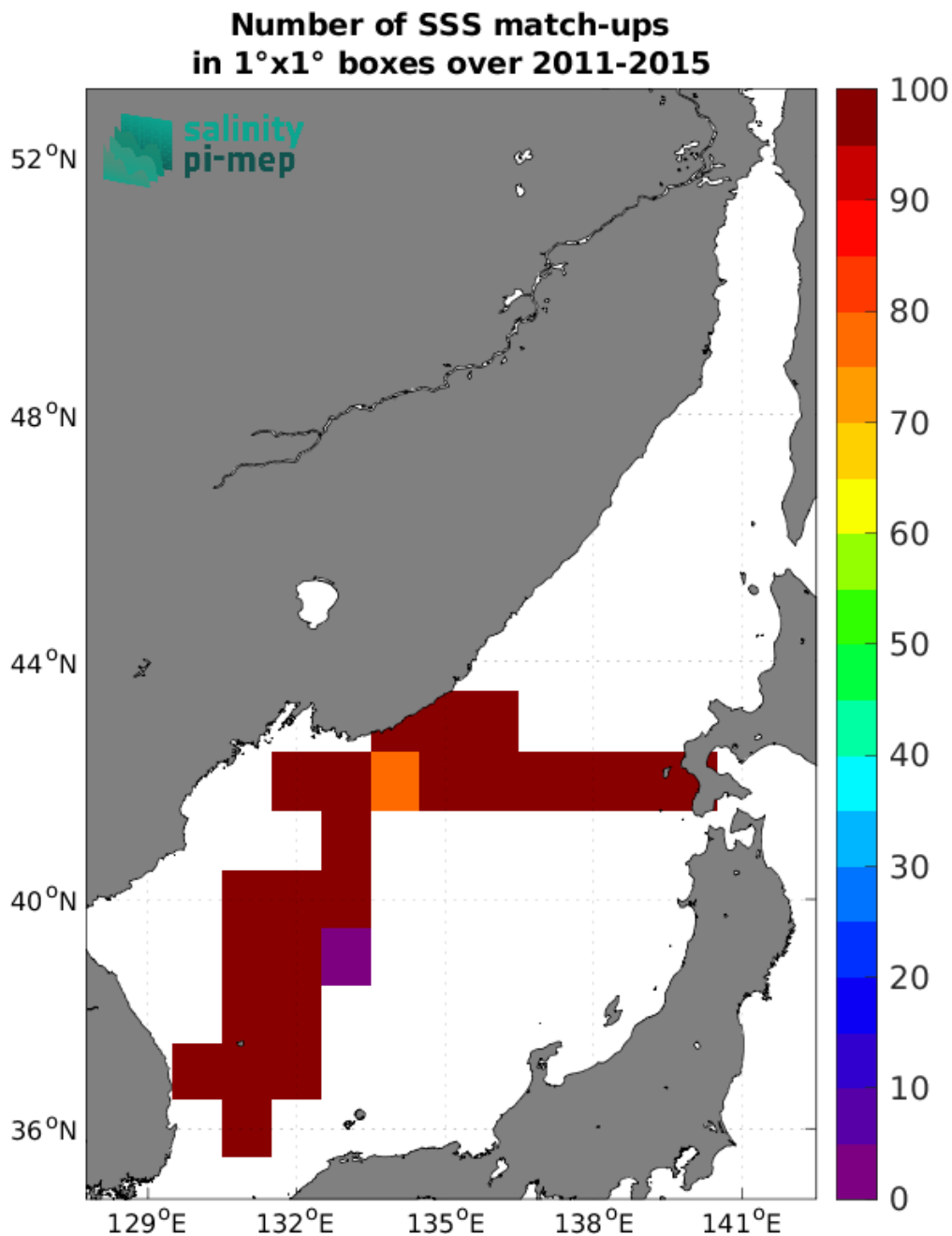
Figure 5: Number of SSS match-ups between TSG (LEGOS-DM) SSS and the Aquarius SSS L3 OR v5 - 7-Day running - Rain mask (NASA-GSFC) SSS product for the Sea of Japan Pi-MEP region over 1°x1° boxes and for the full satellite product period.
