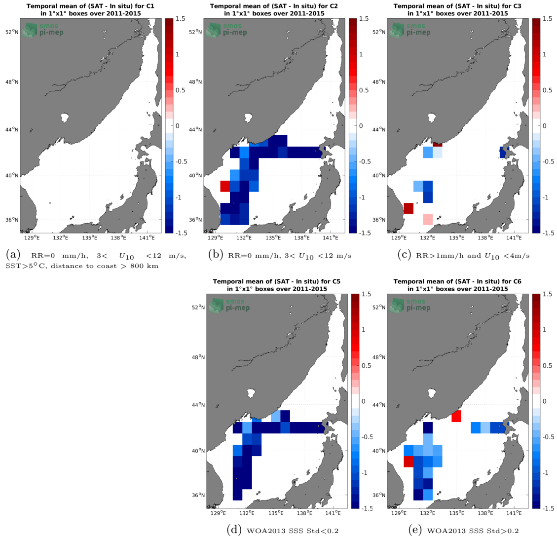
Figure 12: Temporal mean gridded over spatial boxes of size 1^\circ \times 1^\circ of \Delta SSS (Aquarius SSS L3 OR v5 - 7-Day running - Rain mask (NASA-GSFC) - TSG (LEGOS-DM)) for 5 different subdatasets corresponding to:RR=0 mm/h, 3 < U_{10} < 12 m/s, SST>5°C, distance to coast > 800 km (a), RR=0 mm/h, 3 < U_{10} < 12 m/s (b), RR>1mm/h and U_{10} < 4 m/s (c), WOA2013 SSS Std<0.2 (d), WOA2013 SSS Std>0.2 (e).
