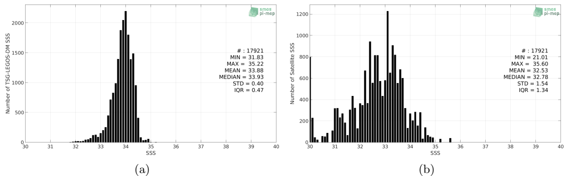
Figure 2: Histograms of SSS from TSG-LEGOS-DM (a) and Aquarius-L3-OR-V5-7DAY-RUNNING-RAIN-MASK-1DEG (b) considering all match-up pairs per bins of 0.1 over the Sea of Japan Pi-MEP region and for the full satellite product period.
