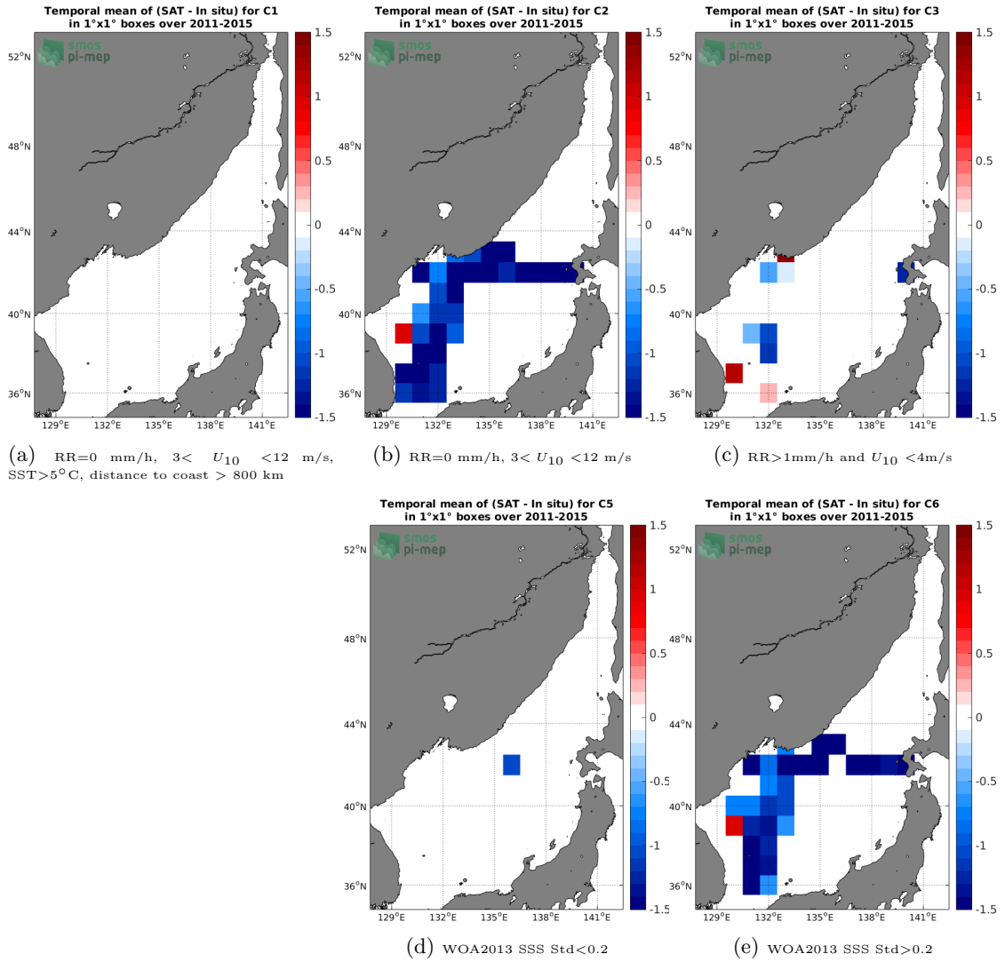
Figure 12: Temporal mean gridded over spatial boxes of size 1°x1° of \Delta SSS (Aquarius-L3-OR-V5-7DAY-RUNNING-RAIN-MASK-1DEG - TSG-LEGOS-DM) for 5 different subdatasets corresponding to:RR=0 mm/h, 3 < U_{10} < 12 m/s, SST > 5°C, distance to coast > 800 km (a), RR=0 mm/h, 3 < U_{10} < 12 m/s (b), RR > 1mm/h and U_{10} < 4 m/s (c), WOA2013 SSS Std < 0.2 (d), WOA2013 SSS Std > 0.2 (e).
