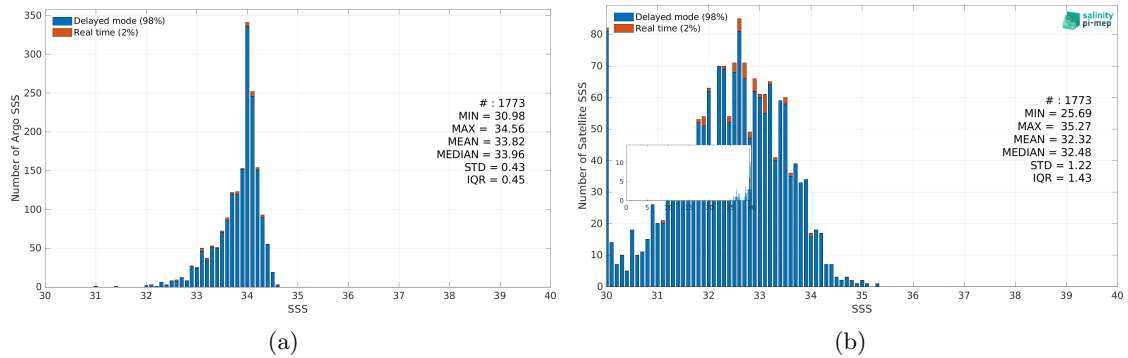
Figure 3: Histograms of SSS from Argo (a) and Aquarius SSS L3 OR v5 - 7-Day running - Rain mask (NASA-GSFC) (b) considering all match-up pairs per bins of 0.1 over the Sea of Japan Pi-MEP region and for the full satellite product period.
