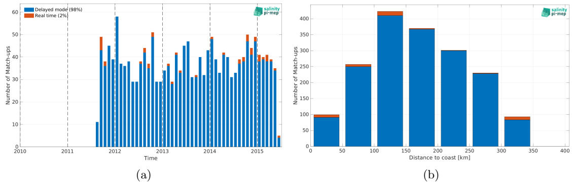
Figure 2: Number of match-ups between Argo and Aquarius SSS L3 OR v5 - 7-Day running - Rain mask (NASA-GSFC) SSS as a function of time (a) and as function of the distance to coast (b) over the Sea of Japan Pi-MEP region and for the full satellite product period.
