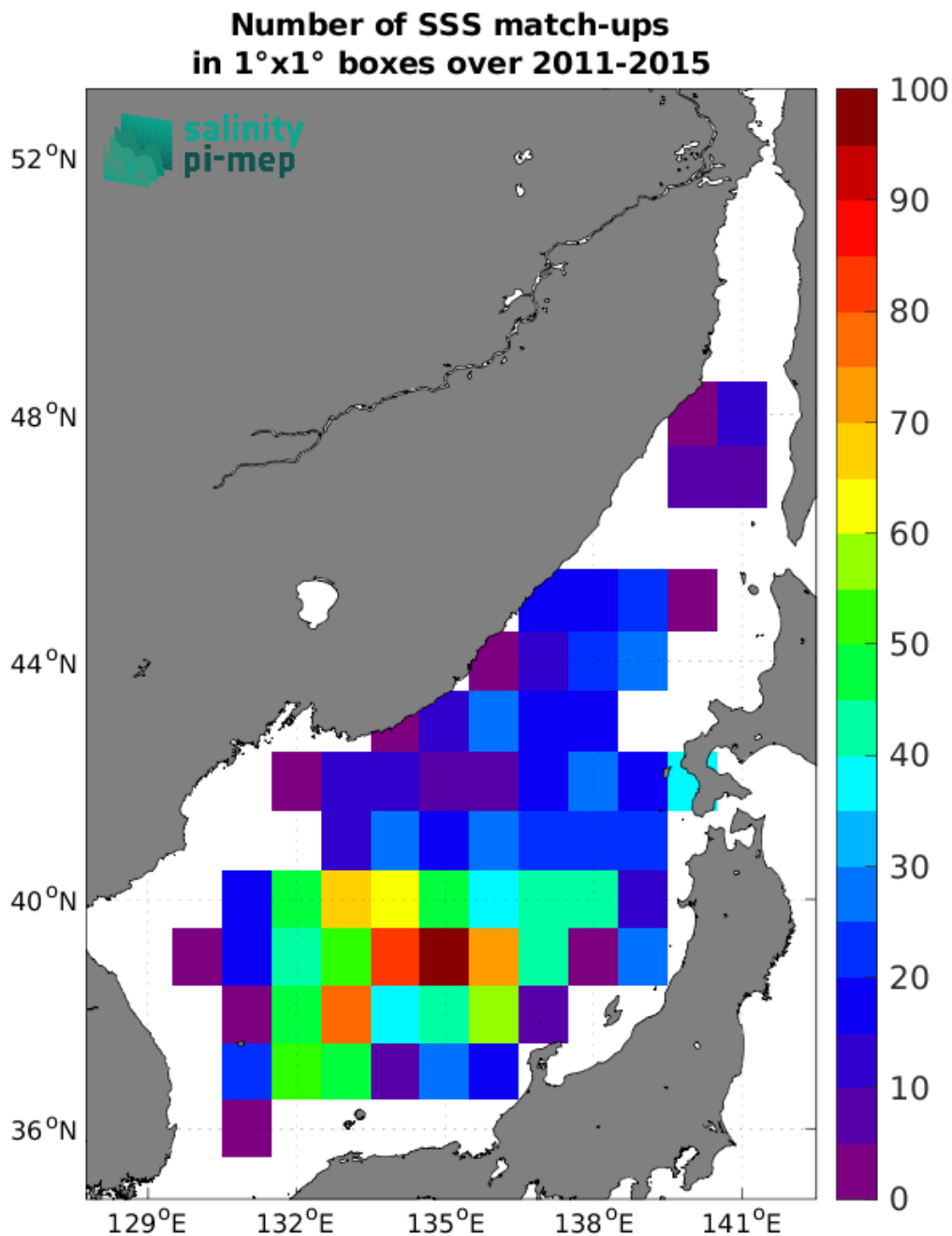
Figure 5: Number of SSS match-ups between Argo SSS and the Aquarius SSS L3 OR v5 - 7-Day running - Rain mask (NASA-GSFC) SSS product for the Sea of Japan Pi-MEP region over 1°x1° boxes and for the full satellite product period.
