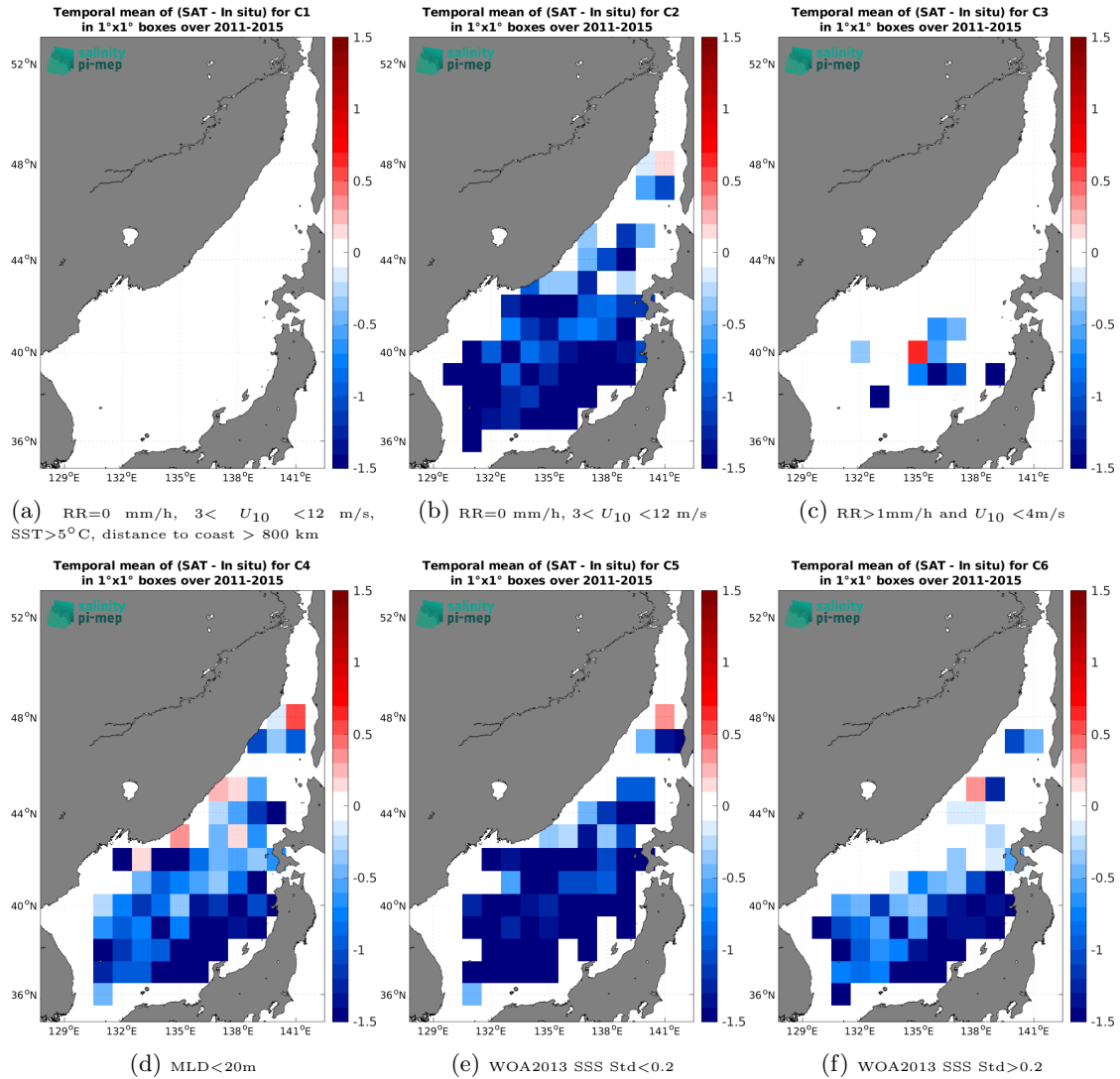
Figure 14: Temporal mean gridded over spatial boxes of size 1^\circ \times 1^\circ of \Delta SSS (Aquarius SSS L3 OR v5 - 7-Day running - Rain mask (NASA-GSFC) - Argo) for 6 different subdatasets corresponding to:RR=0 mm/h, 3 < U_{10} < 12 m/s, SST>5°C, distance to coast > 800 km (a), RR=0 mm/h, 3 < U_{10} < 12 m/s (b), RR>1mm/h and U_{10} < 4 m/s (c),MLD<20m (d),WOA2013 SSS Std<0.2 (e),WOA2013 SSS Std>0.2 (f).
