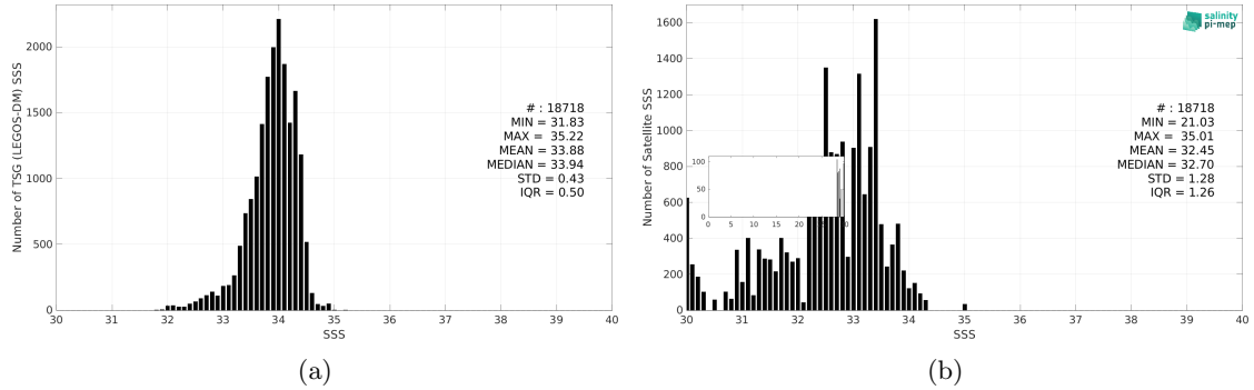
Figure 3: Histograms of SSS from TSG (LEGOS-DM) (a) and Aquarius SSS L3 OR v5 - Monthly (NASA-GSFC) (b) considering all match-up pairs per bins of 0.1 over the Sea of Japan Pi-MEP region and for the full satellite product period.
