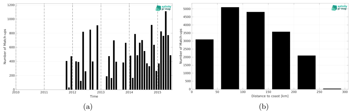
Figure 2: Number of match-ups between TSG (LEGOS-DM) and Aquarius SSS L3 OR v5 - Monthly (NASA-GSFC) SSS as a function of time (a) and as function of the distance to coast (b) over the Sea of Japan Pi-MEP region and for the full satellite product period.
