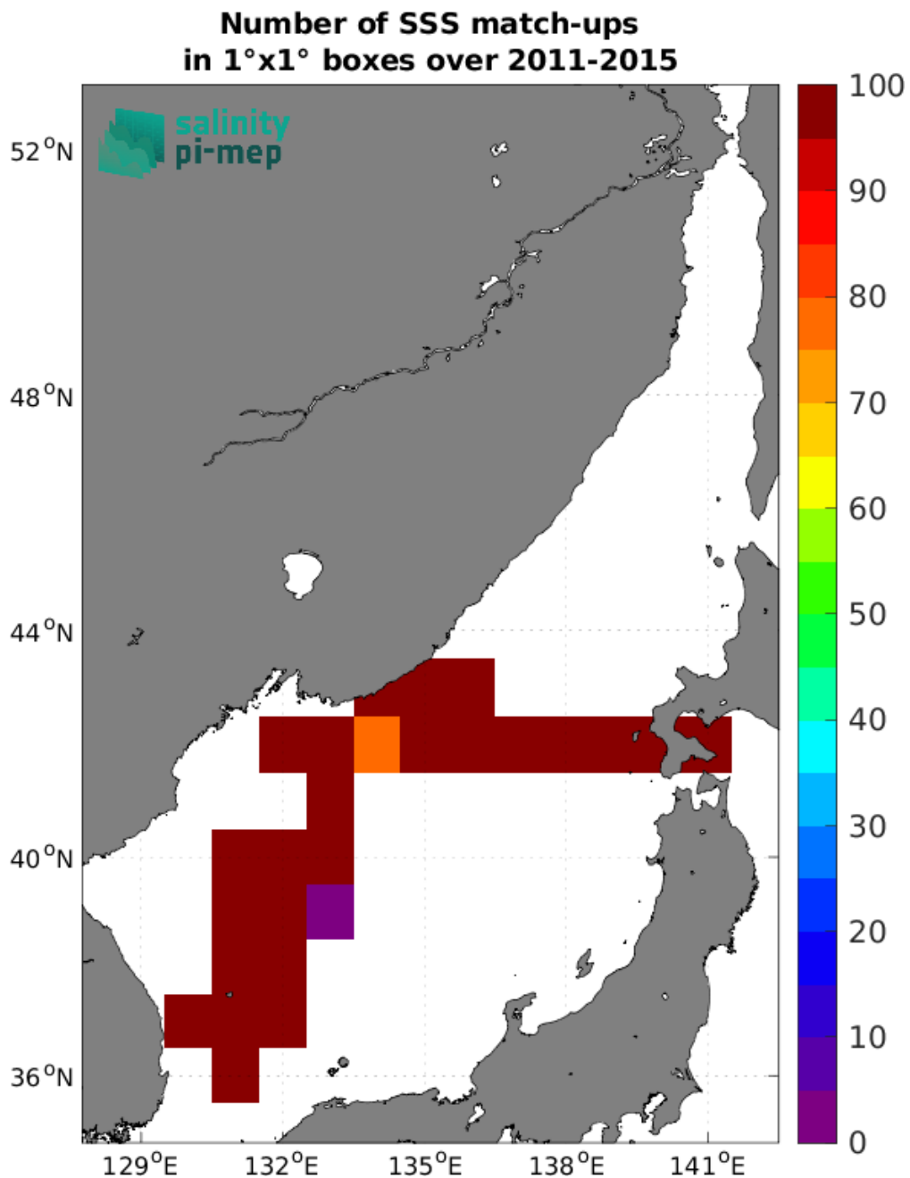
Figure 5: Number of SSS match-ups between TSG (LEGOS-DM) SSS and the Aquarius SSS L3 OR v5 - Monthly (NASA-GSFC) SSS product for the Sea of Japan Pi-MEP region over 1°x1° boxes and for the full satellite product period.
