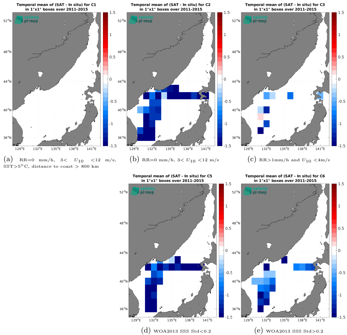
Figure 14: Temporal mean gridded over spatial boxes of size 1^\circ \times 1^\circ of \Delta SSS (Aquarius SSS L3 OR v5 - Monthly (NASA-GSFC) - TSG (LEGOS-DM)) for 5 different subdatasets corresponding to:RR=0 mm/h, 3 < U_{10} < 12 m/s, SST>5°C, distance to coast > 800 km (a), RR=0 mm/h, 3 < U_{10} < 12 m/s (b), RR>1mm/h and U_{10} < 4 m/s (c), WOA2013 SSS Std<0.2 (d), WOA2013 SSS Std>0.2 (e).
