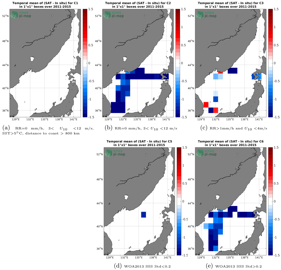
Figure 12: Temporal mean gridded over spatial boxes of size 1^\circ \times 1^\circ of \Delta\text{SSS} (Aquarius-L3-OR-V5-MONTHLY-1DEG - TSG-LEGOS-DM) for 5 different subdatasets corresponding to: RR=0 mm/h, 3 < U_{10} < 12 m/s, SST > 5^\circ\text{C} , distance to coast > 800 km (a), RR=0 mm/h, 3 < U_{10} < 12 m/s (b), RR > 1\text{mm/h} and U_{10} < 4\text{m/s} (c), WOA2013 SSS Std < 0.2 (d), WOA2013 SSS Std > 0.2 (e).
