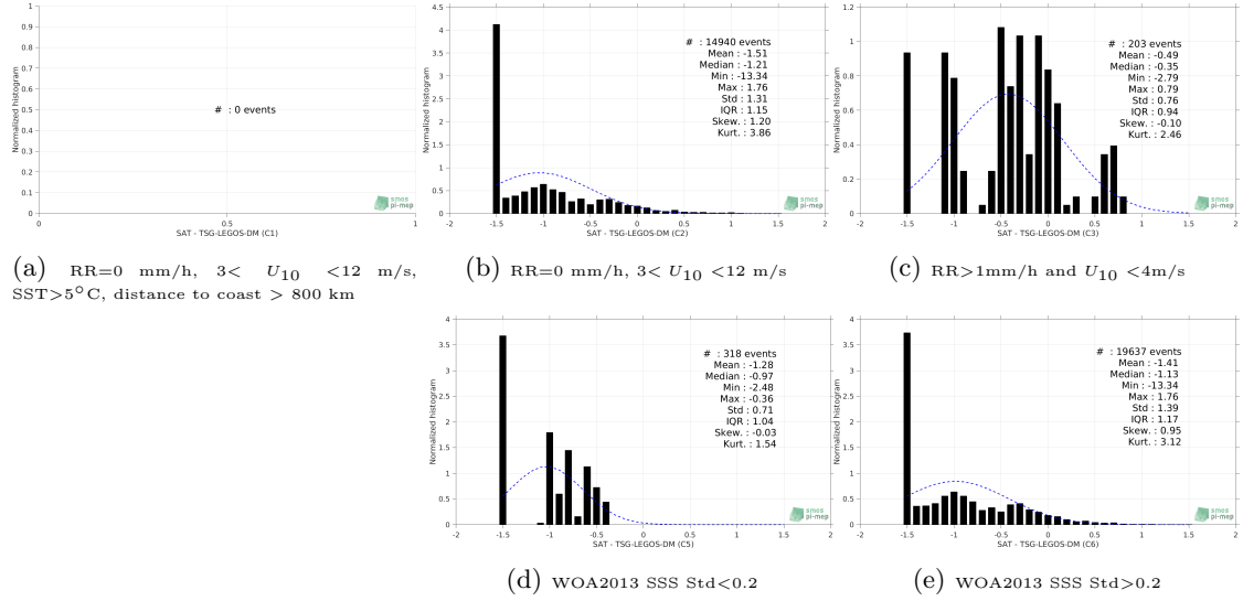
Figure 13: Normalized histogram of \Delta SSS (Aquarius-L3-OR-V5-MONTHLY-1DEG - TSG-LEGOS-DM) for 5 different subdatasets corresponding to: RR=0 mm/h, 3 < U_{10} < 12 m/s, SST > 5°C, distance to coast > 800 km (a), RR=0 mm/h, 3 < U_{10} < 12 m/s (b), RR > 1mm/h and U_{10} < 4 m/s (c), WOA2013 SSS Std < 0.2 (d), WOA2013 SSS Std > 0.2 (e).
