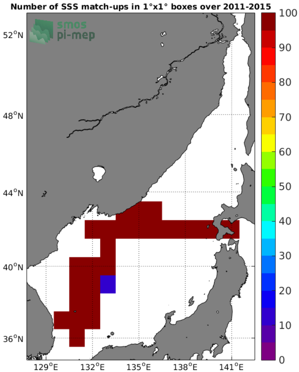
Figure 4: Number of SSS match-ups between TSG-LEGOS-DM SSS and the Aquarius-L3-OR-V5-MONTHLY-1DEG SSS product for the Sea of Japan Pi-MEP region over 1°x1° boxes and for the full satellite product period.
