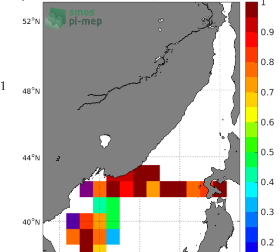
Temporal STD of (Sat-TSG-LEGOS-DM) in 1°x1° boxes over 2011-2015
