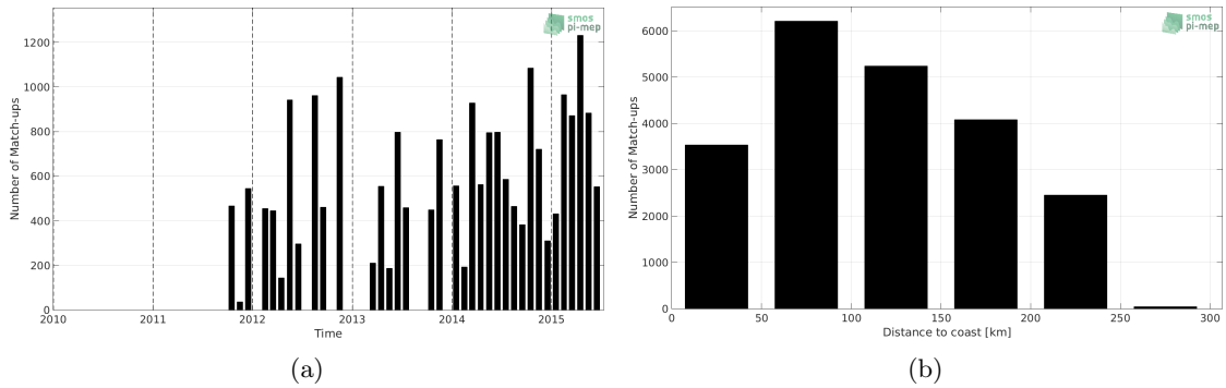
Figure 1: Number of match-ups between TSG-LEGOS-DM and Aquarius-L3-OR-V5-MONTHLY-1DEG SSS as a function of time (a) and as function of the distance to coast (b) over the Sea of Japan Pi-MEP region and for the full satellite product period.
