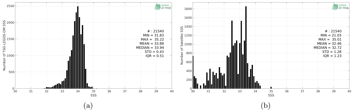
Figure 2: Histograms of SSS from TSG-LEGOS-DM (a) and Aquarius-L3-OR-V5-MONTHLY-1DEG (b) considering all match-up pairs per bins of 0.1 over the Sea of Japan Pi-MEP region and for the full satellite product period.
