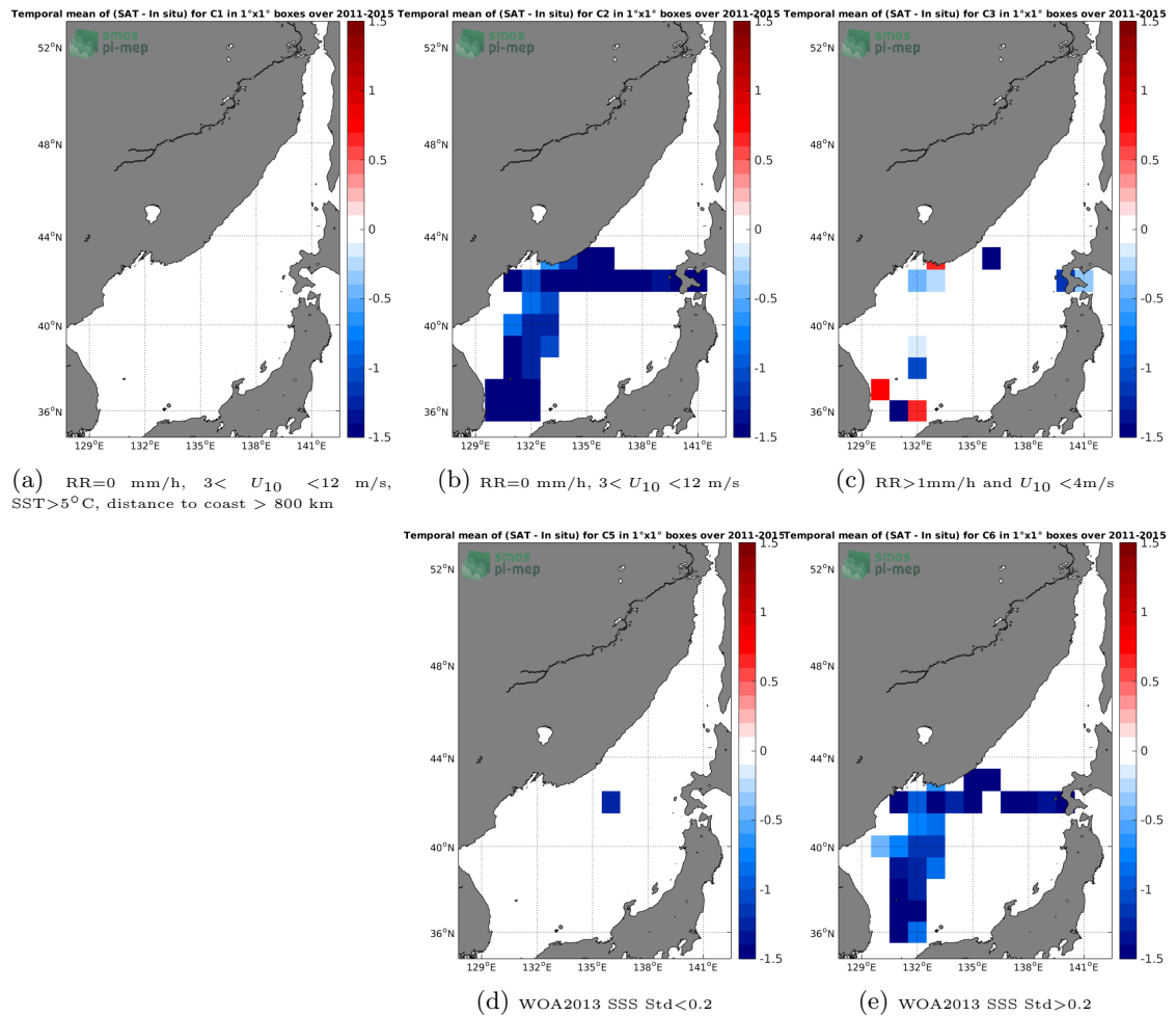
Figure 12: Temporal mean gridded over spatial boxes of size 1^\circ \times 1^\circ of \Delta SSS (Aquarius-L3-OR-V5-MONTHLY-1DEG - TSG-LEGOS-DM) for 5 different subdatasets corresponding to: RR=0 mm/h, 3 < U_{10} < 12 m/s, SST > 5^\circ C , distance to coast > 800 km (a), RR=0 mm/h, 3 < U_{10} < 12 m/s (b), RR > 1 mm/h and U_{10} < 4 m/s (c), WOA2013 SSS Std < 0.2 (d), WOA2013 SSS Std > 0.2 (e).
