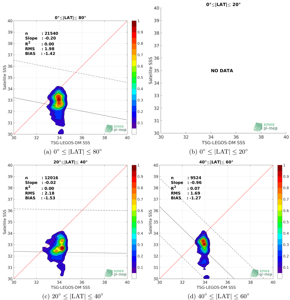
Figure 9: Contour maps of the concentration of Aquarius-L3-OR-V5-MONTHLY-1DEG SSS (y-axis) versus TSG-LEGOS-DM SSS (x-axis) at match-up pairs for different latitudinal bands. For each plot, the red line shows x=y . The black thin and dashed lines indicate a linear fit through the data cloud and the \pm 95\% confidence levels, respectively. The number match-up pairs n , the slope and R^2 coefficient of the linear fit, the root mean square (RMS) and the mean bias between satellite and in situ data are indicated for each latitude band in each plots.
