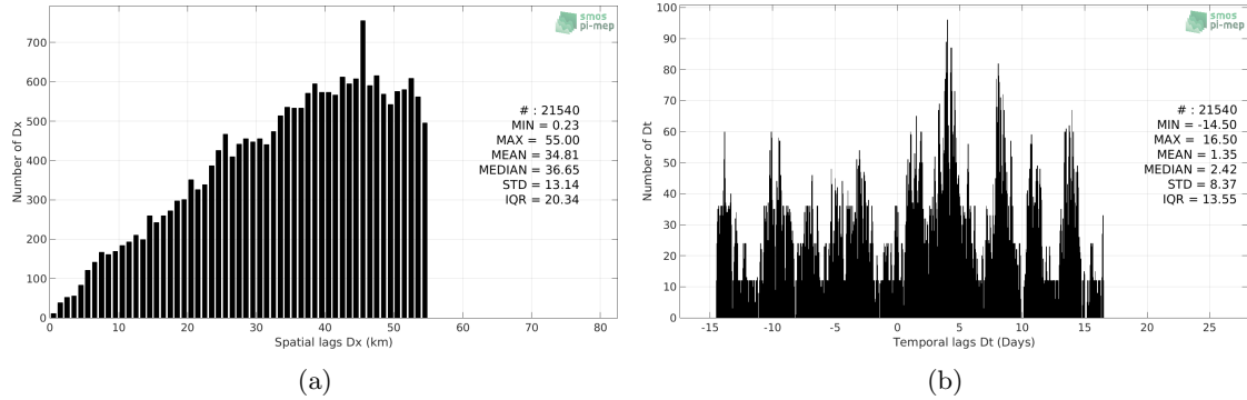
Figure 5: Histograms of the spatial (a) and temporal (b) lags between the time of the TSG-LEGOS-DM measurements and the date of the corresponding Aquarius-L3-OR-V5-MONTHLY-1DEG SSS product.
