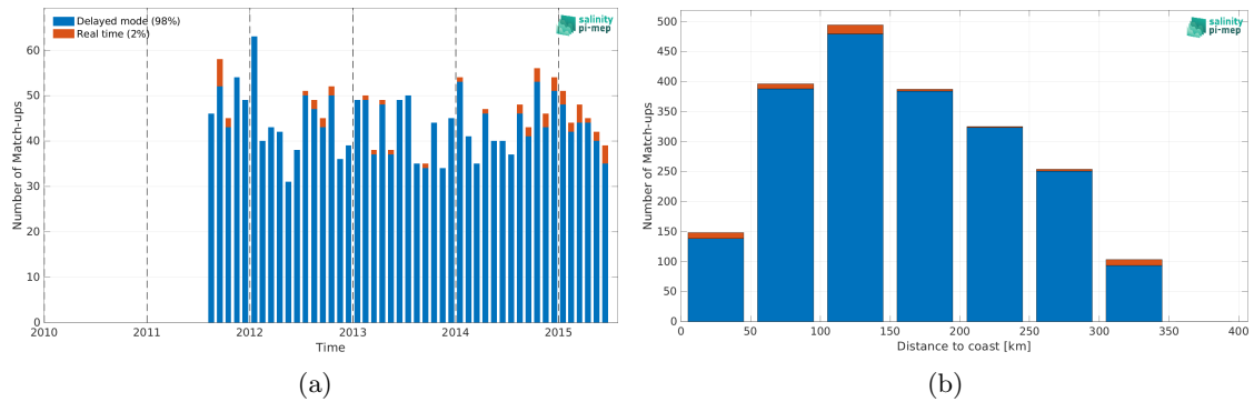
Figure 2: Number of match-ups between Argo and Aquarius SSS L3 OR v5 - Monthly (NASA-GSFC) SSS as a function of time (a) and as function of the distance to coast (b) over the Sea of Japan Pi-MEP region and for the full satellite product period.
