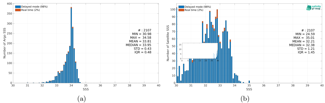
Figure 3: Histograms of SSS from Argo (a) and Aquarius SSS L3 OR v5 - Monthly (NASA-GSFC) (b) considering all match-up pairs per bins of 0.1 over the Sea of Japan Pi-MEP region and for the full satellite product period.
