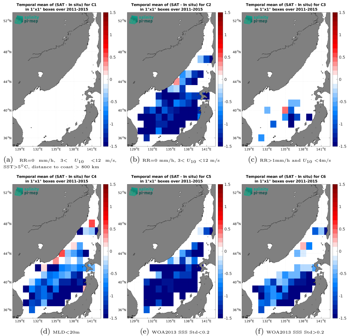
Figure 14: Temporal mean gridded over spatial boxes of size 1^\circ \times 1^\circ of \Delta SSS (Aquarius SSS L3 OR v5 - Monthly (NASA-GSFC) - Argo) for 6 different subdatasets corresponding to:RR=0 mm/h, 3 < U_{10} < 12 m/s, SST>5°C, distance to coast > 800 km (a), RR=0 mm/h, 3 < U_{10} < 12 m/s (b), RR>1mm/h and U_{10} < 4 m/s (c),MLD<20m (d),WOA2013 SSS Std<0.2 (e),WOA2013 SSS Std>0.2 (f).
