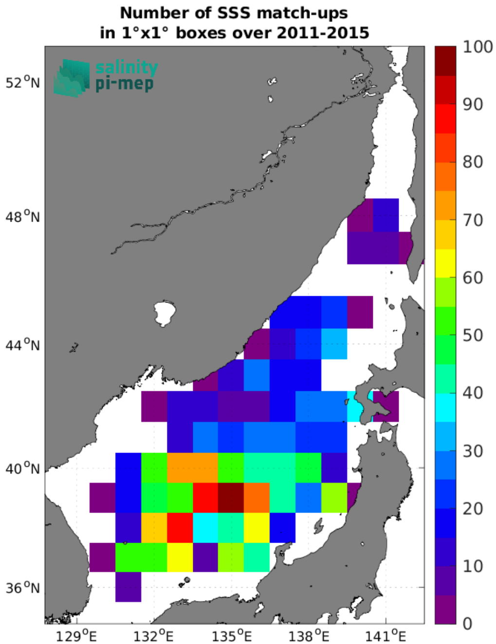
Figure 5: Number of SSS match-ups between Argo SSS and the Aquarius SSS L3 OR v5 - Monthly (NASA-GSFC) SSS product for the Sea of Japan Pi-MEP region over 1°x1° boxes and for the full satellite product period.
