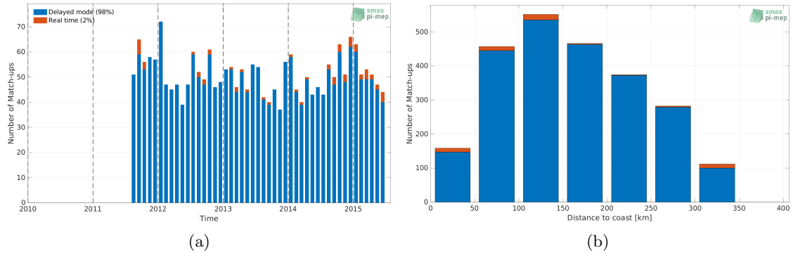
Figure 1: Number of match-ups between Argo and Aquarius SSS L3 OR v5 - Monthly (NASA-GSFC) SSS as a function of time (a) and as function of the distance to coast (b) over the Sea of Japan Pi-MEP region and for the full satellite product period.
