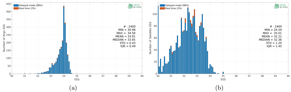
Figure 2: Histograms of SSS from Argo (a) and Aquarius SSS L3 OR v5 - Monthly (NASA-GSFC) (b) considering all match-up pairs per bins of 0.1 over the Sea of Japan Pi-MEP region and for the full satellite product period.
