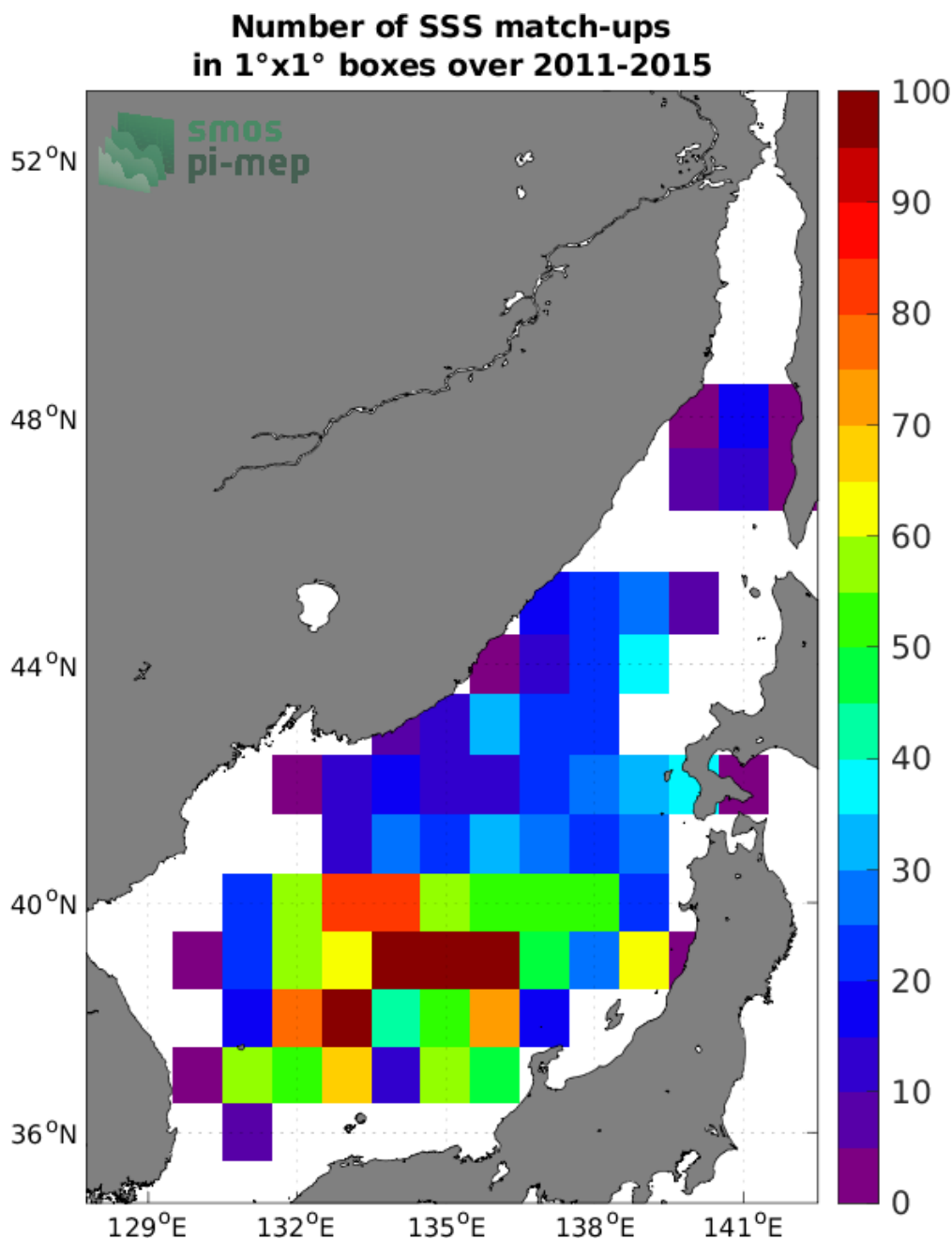
Figure 4: Number of SSS match-ups between Argo SSS and the Aquarius SSS L3 OR v5 - Monthly (NASA-GSFC) SSS product for the Sea of Japan Pi-MEP region over 1°x1° boxes and for the full satellite product period.
