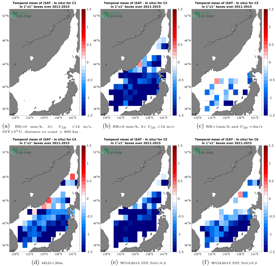
Figure 12: Temporal mean gridded over spatial boxes of size 1^\circ \times 1^\circ of \Delta SSS (Aquarius SSS L3 OR v5 - Monthly (NASA-GSFC) - Argo) for 6 different subdatasets corresponding to: RR=0 mm/h, 3 < U_{10} < 12 m/s, SST > 5^\circ\text{C} , distance to coast > 800 km (a), RR=0 mm/h, 3 < U_{10} < 12 m/s (b), RR > 1 mm/h and U_{10} < 4 m/s (c), MLD < 20 m (d), WOA2013 SSS Std < 0.2 (e), WOA2013 SSS Std > 0.2 (f).
