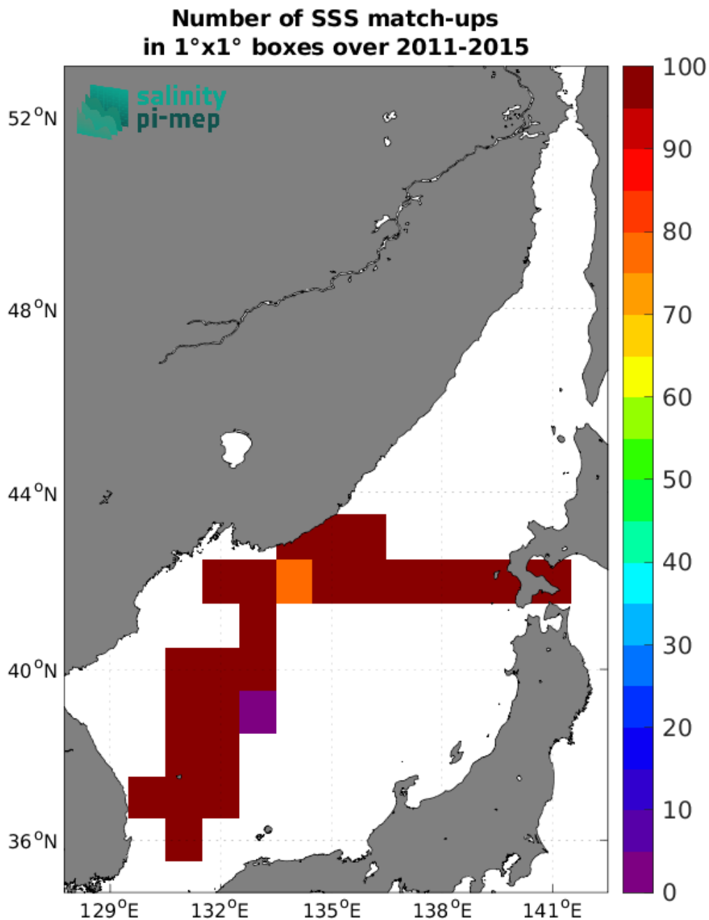
Figure 5: Number of SSS match-ups between TSG (LEGOS-DM) SSS and the Aquarius SSS L3 OR v5 - Monthly - Rain mask (NASA-GSFC) SSS product for the Sea of Japan Pi-MEP region over 1°x1° boxes and for the full satellite product period.
