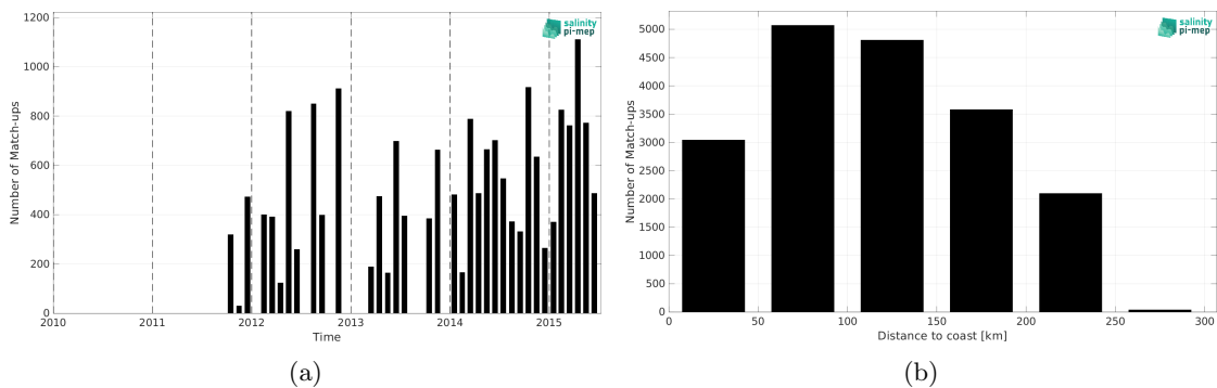
Figure 2: Number of match-ups between TSG (LEGOS-DM) and Aquarius SSS L3 OR v5 - Monthly - Rain mask (NASA-GSFC) SSS as a function of time (a) and as function of the distance to coast (b) over the Sea of Japan Pi-MEP region and for the full satellite product period.
