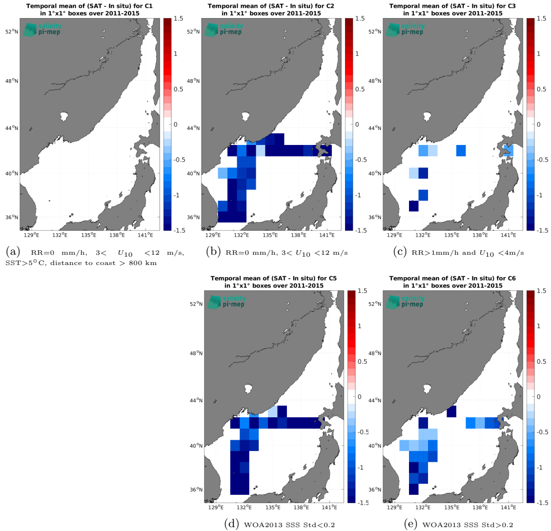
Figure 14: Temporal mean gridded over spatial boxes of size 1^\circ \times 1^\circ of \Delta\text{SSS} (Aquarius SSS L3 OR v5 - Monthly - Rain mask (NASA-GSFC) - TSG (LEGOS-DM)) for 5 different subdatasets corresponding to: RR=0 mm/h, 3 < U_{10} < 12 m/s, SST > 5^\circ\text{C} , distance to coast > 800 km (a), RR=0 mm/h, 3 < U_{10} < 12 m/s (b), RR > 1\text{mm/h} and U_{10} < 4\text{m/s} (c), WOA2013 SSS Std < 0.2 (d), WOA2013 SSS Std > 0.2 (e).
