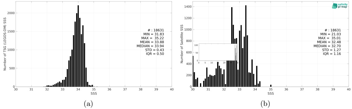
Figure 3: Histograms of SSS from TSG (LEGOS-DM) (a) and Aquarius SSS L3 OR v5 - Monthly - Rain mask (NASA-GSFC) (b) considering all match-up pairs per bins of 0.1 over the Sea of Japan Pi-MEP region and for the full satellite product period.
