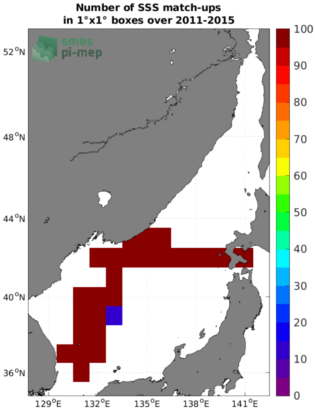
Figure 4: Number of SSS match-ups between TSG (LEGOS-DM) SSS and the Aquarius SSS L3 OR v5 - Monthly - Rain mask (NASA-GSFC) SSS product for the Sea of Japan Pi-MEP region over 1°×1° boxes and for the full satellite product period.
