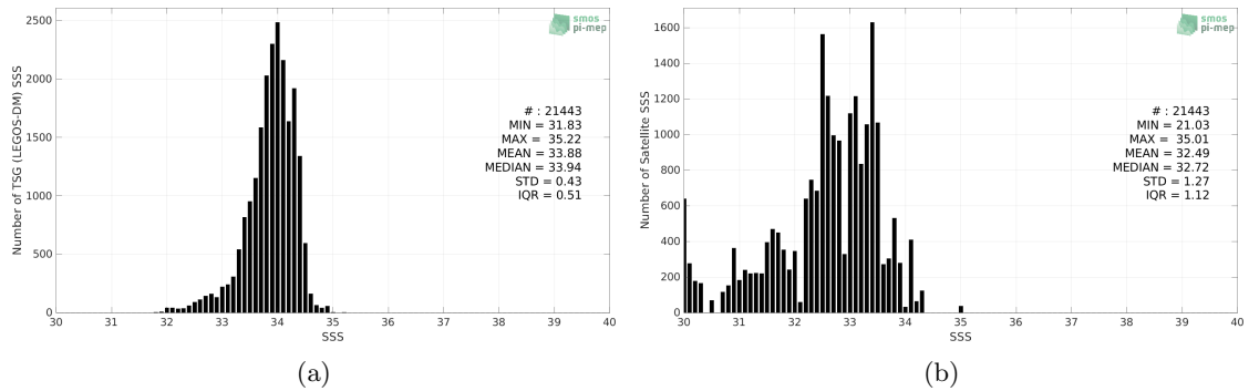
Figure 2: Histograms of SSS from TSG (LEGOS-DM) (a) and Aquarius SSS L3 OR v5 - Monthly - Rain mask (NASA-GSFC) (b) considering all match-up pairs per bins of 0.1 over the Sea of Japan Pi-MEP region and for the full satellite product period.
