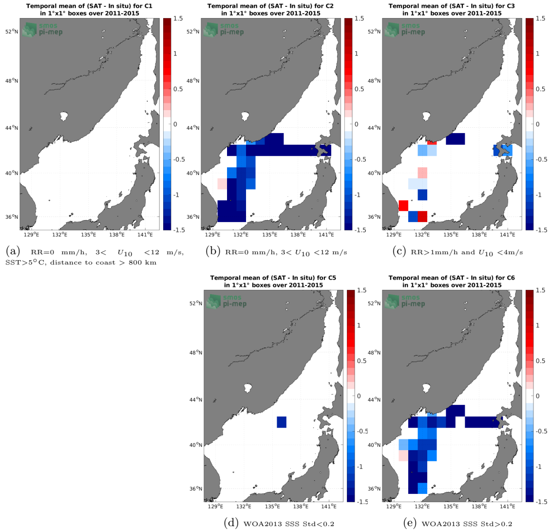
Figure 12: Temporal mean gridded over spatial boxes of size 1^\circ \times 1^\circ of \Delta\text{SSS} (Aquarius SSS L3 OR v5 - Monthly - Rain mask (NASA-GSFC) - TSG (LEGOS-DM)) for 5 different subdatasets corresponding to: RR=0 mm/h, 3 < U_{10} < 12 m/s, SST > 5^\circ\text{C} , distance to coast > 800 km (a), RR=0 mm/h, 3 < U_{10} < 12 m/s (b), RR > 1 mm/h and U_{10} < 4 m/s (c), WOA2013 SSS Std < 0.2 (d), WOA2013 SSS Std > 0.2 (e).
