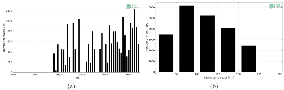
Figure 1: Number of match-ups between TSG (LEGOS-DM) and Aquarius SSS L3 OR v5 - Monthly - Rain mask (NASA-GSFC) SSS as a function of time (a) and as function of the distance to coast (b) over the Sea of Japan Pi-MEP region and for the full satellite product period.
