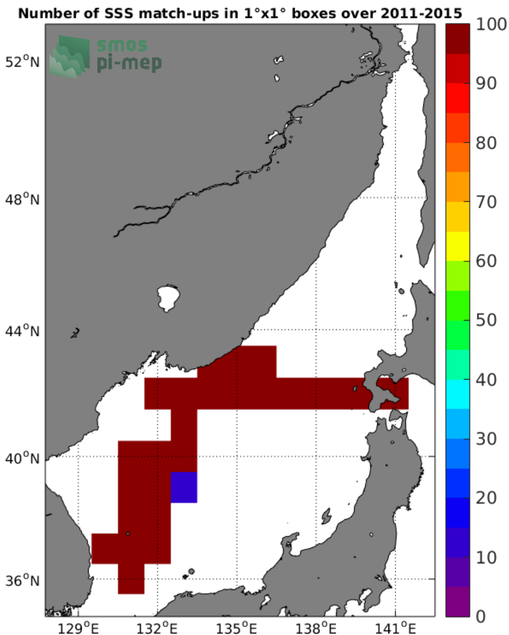
Figure 4: Number of SSS match-ups between TSG-LEGOS-DM SSS and the Aquarius-L3-OR-V5-MONTHLY-RAIN-MASK-1DEG SSS product for the Sea of Japan Pi-MEP region over 1°x1° boxes and for the full satellite product period.
