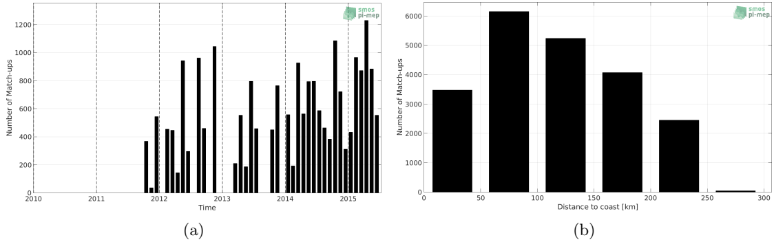
Figure 1: Number of match-ups between TSG-LEGOS-DM and Aquarius-L3-OR-V5-MONTHLY-RAIN-MASK-1DEG SSS as a function of time (a) and as function of the distance to coast (b) over the Sea of Japan Pi-MEP region and for the full satellite product period.
