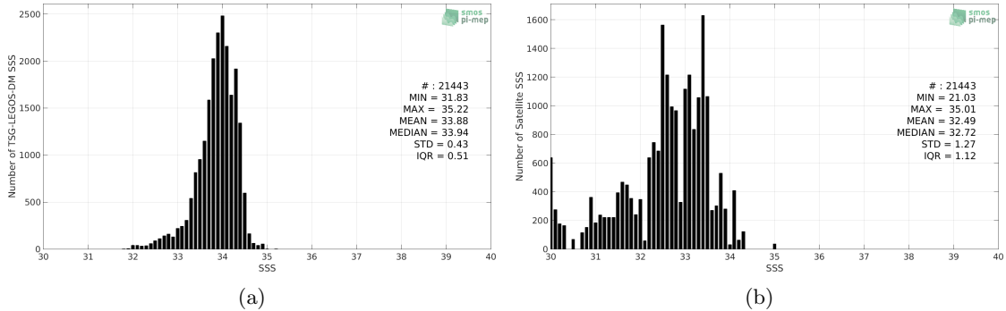
Figure 2: Histograms of SSS from TSG-LEGOS-DM (a) and Aquarius-L3-OR-V5-MONTHLY-RAIN-MASK-1DEG (b) considering all match-up pairs per bins of 0.1 over the Sea of Japan Pi-MEP region and for the full satellite product period.
