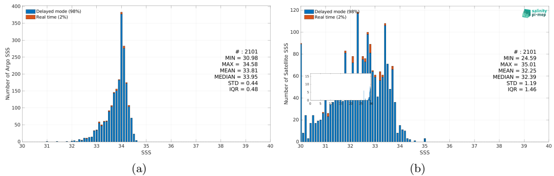
Figure 3: Histograms of SSS from Argo (a) and Aquarius SSS L3 OR v5 - Monthly - Rain mask (NASA-GSFC) (b) considering all match-up pairs per bins of 0.1 over the Sea of Japan Pi-MEP region and for the full satellite product period.
