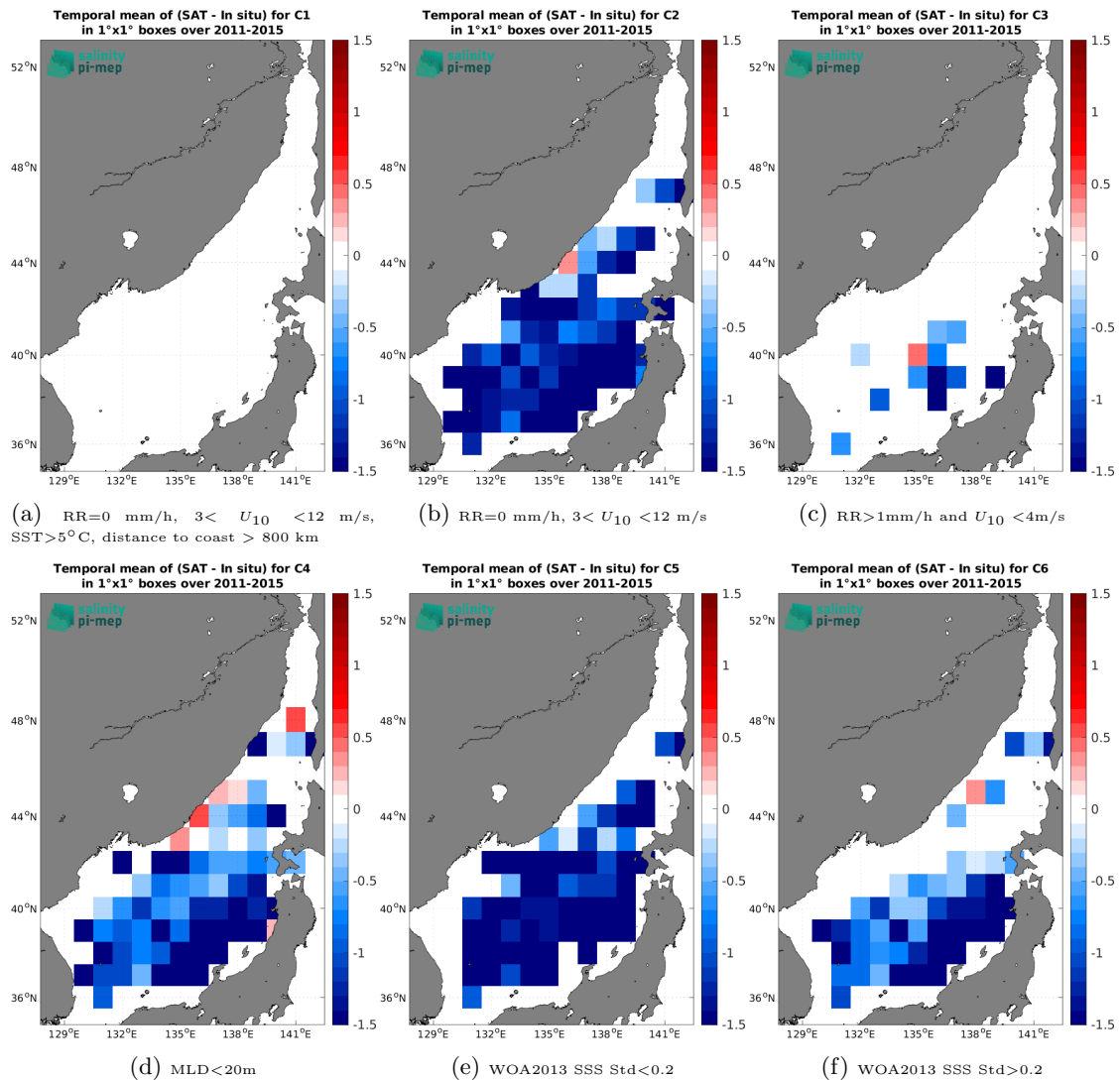
Figure 14: Temporal mean gridded over spatial boxes of size 1^\circ \times 1^\circ of \Delta\text{SSS} (Aquarius SSS L3 OR v5 - Monthly - Rain mask (NASA-GSFC) - Argo) for 6 different subdatasets corresponding to: RR=0 mm/h, 3 < U_{10} < 12 m/s, SST > 5^\circ\text{C} , distance to coast > 800 km (a), RR=0 mm/h, 3 < U_{10} < 12 m/s (b), RR > 1 mm/h and U_{10} < 4 m/s (c), MLD < 20 m (d), WOA2013 SSS Std < 0.2 (e), WOA2013 SSS Std > 0.2 (f).
