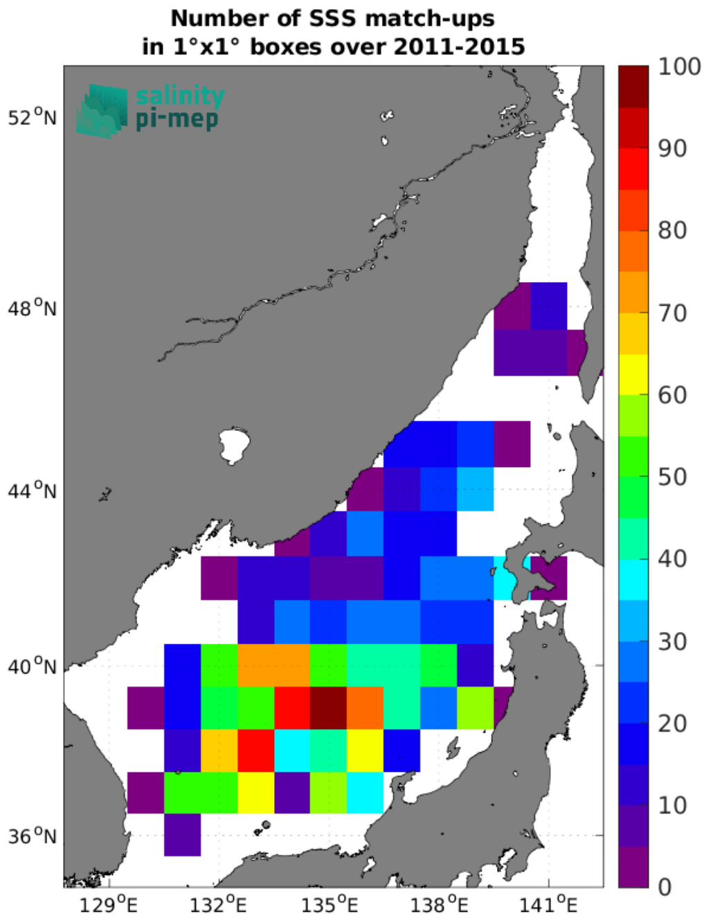
Figure 5: Number of SSS match-ups between Argo SSS and the Aquarius SSS L3 OR v5 - Monthly - Rain mask (NASA-GSFC) SSS product for the Sea of Japan Pi-MEP region over 1°x1° boxes and for the full satellite product period.
