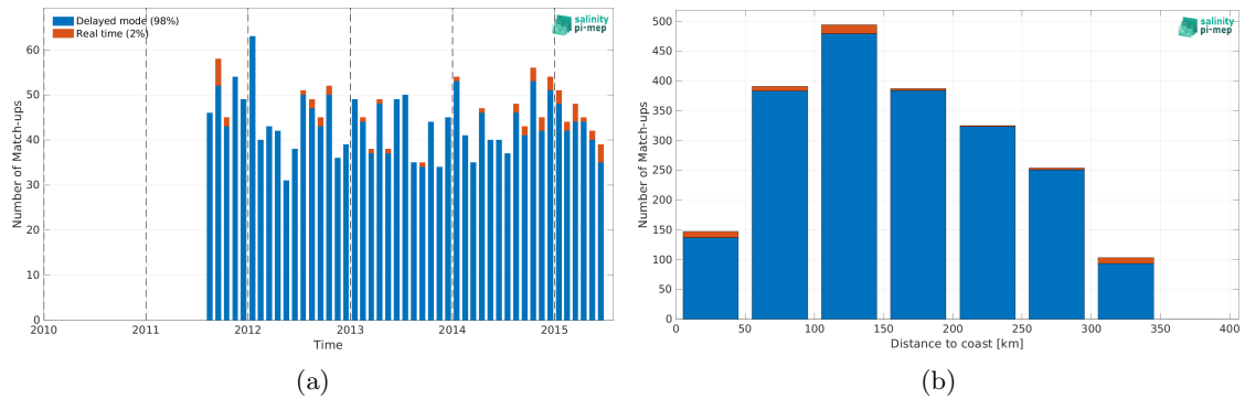
Figure 2: Number of match-ups between Argo and Aquarius SSS L3 OR v5 - Monthly - Rain mask (NASA-GSFC) SSS as a function of time (a) and as function of the distance to coast (b) over the Sea of Japan Pi-MEP region and for the full satellite product period.
