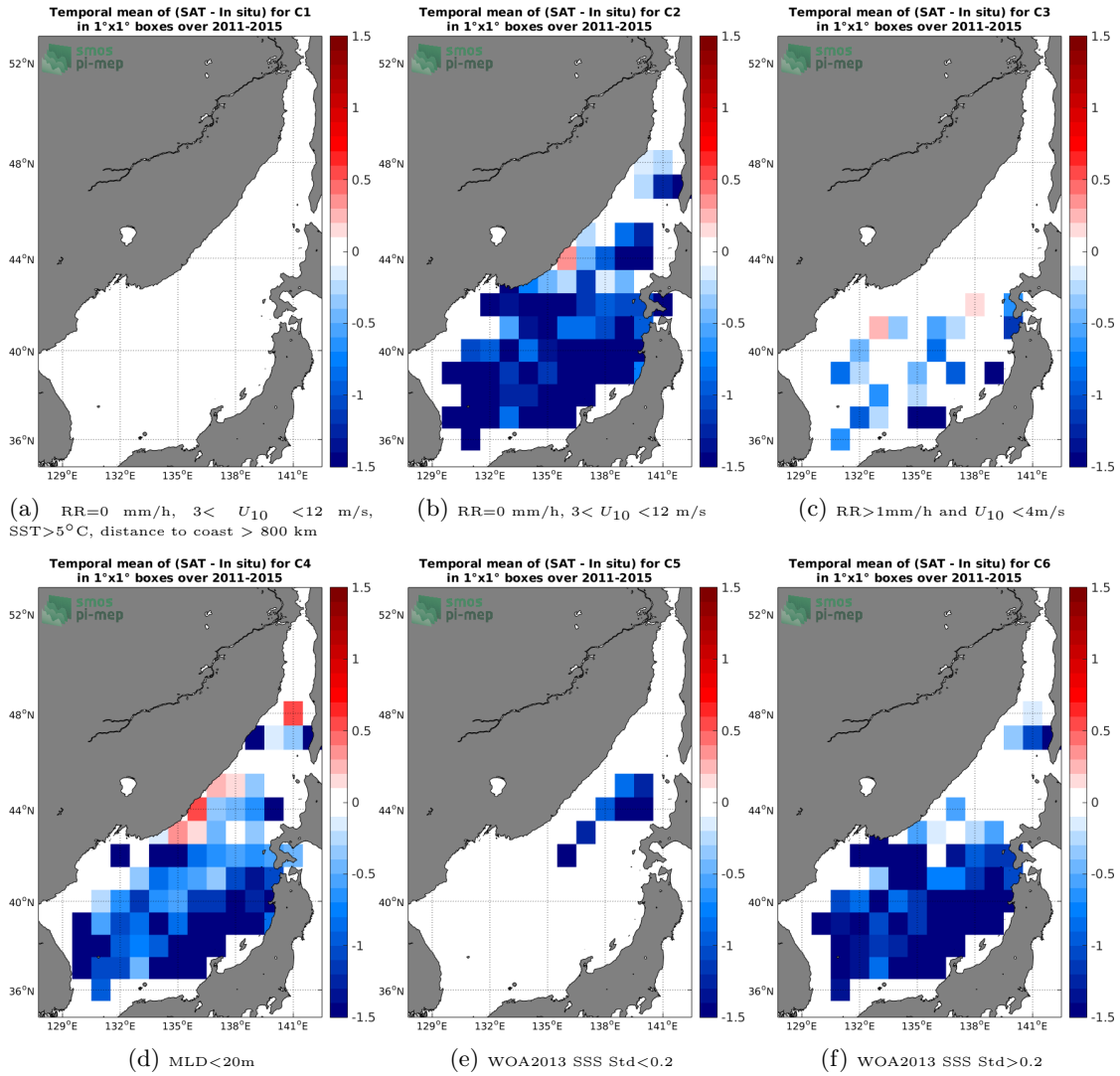
Figure 12: Temporal mean gridded over spatial boxes of size 1°x1° of \Delta SSS (Aquarius-L3-OR-V5-MONTHLY-RAIN-MASK-1DEG - Argo) for 6 different subdatasets corresponding to: RR=0 mm/h, 3 < U_{10} < 12 m/s, SST > 5°C, distance to coast > 800 km (a), RR=0 mm/h, 3 < U_{10} < 12 m/s (b), RR > 1mm/h and U_{10} < 4 m/s (c), MLD < 20m (d), WOA2013 SSS Std < 0.2 (e), WOA2013 SSS Std > 0.2 (f).
