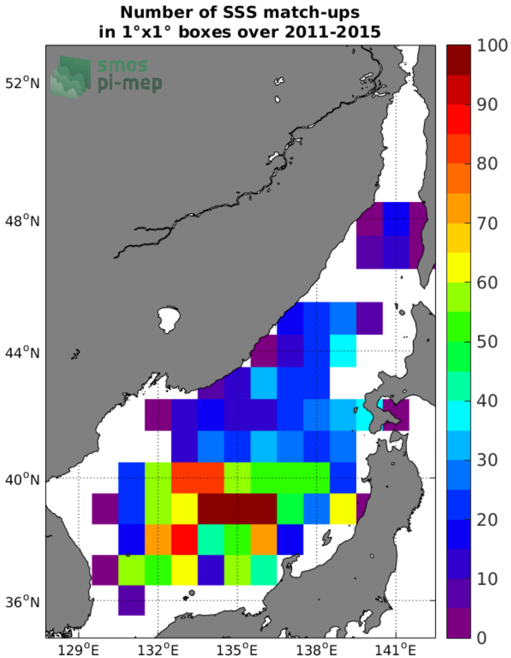
Figure 4: Number of SSS match-ups between Argo SSS and the Aquarius-L3-OR-V5-MONTHLY-RAIN-MASK-1DEG SSS product for the Sea of Japan Pi-MEP region over 1°x1° boxes and for the full satellite product period.
