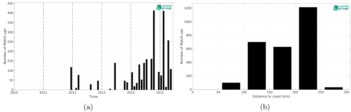
Figure 2: Number of match-ups between TSG (LEGOS-DM) and Aquarius SSS L3 CAP v5 - 7-Day running (JPL) SSS as a function of time (a) and as function of the distance to coast (b) over the Sea of Japan Pi-MEP region and for the full satellite product period.
