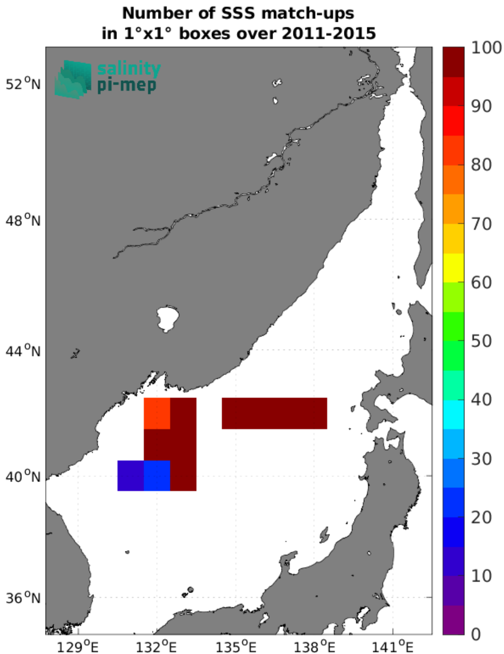
Figure 5: Number of SSS match-ups between TSG (LEGOS-DM) SSS and the Aquarius SSS L3 CAP v5 - 7-Day running (JPL) SSS product for the Sea of Japan Pi-MEP region over 1°x1° boxes and for the full satellite product period.
