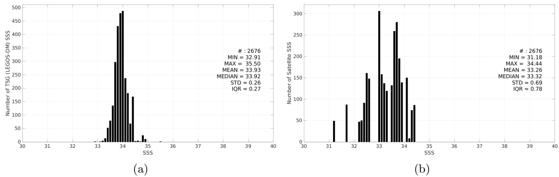
Figure 3: Histograms of SSS from TSG (LEGOS-DM) (a) and Aquarius SSS L3 CAP v5 - 7-Day running (JPL) (b) considering all match-up pairs per bins of 0.1 over the Sea of Japan Pi-MEP region and for the full satellite product period.
