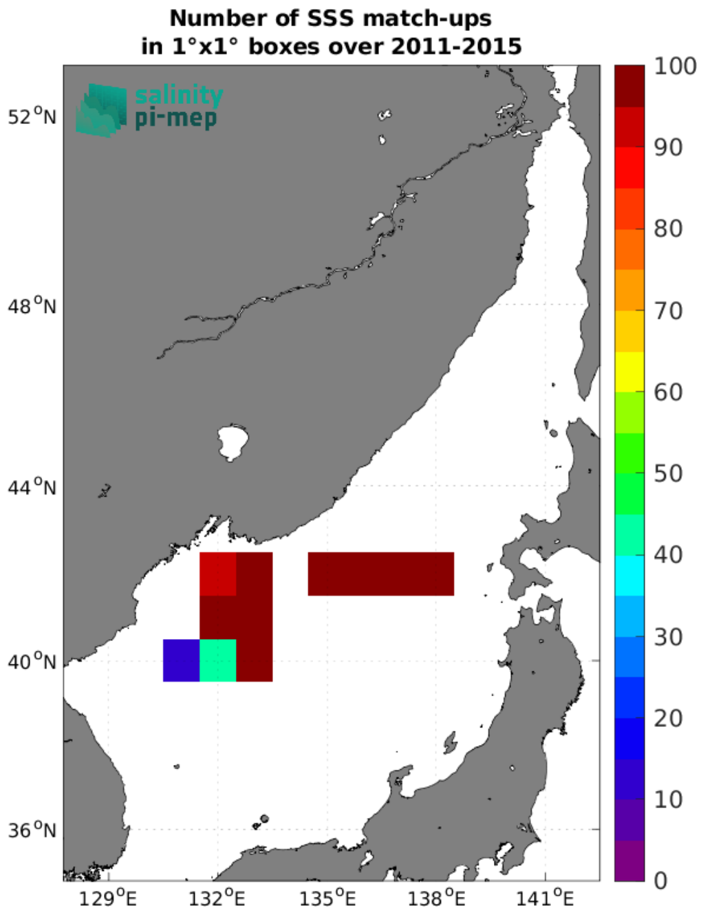
Figure 4: Number of SSS match-ups between TSG (LEGOS-DM) SSS and the Aquarius SSS L3 CAP v5 - 7-Day running (JPL) SSS product for the Sea of Japan Pi-MEP region over 1°x1° boxes and for the full satellite product period.
