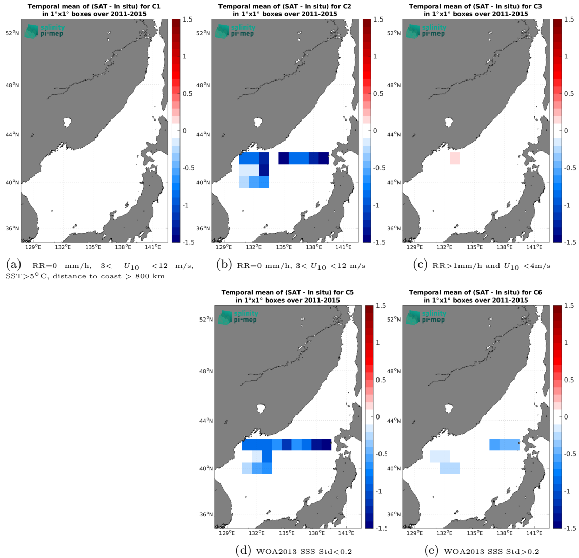
Figure 12: Temporal mean gridded over spatial boxes of size 1^\circ \times 1^\circ of \Delta\text{SSS} (Aquarius SSS L3 CAP v5 - 7-Day running (JPL) - TSG (LEGOS-DM)) for 5 different subdatasets corresponding to: RR=0 mm/h, 3 < U_{10} < 12 m/s, SST > 5^\circ\text{C} , distance to coast > 800 km (a), RR=0 mm/h, 3 < U_{10} < 12 m/s (b), RR > 1 mm/h and U_{10} < 4 m/s (c), WOA2013 SSS Std < 0.2 (d), WOA2013 SSS Std > 0.2 (e).
