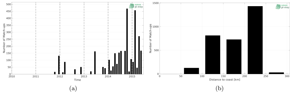
Figure 1: Number of match-ups between TSG (LEGOS-DM) and Aquarius SSS L3 CAP v5 - 7-Day running (JPL) SSS as a function of time (a) and as function of the distance to coast (b) over the Sea of Japan Pi-MEP region and for the full satellite product period.
