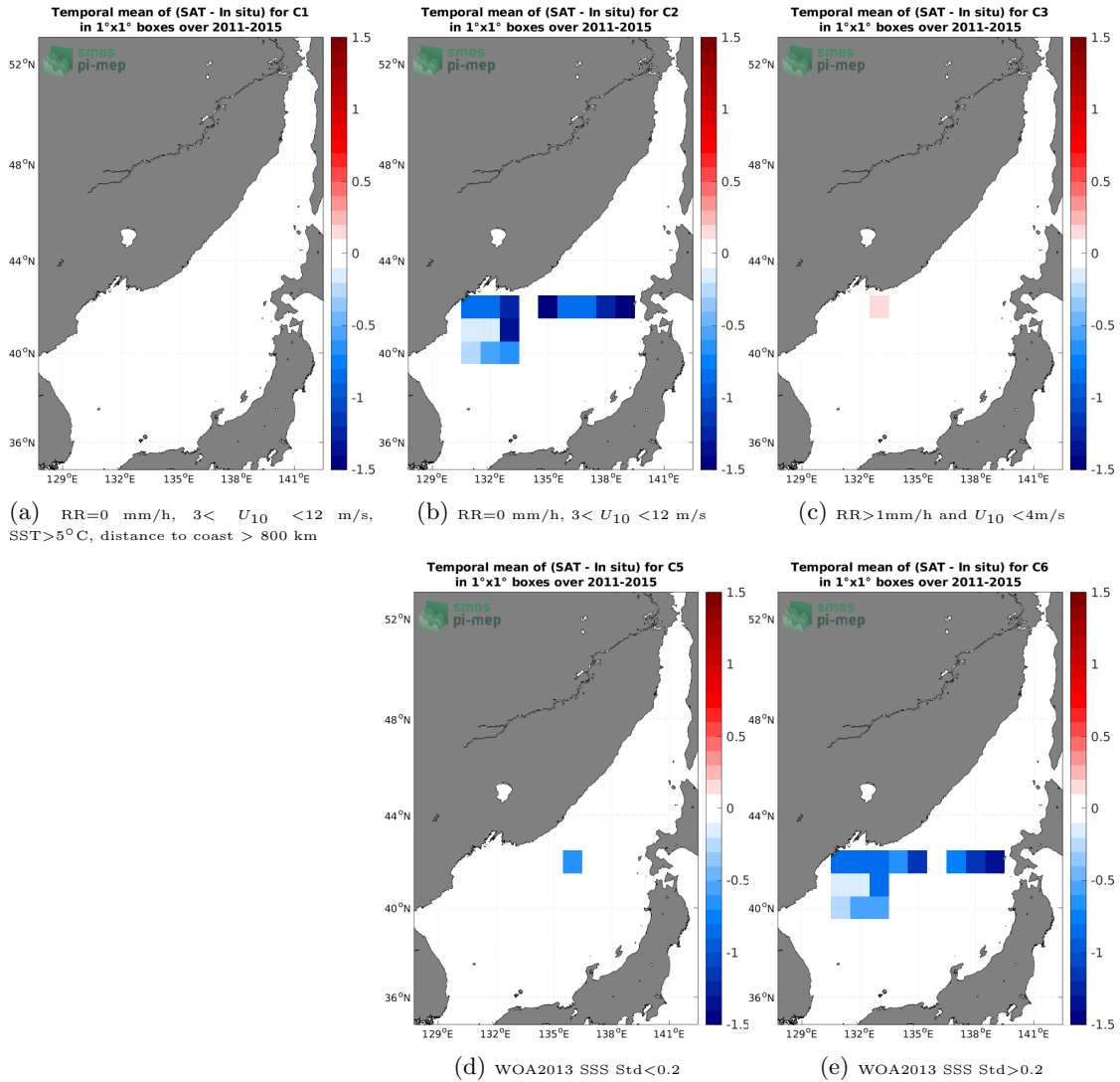
Figure 12: Temporal mean gridded over spatial boxes of size 1°×1° of \Delta SSS (Aquarius SSS L3 CAP v5 - 7-Day running (JPL) - TSG (LEGOS-DM)) for 5 different subdatasets corresponding to:RR=0 mm/h, 3 < U_{10} < 12 m/s, SST>5°C, distance to coast > 800 km (a), RR=0 mm/h, 3 < U_{10} < 12 m/s (b), RR>1mm/h and U_{10} < 4 m/s (c), WOA2013 SSS Std<0.2 (d), WOA2013 SSS Std>0.2 (e).
