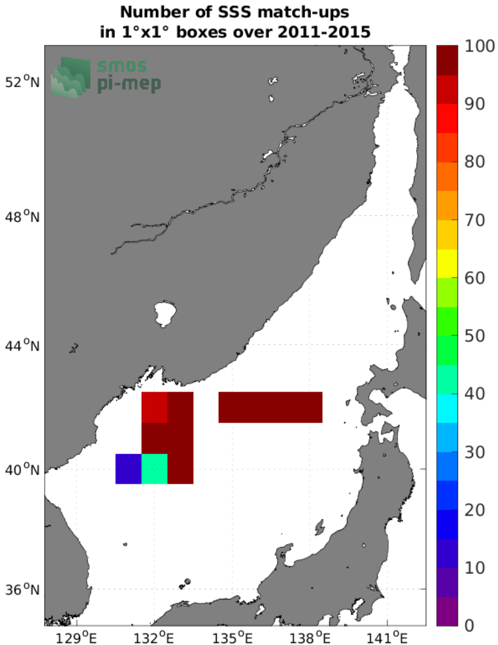
Figure 4: Number of SSS match-ups between TSG (LEGOS-DM) SSS and the Aquarius SSS L3 CAP v5 - 7-Day running (JPL) SSS product for the Sea of Japan Pi-MEP region over 1°×1° boxes and for the full satellite product period.
