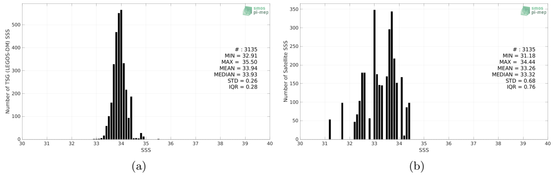
Figure 2: Histograms of SSS from TSG (LEGOS-DM) (a) and Aquarius SSS L3 CAP v5 - 7-Day running (JPL) (b) considering all match-up pairs per bins of 0.1 over the Sea of Japan Pi-MEP region and for the full satellite product period.
