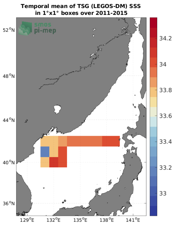
(c) MEAN(TSG (LEGOS-DM) SSS)
