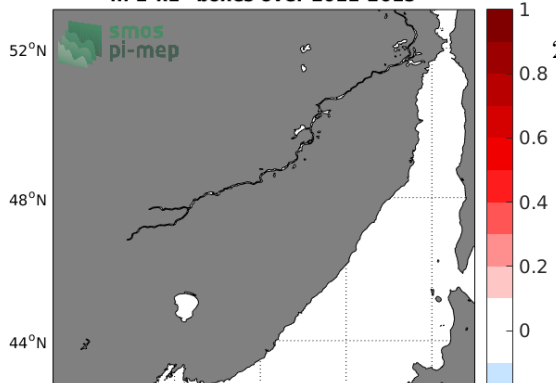
Temporal mean of (Sat - TSG-LEGOS-DM) in 1°x1° boxes over 2011-2015
