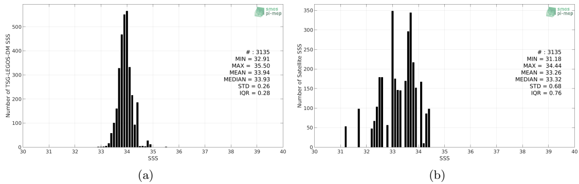
Figure 2: Histograms of SSS from TSG-LEGOS-DM (a) and Aquarius-L3-JPL-V5-7DAY-RUNNING (b) considering all match-up pairs per bins of 0.1 over the Sea of Japan Pi-MEP region and for the full satellite product period.
