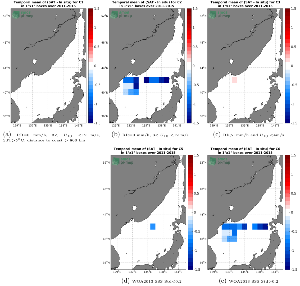
Figure 12: Temporal mean gridded over spatial boxes of size 1^\circ \times 1^\circ of \Delta SSS (Aquarius-L3-JPL-V5-7DAY-RUNNING - TSG-LEGOS-DM) for 5 different subdatasets corresponding to:RR=0 mm/h, 3 < U_{10} < 12 m/s, SST>5°C, distance to coast > 800 km (a), RR=0 mm/h, 3 < U_{10} < 12 m/s (b), RR>1mm/h and U_{10} < 4 m/s (c), WOA2013 SSS Std<0.2 (d), WOA2013 SSS Std>0.2 (e).
