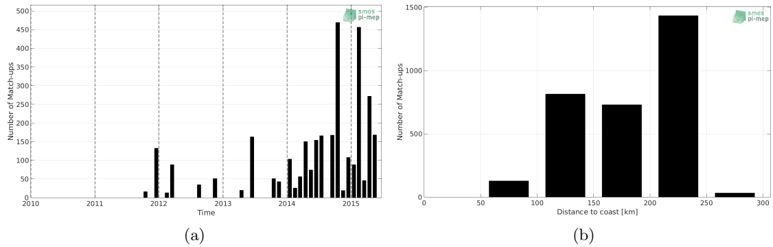
Figure 1: Number of match-ups between TSG-LEGOS-DM and Aquarius-L3-JPL-V5-7DAY-RUNNING SSS as a function of time (a) and as function of the distance to coast (b) over the Sea of Japan Pi-MEP region and for the full satellite product period.
