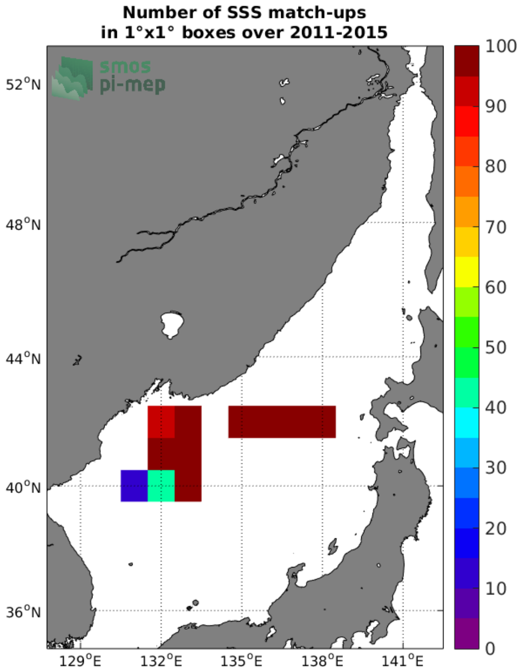
Figure 4: Number of SSS match-ups between TSG-LEGOS-DM SSS and the Aquarius-L3-JPL-V5-7DAY-RUNNING SSS product for the Sea of Japan Pi-MEP region over 1°x1° boxes and for the full satellite product period.
