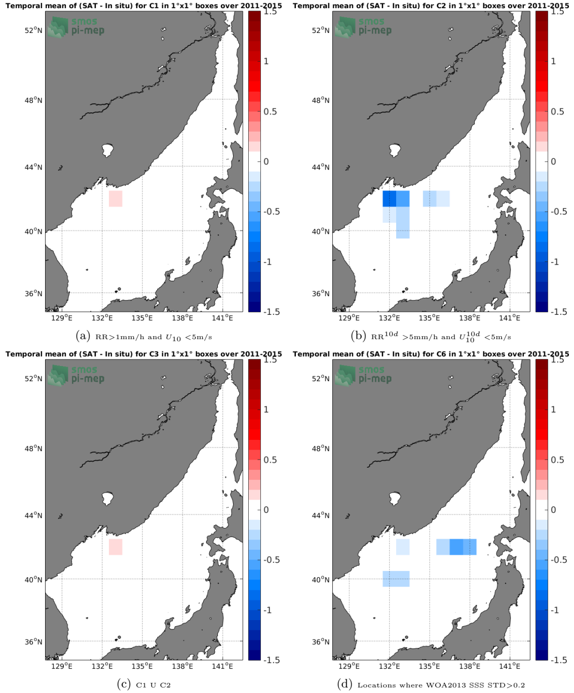
Figure 12: Temporal mean gridded over spatial boxes of size 1°x1° of \Delta\text{SSS} (Aquarius-L3-JPL-V5-7DAY-RUNNING - TSG-LEGOS-DM) for 4 different subdatasets corresponding to: RR > 1\text{mm/h} and U_{10} < 5\text{m/s} (a), RR^{10d} > 5\text{mm/h} and U_{10}^{10d} < 5\text{m/s} (b), C1 U C2 (c), Locations where WOA2013 SSS STD > 0.2 (d).
