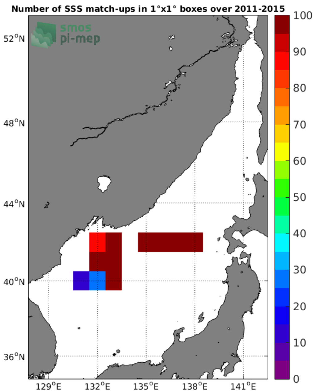
Figure 4: Number of SSS match-ups between TSG-LEGOS-DM SSS and the Aquarius-L3-JPL-V5-7DAY-RUNNING SSS product for the Sea of Japan Pi-MEP region over 1°x1° boxes and for the full satellite product period.
