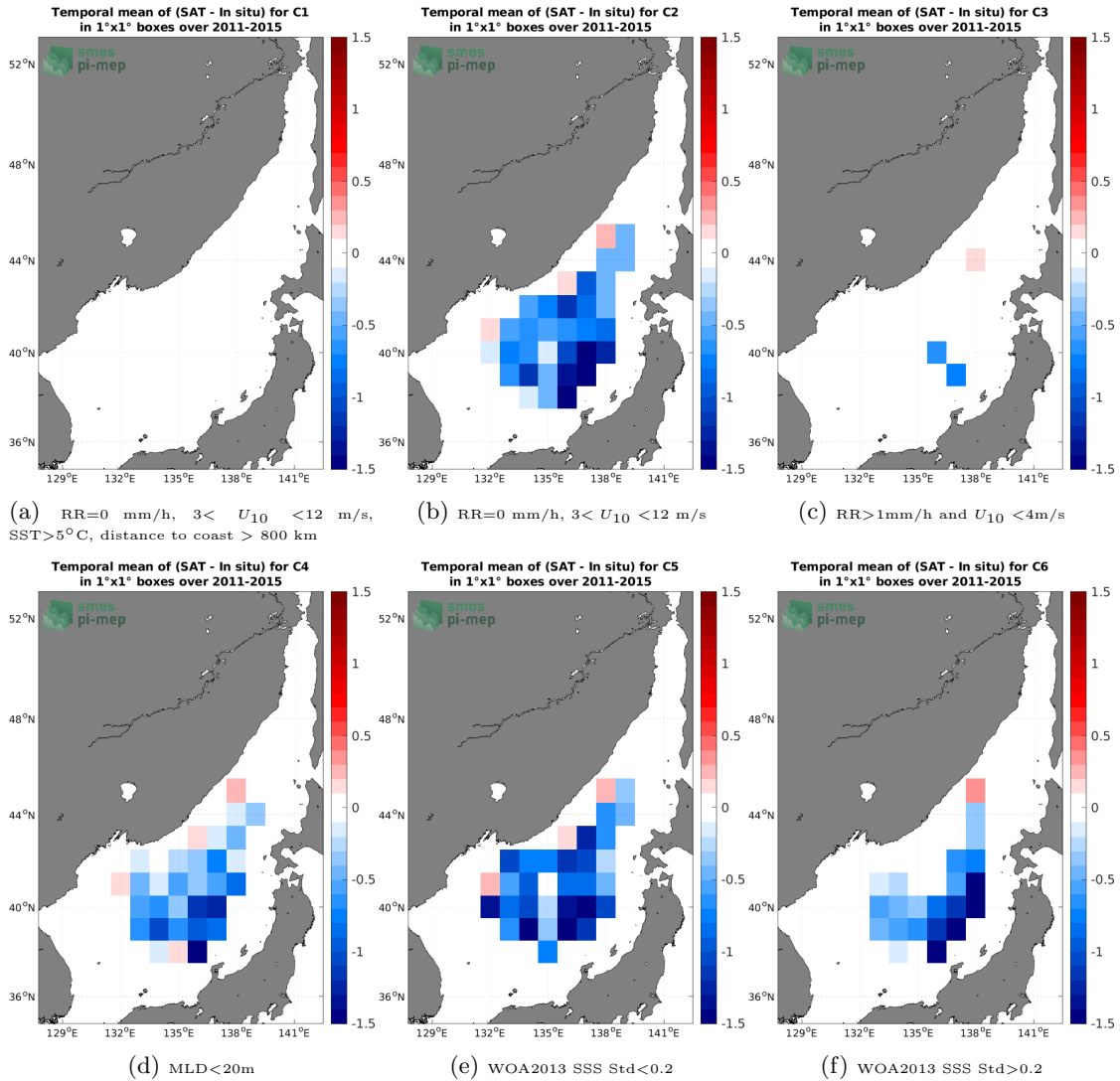
Figure 12: Temporal mean gridded over spatial boxes of size 1^\circ \times 1^\circ of \Delta SSS (Aquarius SSS L3 CAP v5 - 7-Day running (JPL) - Argo) for 6 different subdatasets corresponding to: RR=0 mm/h, 3 < U_{10} < 12 m/s, SST > 5°C, distance to coast > 800 km (a), RR=0 mm/h, 3 < U_{10} < 12 m/s (b), RR > 1mm/h and U_{10} < 4 m/s (c),MLD < 20m (d),WOA2013 SSS Std < 0.2 (e),WOA2013 SSS Std > 0.2 (f).
