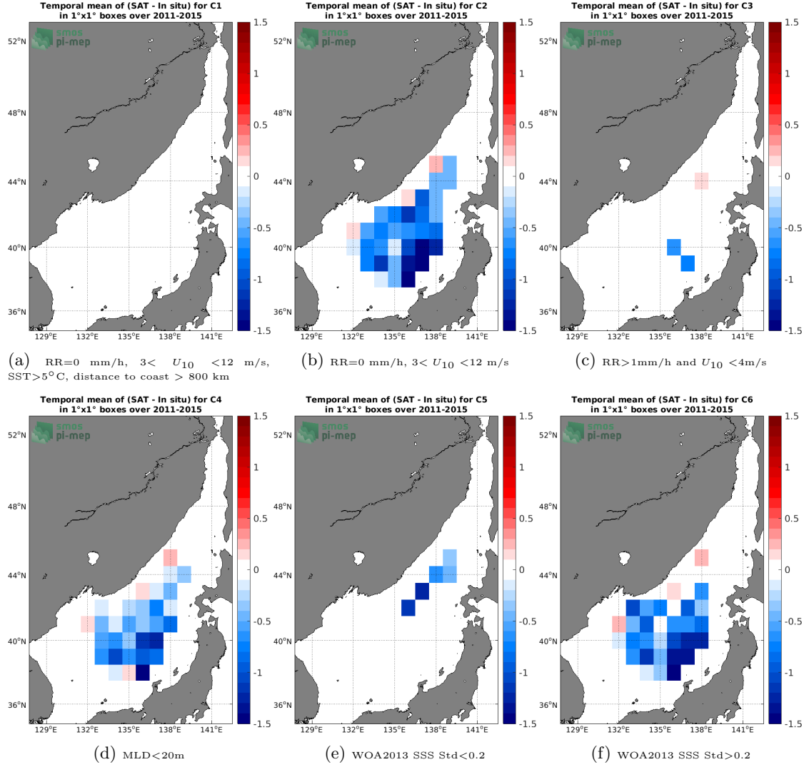
Figure 12: Temporal mean gridded over spatial boxes of size 1^\circ \times 1^\circ of \Delta\text{SSS} (Aquarius SSS L3 CAP v5 - 7-Day running (JPL) - Argo) for 6 different subdatasets corresponding to: RR=0 mm/h, 3 < U_{10} < 12 m/s, SST > 5^\circ\text{C} , distance to coast > 800 km (a), RR=0 mm/h, 3 < U_{10} < 12 m/s (b), RR > 1\text{mm/h} and U_{10} < 4\text{m/s} (c), MLD < 20\text{m} (d), WOA2013 SSS Std < 0.2 (e), WOA2013 SSS Std > 0.2 (f).
