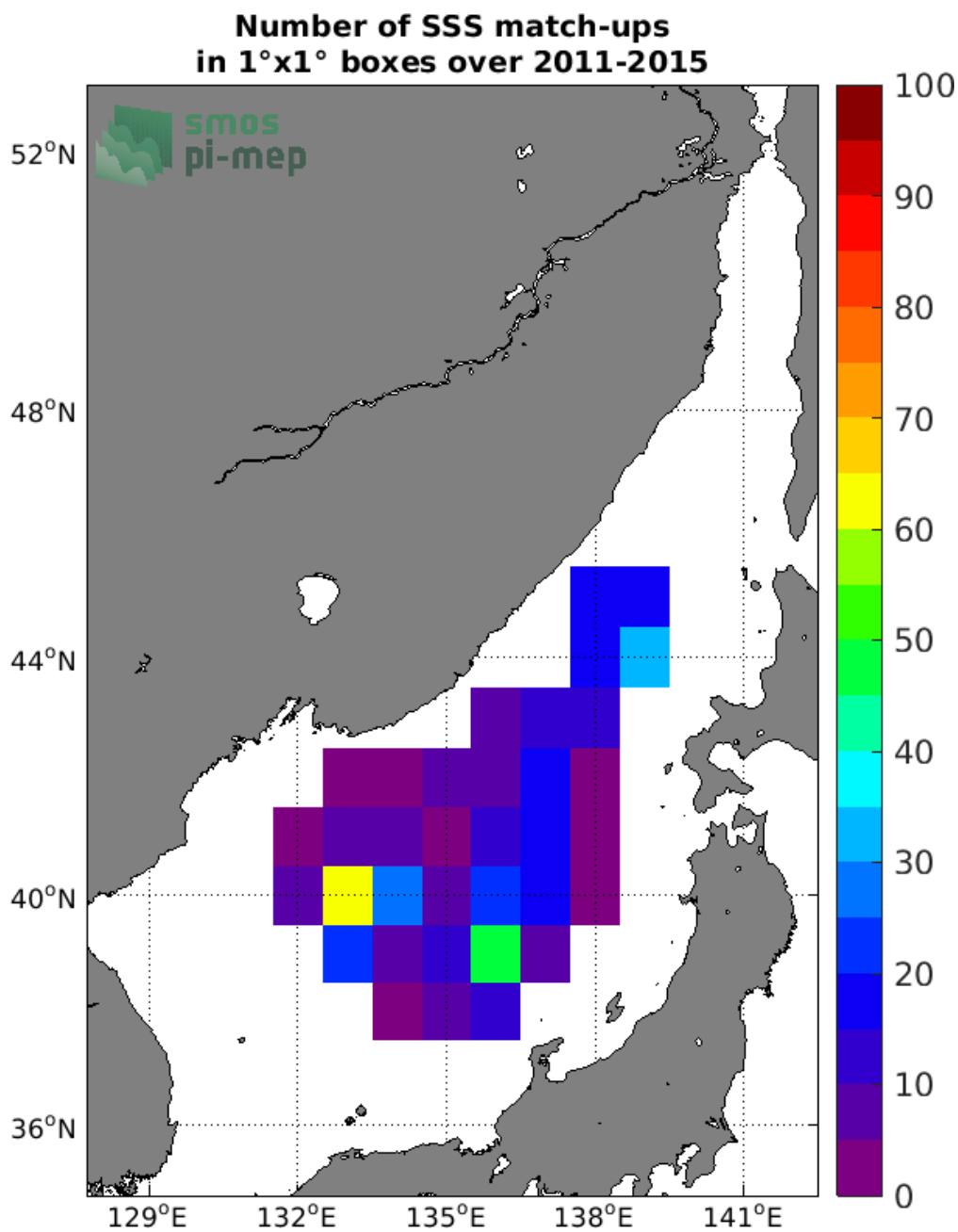
Figure 4: Number of SSS match-ups between Argo SSS and the Aquarius SSS L3 CAP v5 - 7-Day running (JPL) SSS product for the Sea of Japan Pi-MEP region over 1°x1° boxes and for the full satellite product period.
