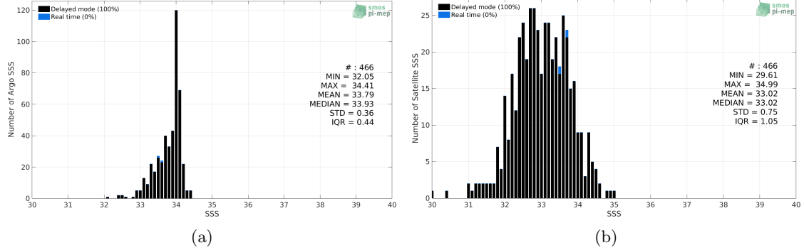
Figure 2: Histograms of SSS from Argo (a) and Aquarius SSS L3 CAP v5 - 7-Day running (JPL) (b) considering all match-up pairs per bins of 0.1 over the Sea of Japan Pi-MEP region and for the full satellite product period.
