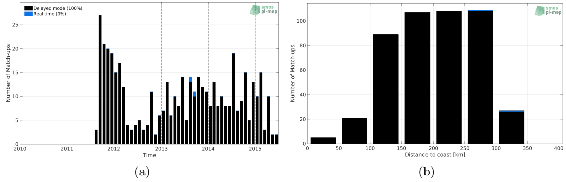
Figure 1: Number of match-ups between Argo and Aquarius SSS L3 CAP v5 - 7-Day running (JPL) SSS as a function of time (a) and as function of the distance to coast (b) over the Sea of Japan Pi-MEP region and for the full satellite product period.
